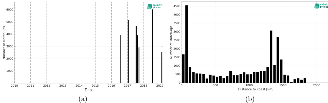
Figure 2: Number of match-ups between TSG (GOSUD-Research-vessel) and SMAP SSS L3 v5.3 - 8-Day running (RSS) SSS as a function of time (a) and as function of the distance to coast (b) over the Gulf Stream Pi-MEP region and for the full satellite product period.
