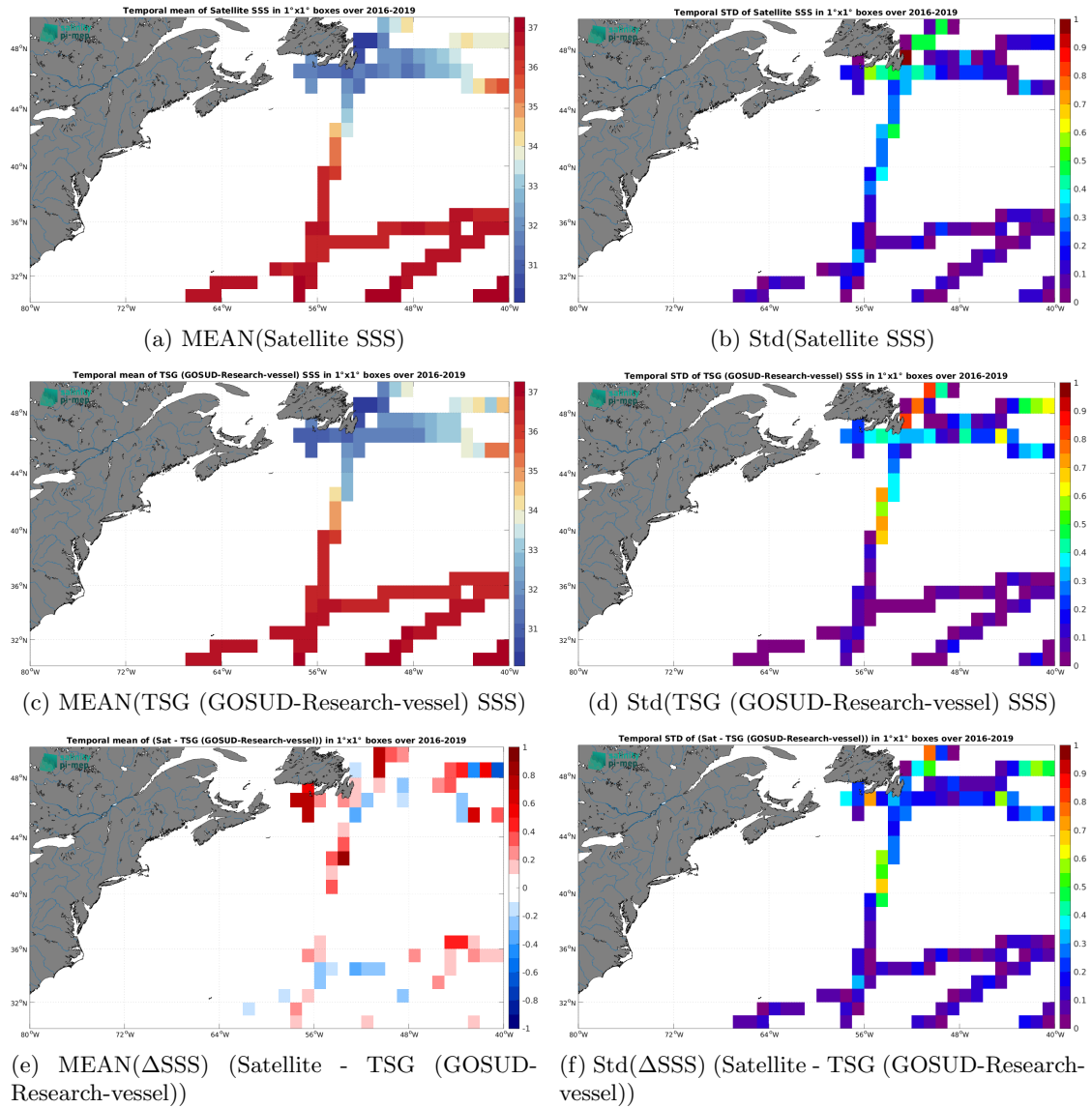
Figure 7: Temporal mean (left) and Std (right) of SSS from SMAP SSS L3 v5.3 - 8-Day running (RSS) (top), TSG (GOSUD-Research-vessel) (middle), and of \Delta SSS (Satellite - TSG (GOSUD-Research-vessel)). Only match-up pairs are used to generate these maps.
