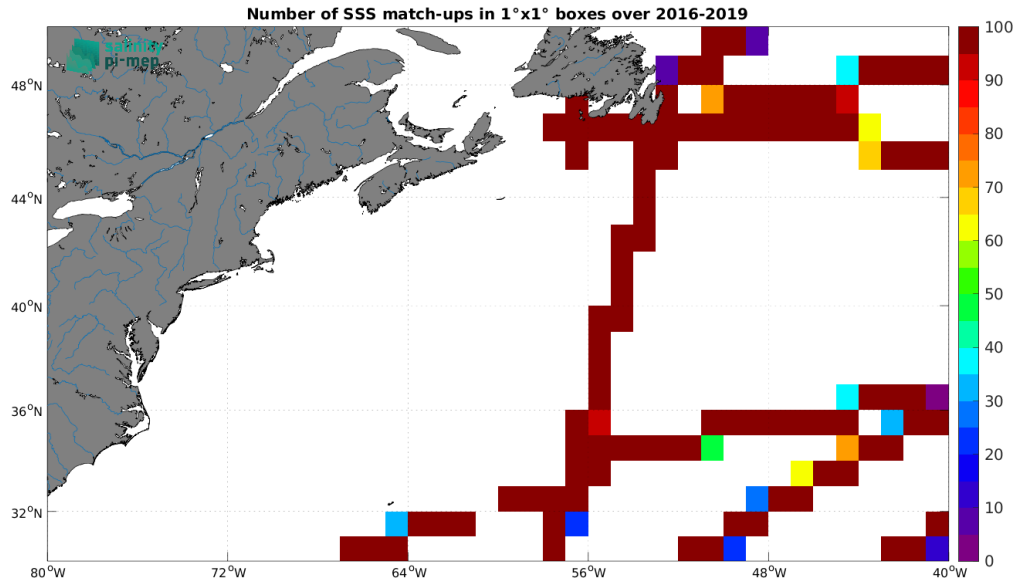
Figure 5: Number of SSS match-ups between TSG (GOSUD-Research-vessel) SSS and the SMAP SSS L3 v5.3 - 8-Day running (RSS) SSS product for the Gulf Stream Pi-MEP region over 1^\circ \times 1^\circ boxes and for the full satellite product period.
