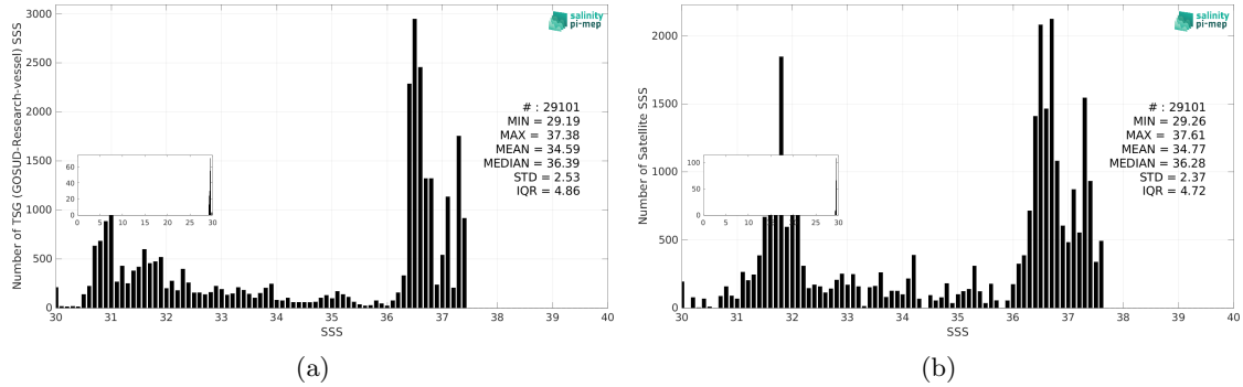
Figure 3: Histograms of SSS from TSG (GOSUD-Research-vessel) (a) and SMAP SSS L3 v5.3 - 8-Day running (RSS) (b) considering all match-up pairs per bins of 0.1 over the Gulf Stream Pi-MEP region and for the full satellite product period.
