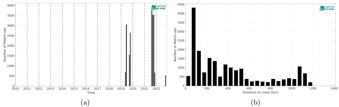
Figure 2: Number of match-ups between Sairdrone and SMAP SSS L3 v5.3 - 8-Day running (RSS) SSS as a function of time (a) and as function of the distance to coast (b) over the Gulf Stream Pi-MEP region and for the full satellite product period.
