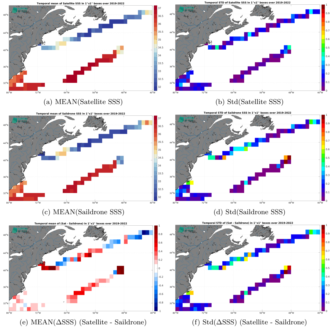
Figure 7: Temporal mean (left) and Std (right) of SSS from SMAP SSS L3 v5.3 - 8-Day running (RSS) (top), Saildrone (middle), and of \Delta SSS (Satellite - Saildrone). Only match-up pairs are used to generate these maps.
