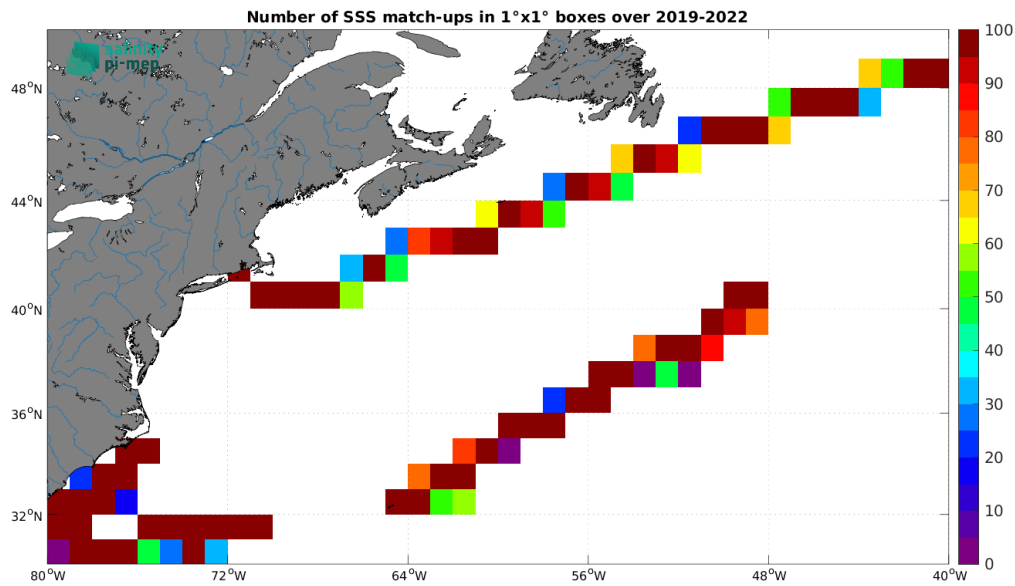
Figure 5: Number of SSS match-ups between Sairdrone SSS and the SMAP SSS L3 v5.3 - 8-Day running (RSS) SSS product for the Gulf Stream Pi-MEP region over 1^\circ \times 1^\circ boxes and for the full satellite product period.
