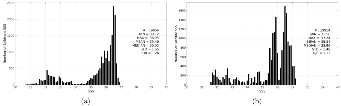
Figure 3: Histograms of SSS from Saildrone (a) and SMAP SSS L3 v5.3 - 8-Day running (RSS) (b) considering all match-up pairs per bins of 0.1 over the Gulf Stream Pi-MEP region and for the full satellite product period.
