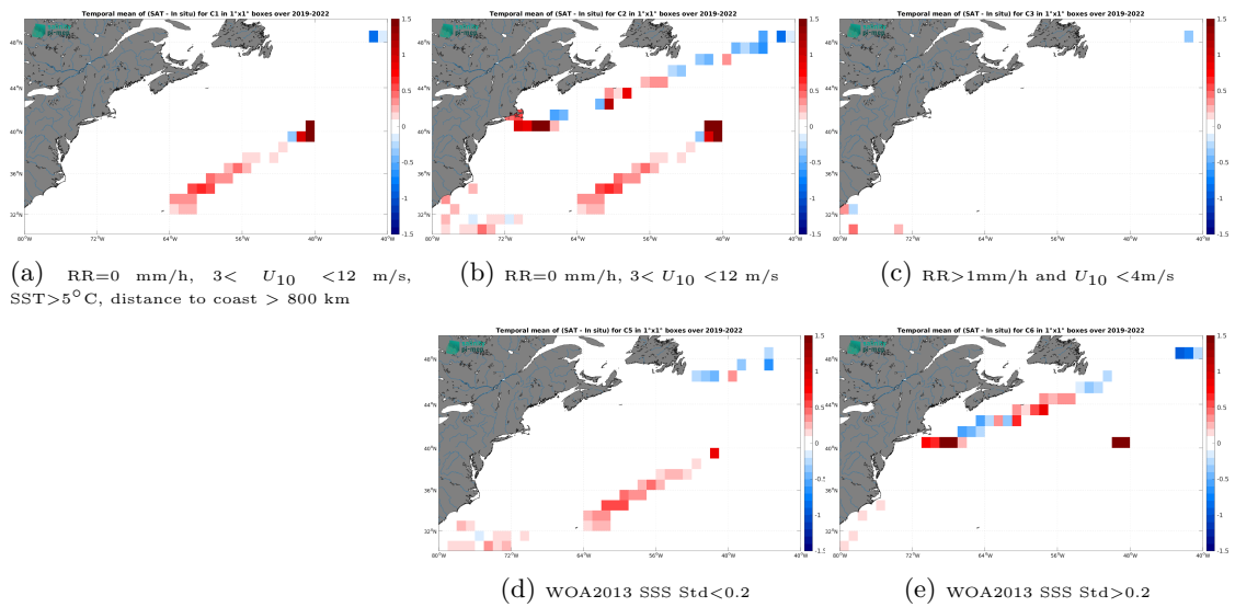
Figure 14: Temporal mean gridded over spatial boxes of size 1^\circ \times 1^\circ of \Delta SSS (SMAP SSS L3 v5.3 - 8-Day running (RSS) - Sairdrone) for 5 different subdatasets corresponding to:RR=0 mm/h, 3 < U_{10} < 12 m/s, SST>5°C, distance to coast > 800 km (a), RR=0 mm/h, 3 < U_{10} < 12 m/s (b), RR>1mm/h and U_{10} < 4 m/s (c), WOA2013 SSS Std<0.2 (d), WOA2013 SSS Std>0.2 (e).
