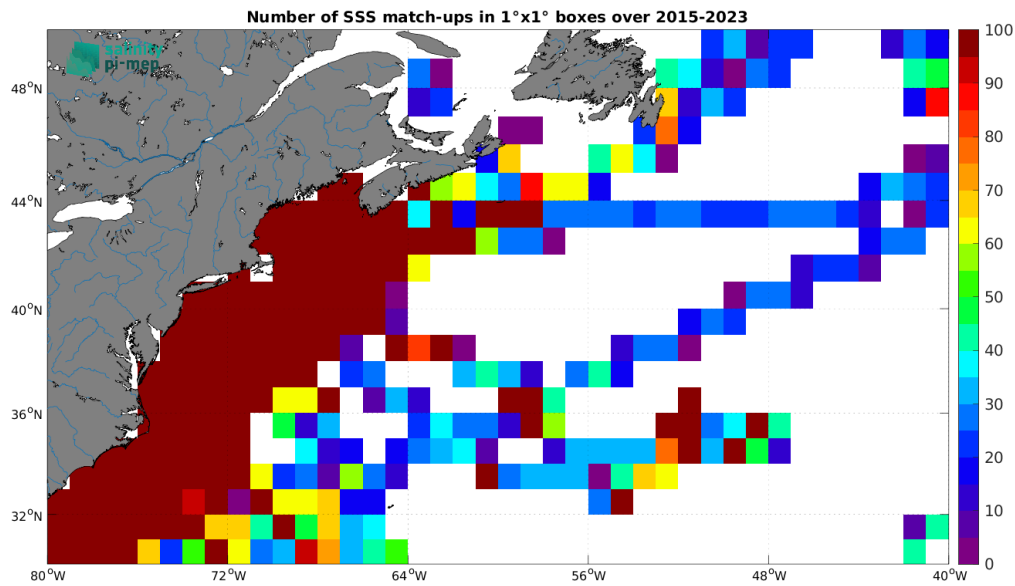
Figure 5: Number of SSS match-ups between TSG (SAMOS) SSS and the SMAP SSS L3 v5.3 - Monthly (RSS) SSS product for the Gulf Stream Pi-MEP region over 1^\circ \times 1^\circ boxes and for the full satellite product period.
