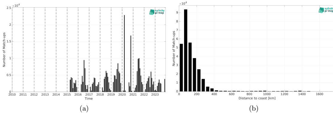
Figure 2: Number of match-ups between TSG (SAMOS) and SMAP SSS L3 v5.3 - Monthly (RSS) SSS as a function of time (a) and as function of the distance to coast (b) over the Gulf Stream Pi-MEP region and for the full satellite product period.
