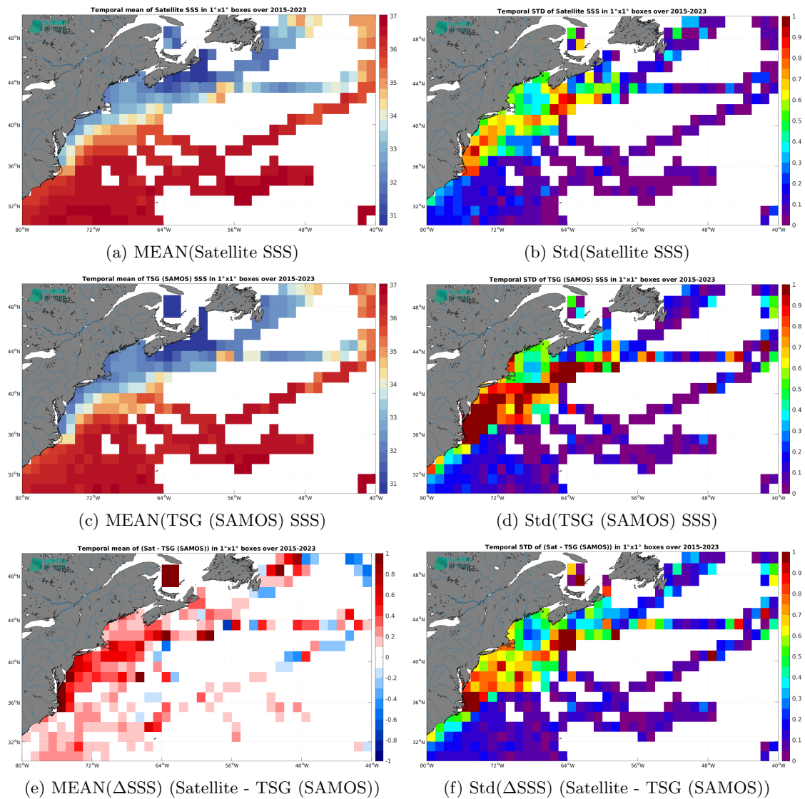
Figure 7: Temporal mean (left) and Std (right) of SSS from SMAP SSS L3 v5.3 - Monthly (RSS) (top), TSG (SAMOS) (middle), and of \Delta SSS (Satellite - TSG (SAMOS)). Only match-up pairs are used to generate these maps.
