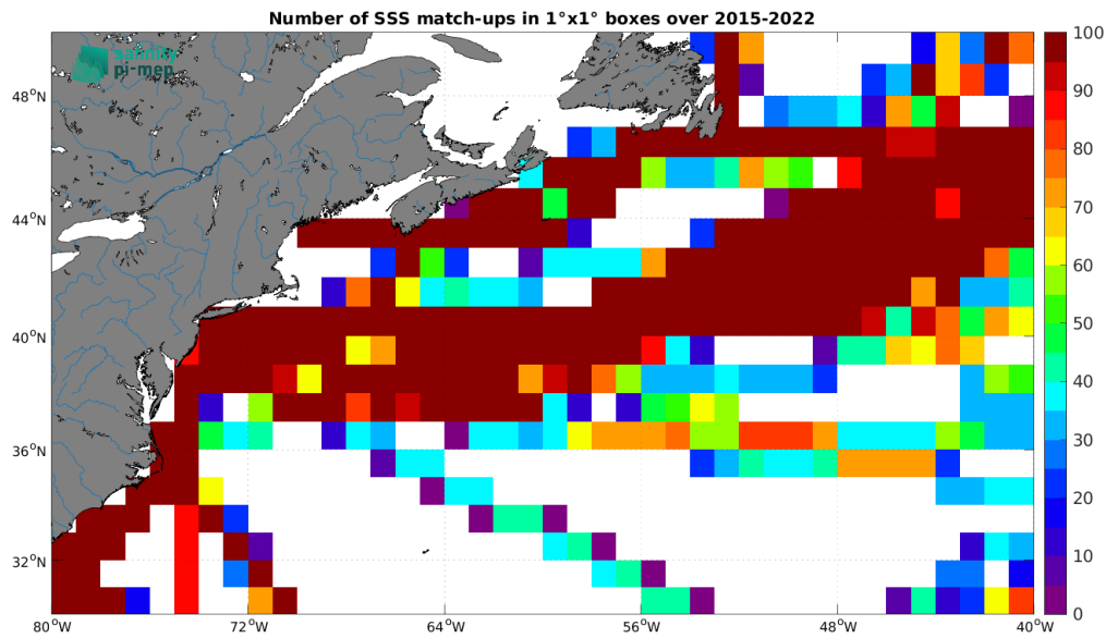
Figure 5: Number of SSS match-ups between TSG (LEGOS-DM) SSS and the SMAP SSS L3 v5.3 - Monthly (RSS) SSS product for the Gulf Stream Pi-MEP region over 1^\circ \times 1^\circ boxes and for the full satellite product period.
