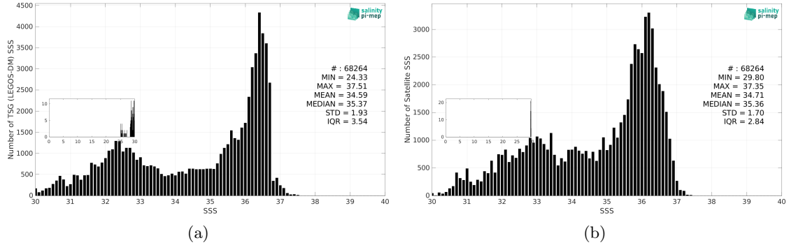
Figure 3: Histograms of SSS from TSG (LEGOS-DM) (a) and SMAP SSS L3 v5.3 - Monthly (RSS) (b) considering all match-up pairs per bins of 0.1 over the Gulf Stream Pi-MEP region and for the full satellite product period.
