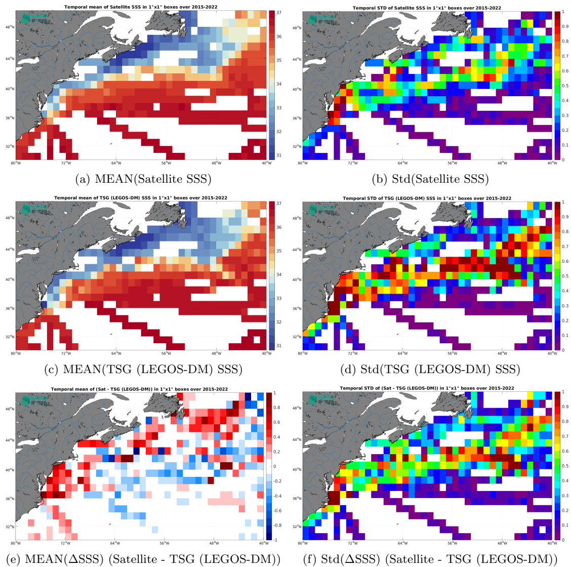
Figure 7: Temporal mean (left) and Std (right) of SSS from SMAP SSS L3 v5.3 - Monthly (RSS) (top), TSG (LEGOS-DM) (middle), and of \Delta SSS (Satellite - TSG (LEGOS-DM)). Only match-up pairs are used to generate these maps.
