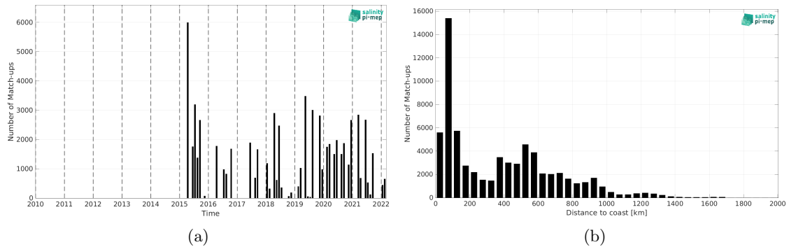
Figure 2: Number of match-ups between TSG (LEGOS-DM) and SMAP SSS L3 v5.3 - Monthly (RSS) SSS as a function of time (a) and as function of the distance to coast (b) over the Gulf Stream Pi-MEP region and for the full satellite product period.
