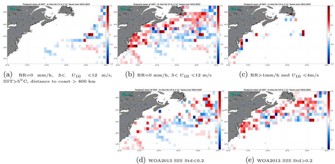
Figure 14: Temporal mean gridded over spatial boxes of size 1^\circ \times 1^\circ of \Delta SSS (SMAP SSS L3 v5.3 - Monthly (RSS) - TSG (LEGOS-DM)) for 5 different subdatasets corresponding to: RR=0 mm/h, 3 < U_{10} < 12 m/s, SST > 5°C, distance to coast > 800 km (a), RR=0 mm/h, 3 < U_{10} < 12 m/s (b), RR > 1mm/h and U_{10} < 4 m/s (c), WOA2013 SSS Std < 0.2 (d), WOA2013 SSS Std > 0.2 (e).
