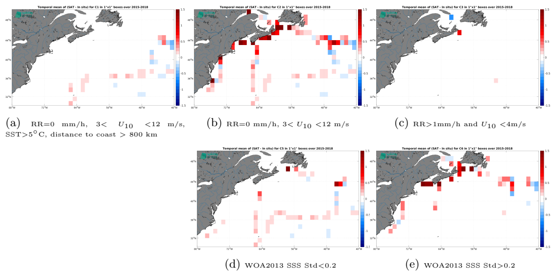
Figure 14: Temporal mean gridded over spatial boxes of size 1^\circ \times 1^\circ of \Delta SSS (SMAP SSS L3 v5.3 - Monthly (RSS) - TSG (GOSUD-Sailing-ship)) for 5 different subdatasets corresponding to: RR=0 mm/h, 3 < U_{10} < 12 m/s, SST>5°C, distance to coast > 800 km (a), RR=0 mm/h, 3 < U_{10} < 12 m/s (b), RR>1mm/h and U_{10} < 4 m/s (c), WOA2013 SSS Std<0.2 (d), WOA2013 SSS Std>0.2 (e).
