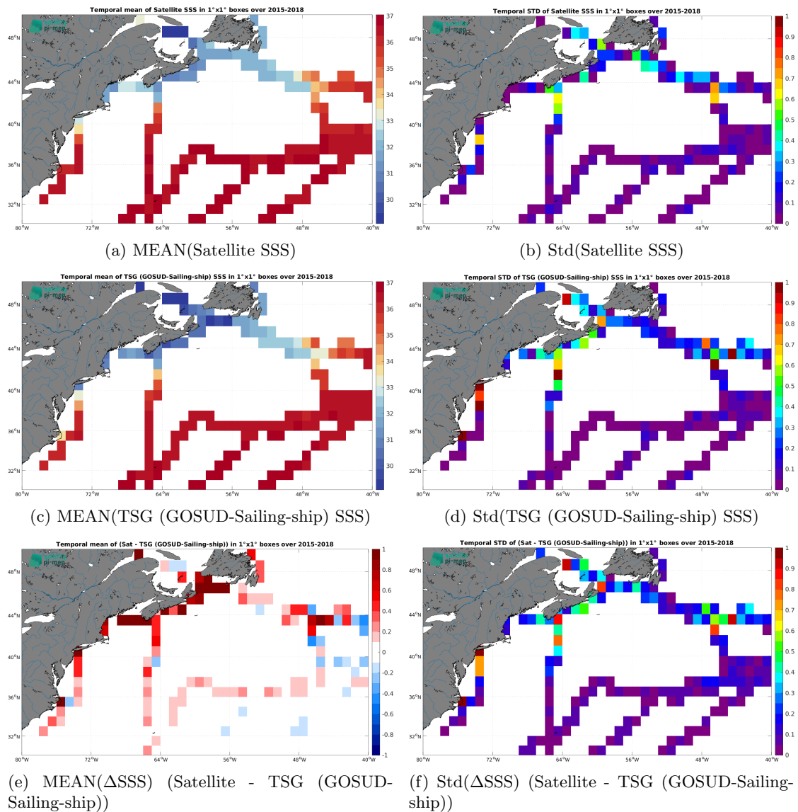
Figure 7: Temporal mean (left) and Std (right) of SSS from SMAP SSS L3 v5.3 - Monthly (RSS) (top), TSG (GOSUD-Sailing-ship) (middle), and of \Delta SSS (Satellite - TSG (GOSUD-Sailing-ship)). Only match-up pairs are used to generate these maps.
