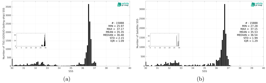
Figure 3: Histograms of SSS from TSG (GOSUD-Sailing-ship) (a) and SMAP SSS L3 v5.3 - Monthly (RSS) (b) considering all match-up pairs per bins of 0.1 over the Gulf Stream Pi-MEP region and for the full satellite product period.
