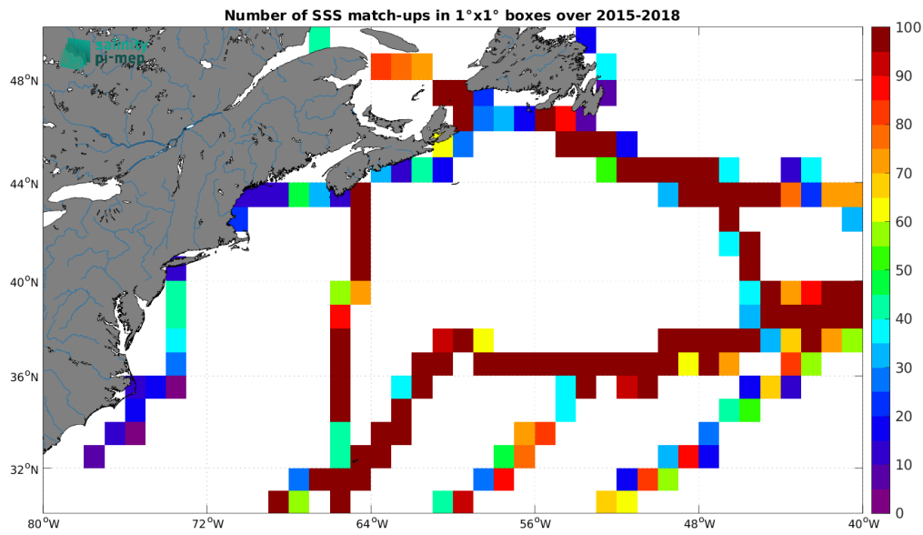
Figure 5: Number of SSS match-ups between TSG (GOSUD-Sailing-ship) SSS and the SMAP SSS L3 v5.3 - Monthly (RSS) SSS product for the Gulf Stream Pi-MEP region over 1^\circ \times 1^\circ boxes and for the full satellite product period.
