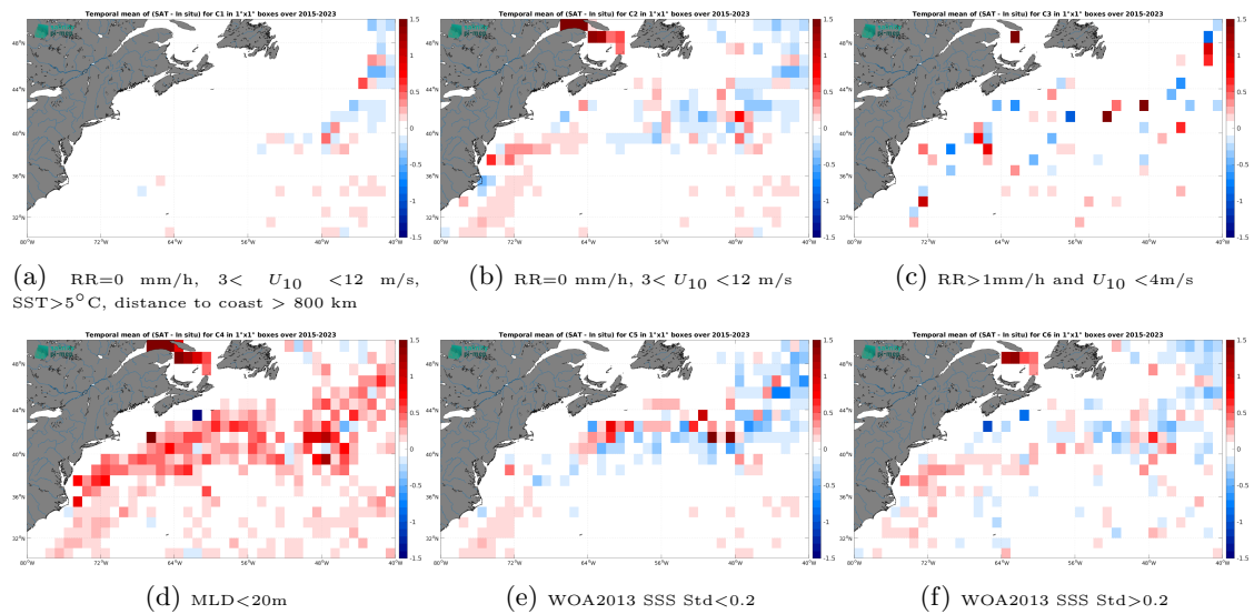
Figure 14: Temporal mean gridded over spatial boxes of size 1^\circ \times 1^\circ of \Delta SSS (SMAP SSS L3 v5.3 - Monthly (RSS) - Argo) for 6 different subdatasets corresponding to:RR=0 mm/h, 3 < U_{10} < 12 m/s, SST >5^\circ C, distance to coast > 800 km (a), RR=0 mm/h, 3 < U_{10} < 12 m/s (b), RR >1 mm/h and U_{10} < 4 m/s (c),MLD <20 m (d),WOA2013 SSS Std <0.2 (e),WOA2013 SSS Std >0.2 (f).
