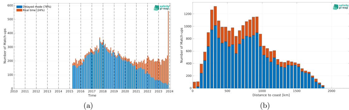
Figure 2: Number of match-ups between Argo and SMAP SSS L3 v5.3 - Monthly (RSS) SSS as a function of time (a) and as function of the distance to coast (b) over the Gulf Stream Pi-MEP region and for the full satellite product period.
