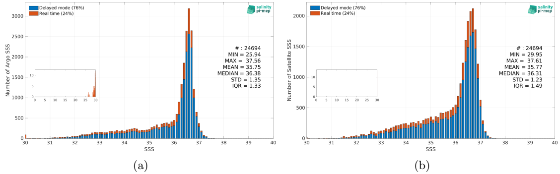
Figure 3: Histograms of SSS from Argo (a) and SMAP SSS L3 v5.3 - Monthly (RSS) (b) considering all match-up pairs per bins of 0.1 over the Gulf Stream Pi-MEP region and for the full satellite product period.
