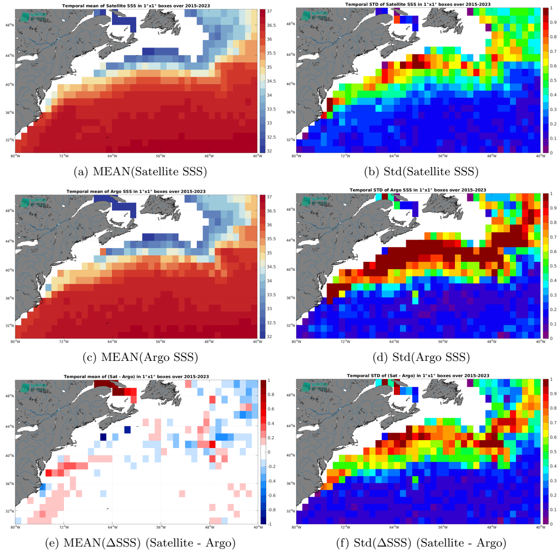
Figure 7: Temporal mean (left) and Std (right) of SSS from SMAP SSS L3 v5.3 - Monthly (RSS) (top), Argo (middle), and of \Delta SSS (Satellite - Argo). Only match-up pairs are used to generate these maps.
