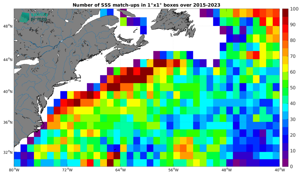
Figure 5: Number of SSS match-ups between Argo SSS and the SMAP SSS L3 v5.3 - Monthly (RSS) SSS product for the Gulf Stream Pi-MEP region over 1^\circ \times 1^\circ boxes and for the full satellite product period.
