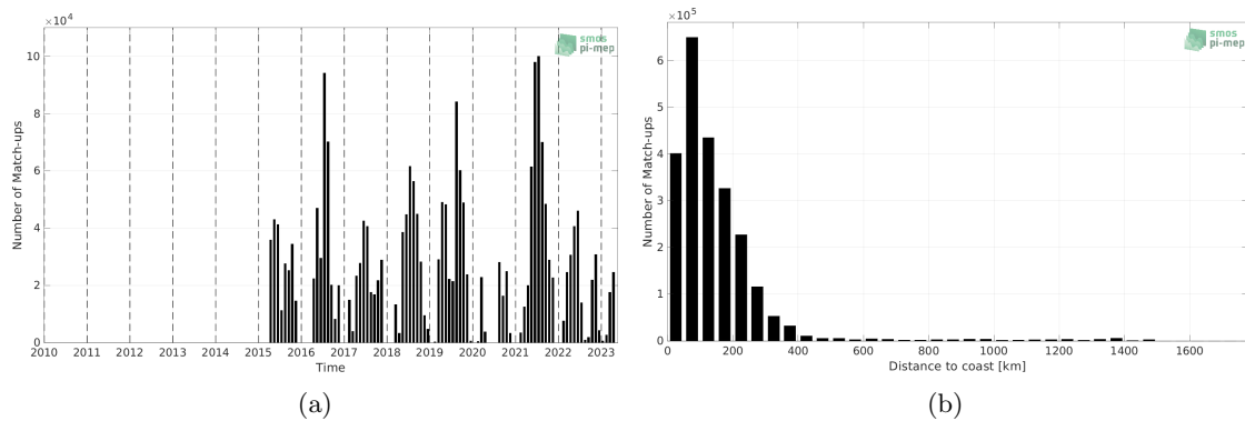
Figure 1: Number of match-ups between TSG (SAMOS) and SMAP SSS L3 v5 - 8-Day running (RSS) SSS as a function of time (a) and as function of the distance to coast (b) over the Gulf Stream Pi-MEP region and for the full satellite product period.
