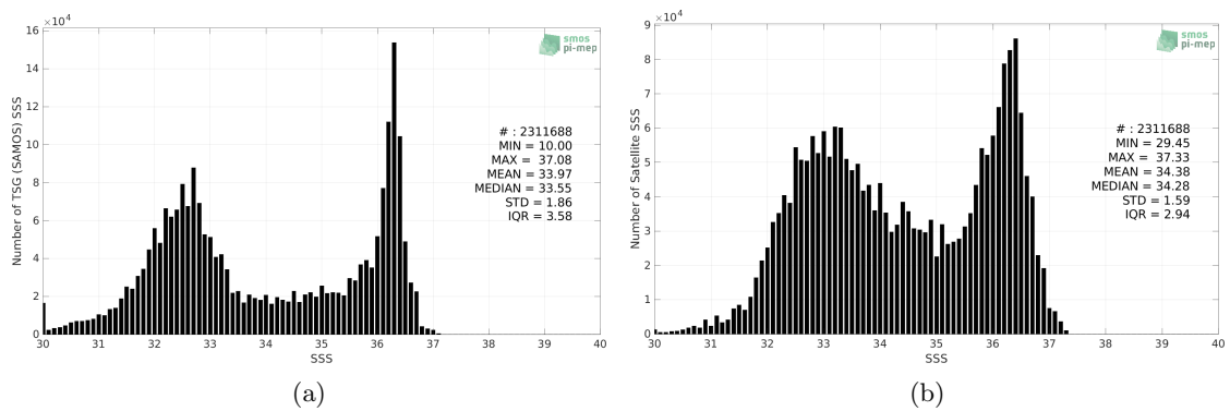
Figure 2: Histograms of SSS from TSG (SAMOS) (a) and SMAP SSS L3 v5 - 8-Day running (RSS) (b) considering all match-up pairs per bins of 0.1 over the Gulf Stream Pi-MEP region and for the full satellite product period.
