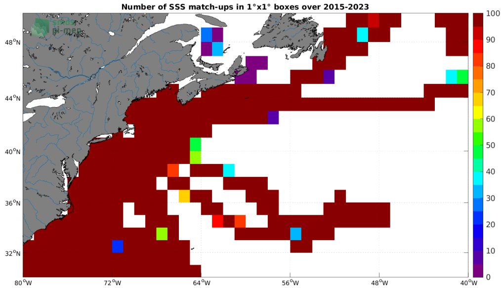
Figure 4: Number of SSS match-ups between TSG (SAMOS) SSS and the SMAP SSS L3 v5 - 8-Day running (RSS) SSS product for the Gulf Stream Pi-MEP region over 1^\circ \times 1^\circ boxes and for the full satellite product period.
