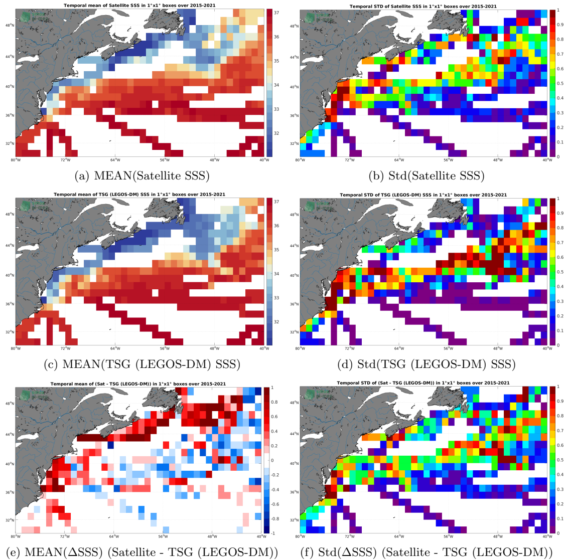
Figure 6: Temporal mean (left) and Std (right) of SSS from SMAP SSS L3 v5 - 8-Day running (RSS) (top), TSG (LEGOS-DM) (middle), and of \Delta SSS (Satellite - TSG (LEGOS-DM)). Only match-up pairs are used to generate these maps.
