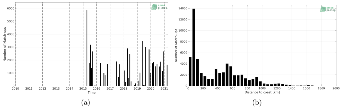
Figure 1: Number of match-ups between TSG (LEGOS-DM) and SMAP SSS L3 v5 - 8-Day running (RSS) SSS as a function of time (a) and as function of the distance to coast (b) over the Gulf Stream Pi-MEP region and for the full satellite product period.
