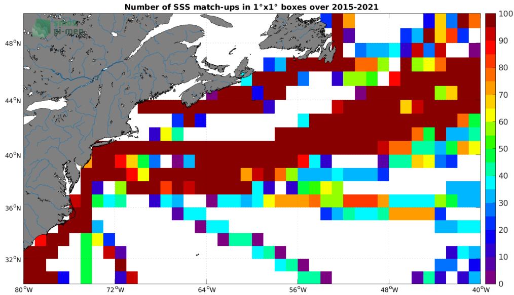
Figure 4: Number of SSS match-ups between TSG (LEGOS-DM) SSS and the SMAP SSS L3 v5 - 8-Day running (RSS) SSS product for the Gulf Stream Pi-MEP region over 1^\circ \times 1^\circ boxes and for the full satellite product period.
