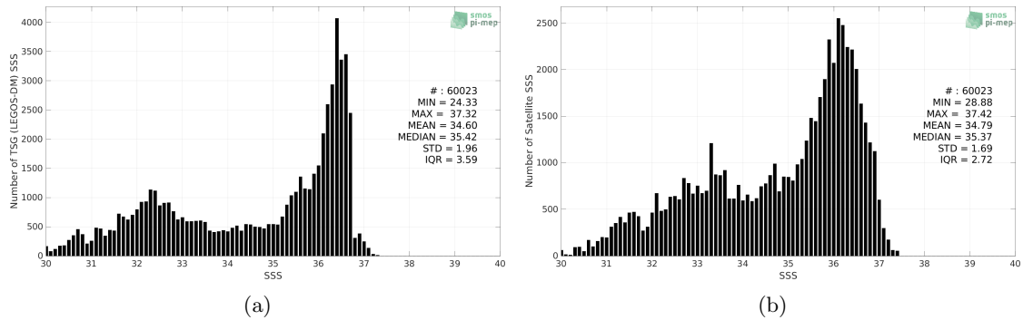
Figure 2: Histograms of SSS from TSG (LEGOS-DM) (a) and SMAP SSS L3 v5 - 8-Day running (RSS) (b) considering all match-up pairs per bins of 0.1 over the Gulf Stream Pi-MEP region and for the full satellite product period.
