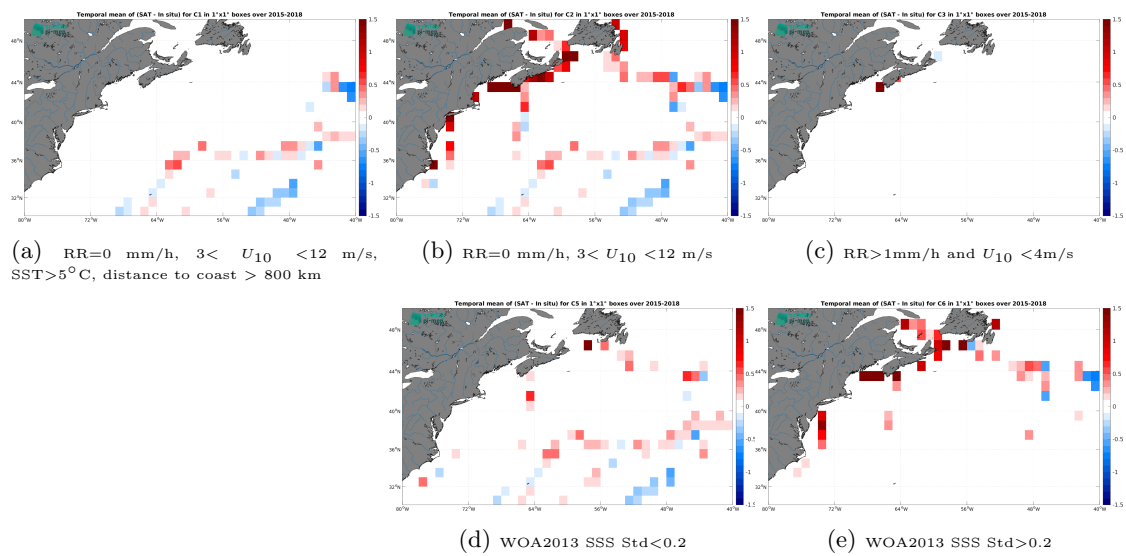
Figure 12: Temporal mean gridded over spatial boxes of size 1^\circ \times 1^\circ of \Delta\text{SSS} (SMAP SSS L3 v5 - 8-Day running (RSS) - TSG (GOSUD-Sailing-ship)) for 5 different subdatasets corresponding to:RR=0 mm/h, 3 < U_{10} < 12 m/s, SST >5^\circ\text{C} , distance to coast > 800 km (a), RR=0 mm/h, 3 < U_{10} < 12 m/s (b), RR >1 mm/h and U_{10} < 4 m/s (c), WOA2013 SSS Std <0.2 (d), WOA2013 SSS Std >0.2 (e).
