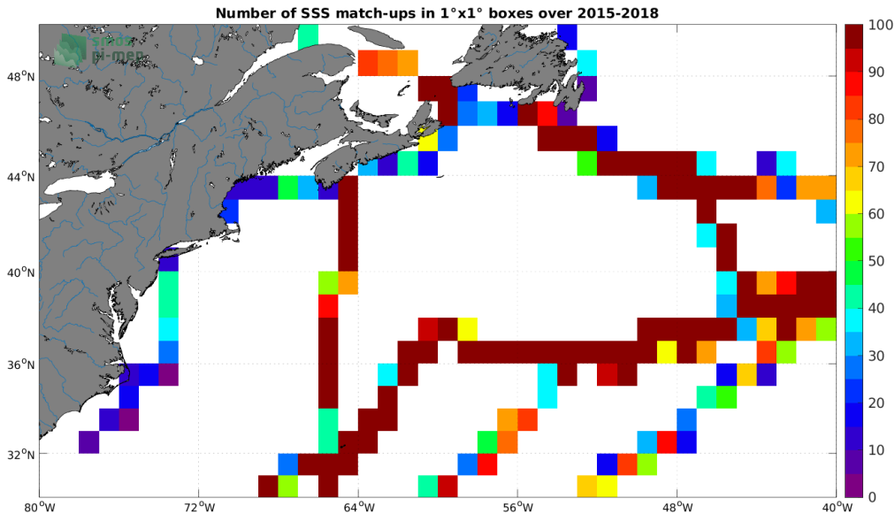
Figure 4: Number of SSS match-ups between TSG (GOSUD-Sailing-ship) SSS and the SMAP SSS L3 v5 - 8-Day running (RSS) SSS product for the Gulf Stream Pi-MEP region over 1^\circ \times 1^\circ boxes and for the full satellite product period.
