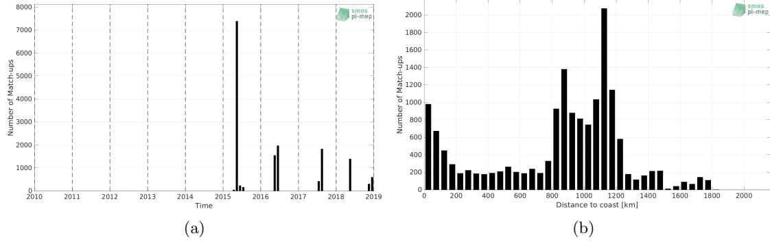
Figure 1: Number of match-ups between TSG (GOSUD-Sailing-ship) and SMAP SSS L3 v5 - 8-Day running (RSS) SSS as a function of time (a) and as function of the distance to coast (b) over the Gulf Stream Pi-MEP region and for the full satellite product period.
