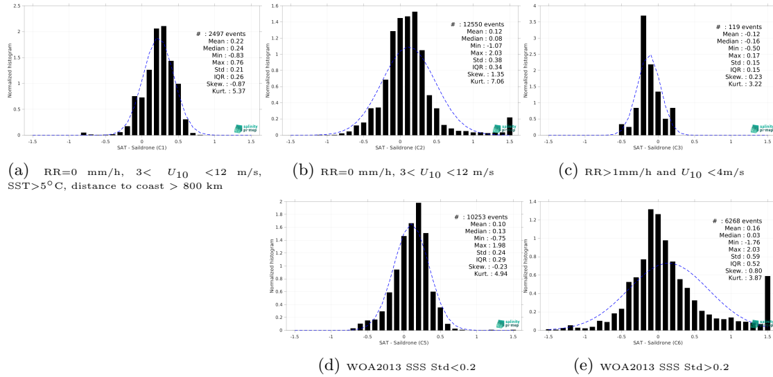
Figure 13: Normalized histogram of \Delta SSS (SMAP SSS L3 v5 - 8-Day running (RSS) - Saldrone) for 5 different subdatasets corresponding to: RR=0 mm/h, 3 < U_{10} < 12 m/s, SST>5°C, distance to coast > 800 km (a), RR=0 mm/h, 3 < U_{10} < 12 m/s (b), RR>1mm/h and U_{10} < 4 m/s (c), WOA2013 SSS Std<0.2 (d), WOA2013 SSS Std>0.2 (e).
