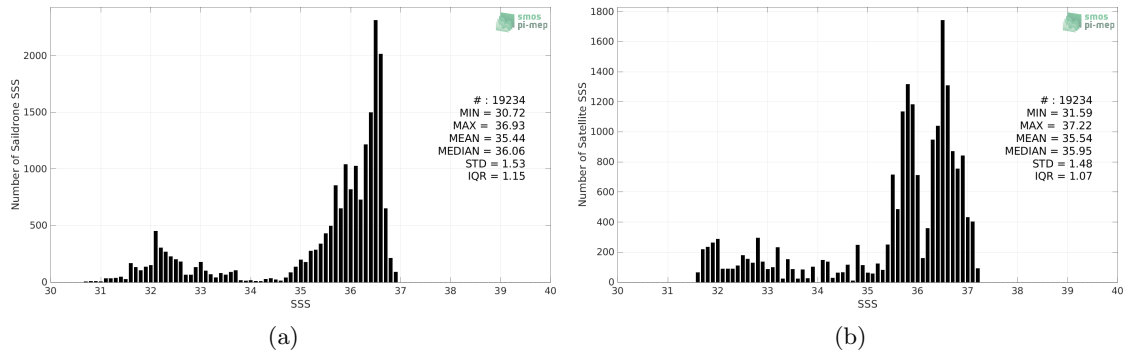
Figure 2: Histograms of SSS from Saildrone (a) and SMAP SSS L3 v5 - 8-Day running (RSS) (b) considering all match-up pairs per bins of 0.1 over the Gulf Stream Pi-MEP region and for the full satellite product period.
