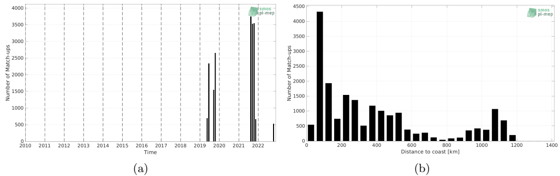
Figure 1: Number of match-ups between Saildrone and SMAP SSS L3 v5 - 8-Day running (RSS) SSS as a function of time (a) and as function of the distance to coast (b) over the Gulf Stream Pi-MEP region and for the full satellite product period.
