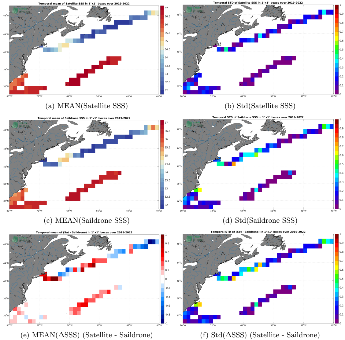
Figure 6: Temporal mean (left) and Std (right) of SSS from SMAP SSS L3 v5 - 8-Day running (RSS) (top), Saildrone (middle), and of \Delta SSS (Satellite - Saildrone). Only match-up pairs are used to generate these maps.
