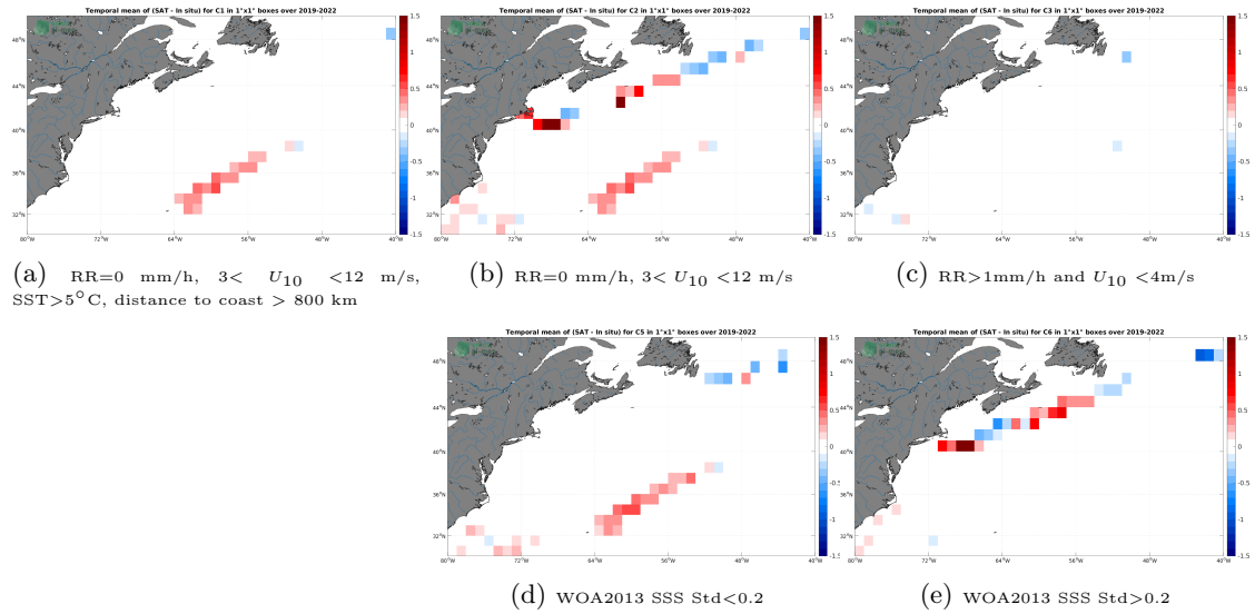
Figure 12: Temporal mean gridded over spatial boxes of size 1^\circ \times 1^\circ of \Delta SSS (SMAP SSS L3 v5 - 8-Day running (RSS) - Sairdrone) for 5 different subdatasets corresponding to:RR=0 mm/h, 3 < U_{10} < 12 m/s, SST >5^\circ C, distance to coast > 800 km (a), RR=0 mm/h, 3 < U_{10} < 12 m/s (b), RR >1 mm/h and U_{10} < 4 m/s (c), WOA2013 SSS Std <0.2 (d), WOA2013 SSS Std >0.2 (e).
