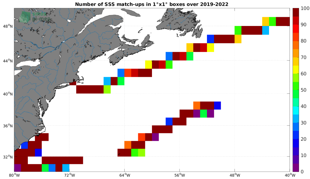
Figure 4: Number of SSS match-ups between Saildrone SSS and the SMAP SSS L3 v5 - 8-Day running (RSS) SSS product for the Gulf Stream Pi-MEP region over 1^\circ \times 1^\circ boxes and for the full satellite product period.
