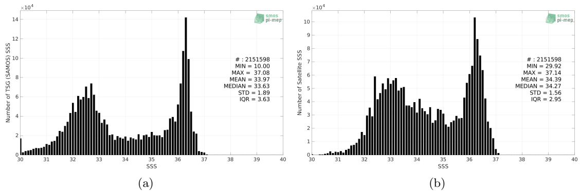
Figure 2: Histograms of SSS from TSG (SAMOS) (a) and SMAP SSS L3 v5 - Monthly (RSS) (b) considering all match-up pairs per bins of 0.1 over the Gulf Stream Pi-MEP region and for the full satellite product period.
