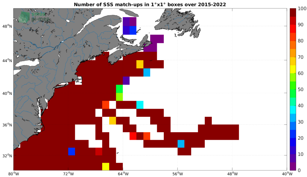
Figure 4: Number of SSS match-ups between TSG (SAMOS) SSS and the SMAP SSS L3 v5 - Monthly (RSS) SSS product for the Gulf Stream Pi-MEP region over 1^\circ \times 1^\circ boxes and for the full satellite product period.
