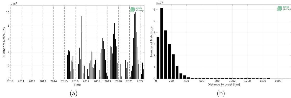
Figure 1: Number of match-ups between TSG (SAMOS) and SMAP SSS L3 v5 - Monthly (RSS) SSS as a function of time (a) and as function of the distance to coast (b) over the Gulf Stream Pi-MEP region and for the full satellite product period.
