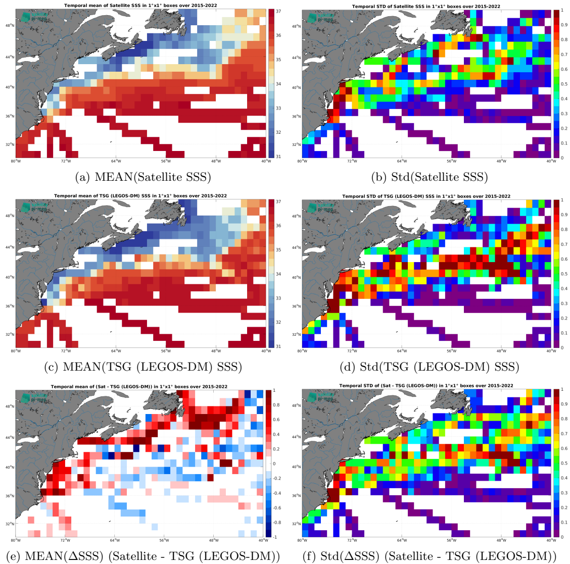
Figure 6: Temporal mean (left) and Std (right) of SSS from SMAP SSS L3 v5 - Monthly (RSS) (top), TSG (LEGOS-DM) (middle), and of \Delta SSS (Satellite - TSG (LEGOS-DM)). Only match-up pairs are used to generate these maps.
