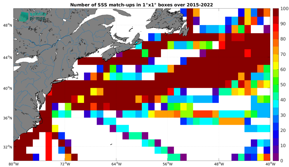
Figure 4: Number of SSS match-ups between TSG (LEGOS-DM) SSS and the SMAP SSS L3 v5 - Monthly (RSS) SSS product for the Gulf Stream Pi-MEP region over 1^\circ \times 1^\circ boxes and for the full satellite product period.
