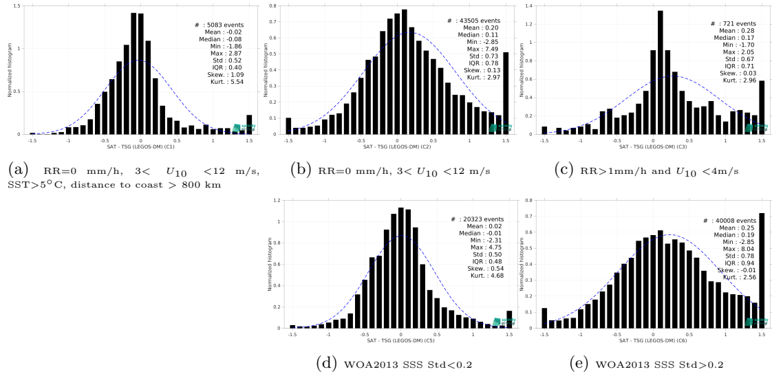
Figure 13: Normalized histogram of \Delta\text{SSS} (SMAP SSS L3 v5 - Monthly (RSS) - TSG (LEGOS-DM)) for 5 different subdatasets corresponding to: RR=0 mm/h, 3 < U_{10} < 12 m/s, SST > 5^\circ\text{C} , distance to coast > 800 km (a), RR=0 mm/h, 3 < U_{10} < 12 m/s (b), RR > 1 mm/h and U_{10} < 4 m/s (c), WOA2013 SSS Std < 0.2 (d), WOA2013 SSS Std > 0.2 (e).
