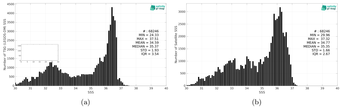
Figure 2: Histograms of SSS from TSG (LEGOS-DM) (a) and SMAP SSS L3 v5 - Monthly (RSS) (b) considering all match-up pairs per bins of 0.1 over the Gulf Stream Pi-MEP region and for the full satellite product period.
