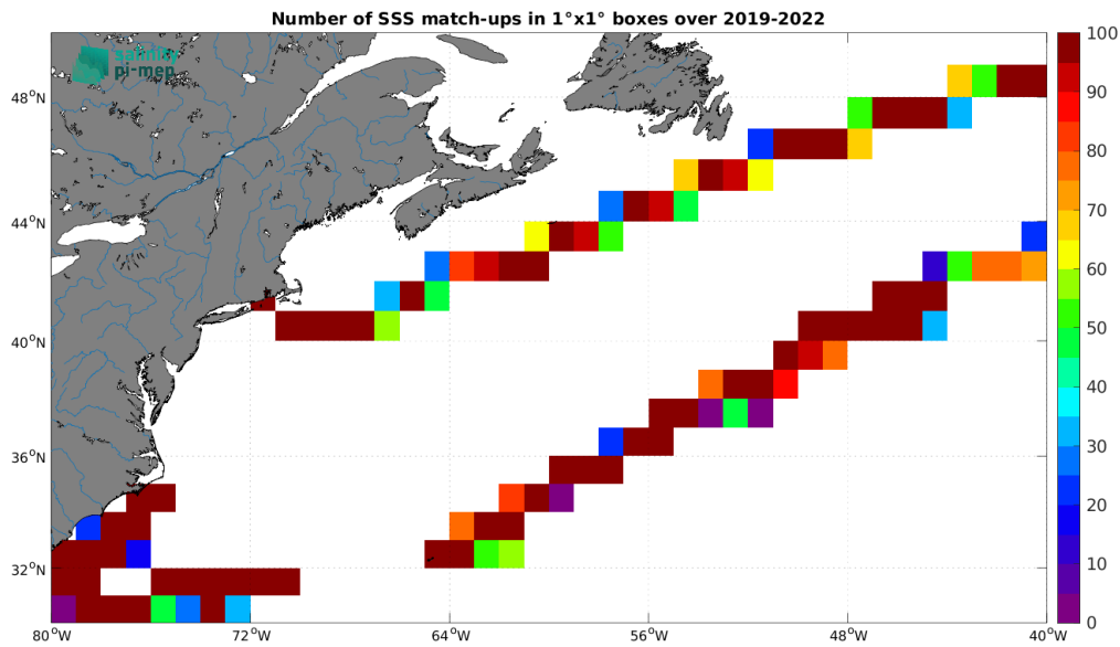
Figure 4: Number of SSS match-ups between Saildrone SSS and the SMAP SSS L3 v5 - Monthly (RSS) SSS product for the Gulf Stream Pi-MEP region over 1^\circ \times 1^\circ boxes and for the full satellite product period.
