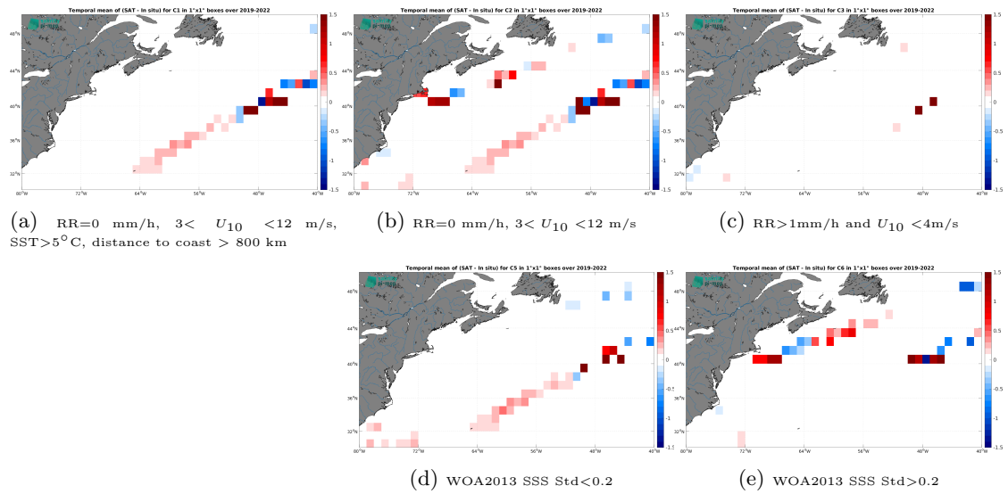
Figure 12: Temporal mean gridded over spatial boxes of size 1^\circ \times 1^\circ of \Delta SSS (SMAP SSS L3 v5 - Monthly (RSS) - Saildrone) for 5 different subdatasets corresponding to:RR=0 mm/h, 3 < U_{10} < 12 m/s, SST >5^\circ C, distance to coast > 800 km (a), RR=0 mm/h, 3 < U_{10} < 12 m/s (b), RR >1 mm/h and U_{10} < 4 m/s (c), WOA2013 SSS Std <0.2 (d), WOA2013 SSS Std >0.2 (e).
