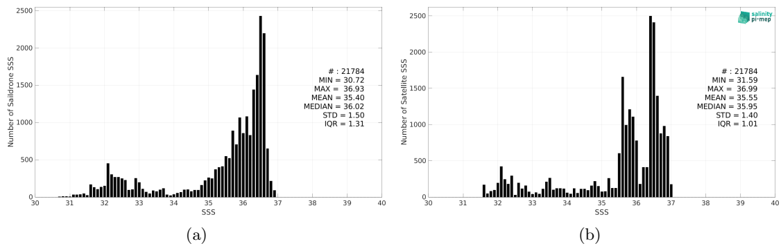
Figure 2: Histograms of SSS from Saildrone (a) and SMAP SSS L3 v5 - Monthly (RSS) (b) considering all match-up pairs per bins of 0.1 over the Gulf Stream Pi-MEP region and for the full satellite product period.
