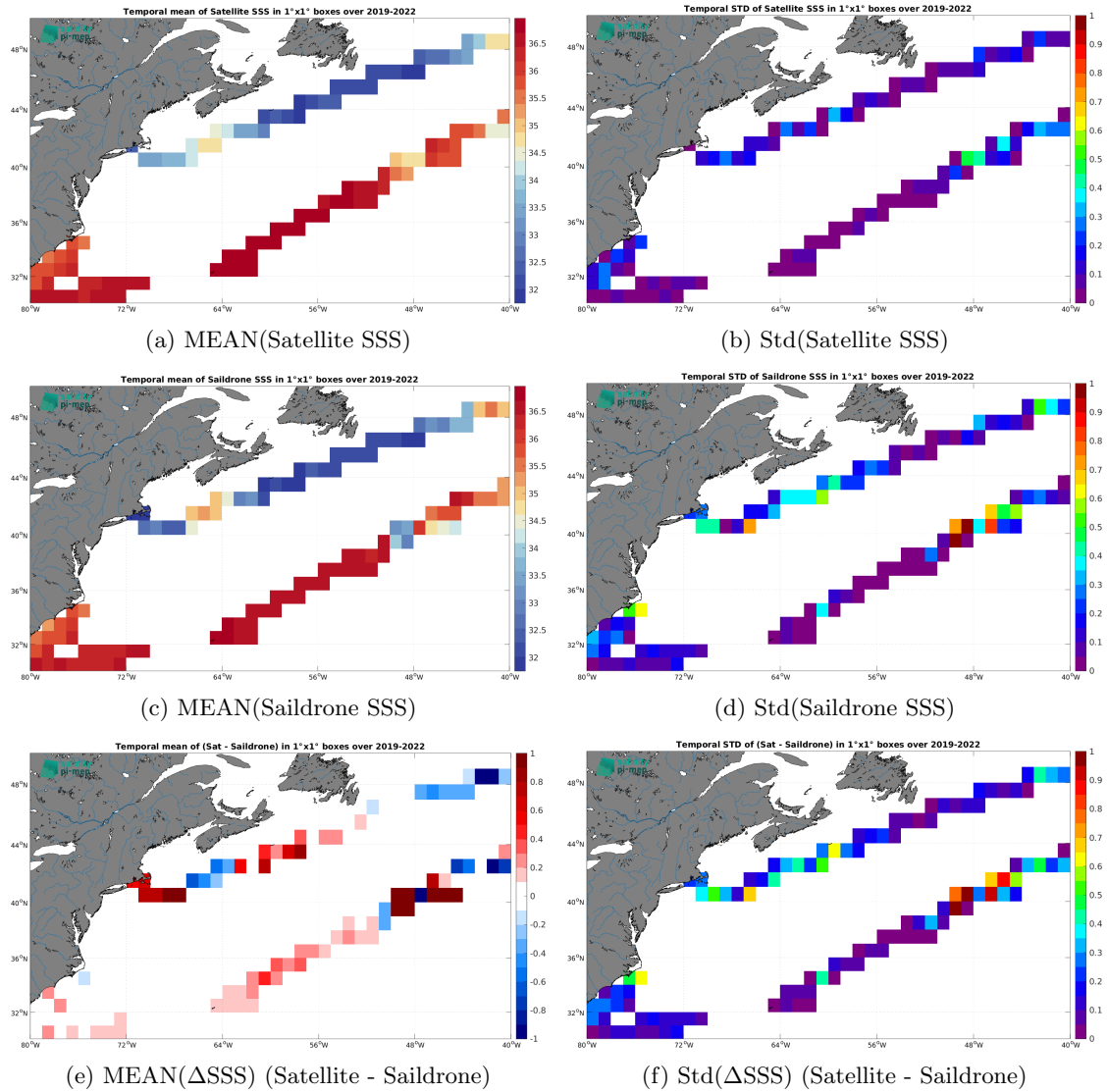
Figure 6: Temporal mean (left) and Std (right) of SSS from SMAP SSS L3 v5 - Monthly (RSS) (top), Saildrone (middle), and of \Delta SSS (Satellite - Saildrone). Only match-up pairs are used to generate these maps.
