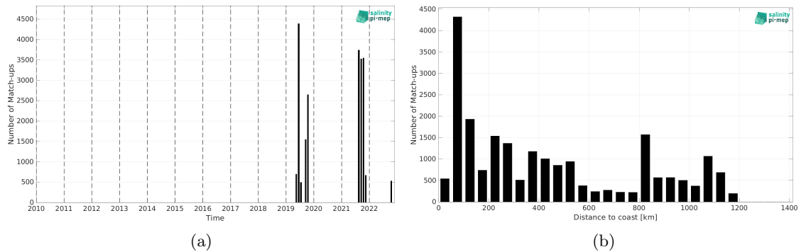
Figure 1: Number of match-ups between Saildrone and SMAP SSS L3 v5 - Monthly (RSS) SSS as a function of time (a) and as function of the distance to coast (b) over the Gulf Stream Pi-MEP region and for the full satellite product period.
