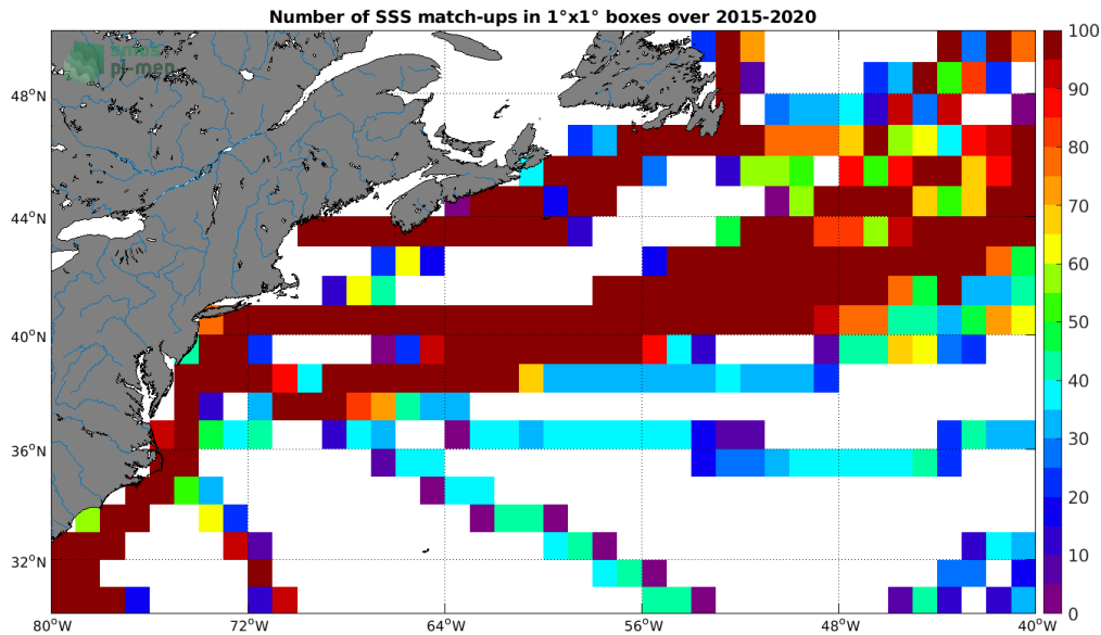
Figure 4: Number of SSS match-ups between TSG (LEGOS-DM) SSS and the SMAP SSS L3 v4 - 8-Day running (RSS) SSS product for the Gulf Stream Pi-MEP region over 1°x1° boxes and for the full satellite product period.
