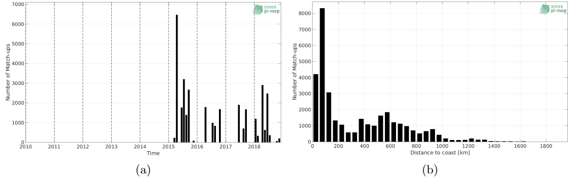
Figure 1: Number of match-ups between TSG-LEGOS-DM and SMAP-L3-RSS-V4-8DAY-RUNNING SSS as a function of time (a) and as function of the distance to coast (b) over the Gulf Stream Pi-MEP region and for the full satellite product period.
