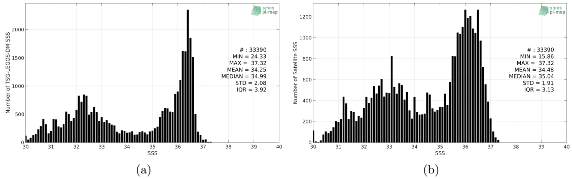
Figure 2: Histograms of SSS from TSG-LEGOS-DM (a) and SMAP-L3-RSS-V4-8DAY-RUNNING (b) considering all match-up pairs per bins of 0.1 over the Gulf Stream Pi-MEP region and for the full satellite product period.
