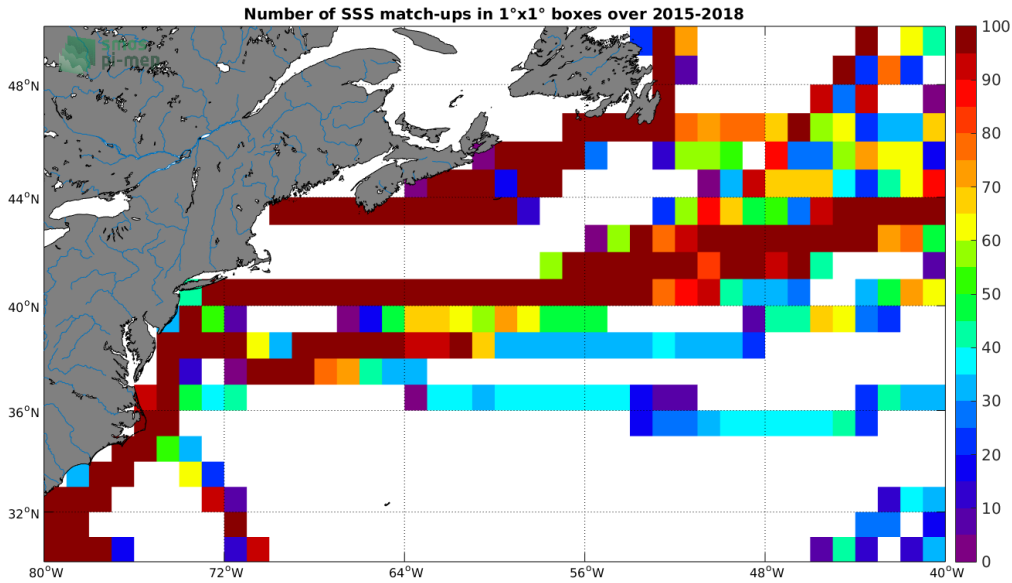
Figure 4: Number of SSS match-ups between TSG-LEGOS-DM SSS and the SMAP-L3-RSS-V4-8DAY-RUNNING SSS product for the Gulf Stream Pi-MEP region over 1^\circ \times 1^\circ boxes and for the full satellite product period.
