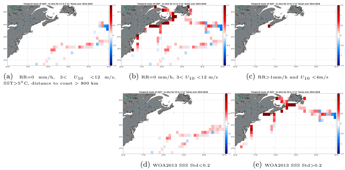
Figure 12: Temporal mean gridded over spatial boxes of size 1^\circ \times 1^\circ of \Delta SSS (SMAP SSS L3 v4 - 8-Day running (RSS) - TSG (GOSUD-Sailing-ship)) for 5 different subdatasets corresponding to:RR=0 mm/h, 3 < U_{10} < 12 m/s, SST>5°C, distance to coast > 800 km (a), RR=0 mm/h, 3 < U_{10} < 12 m/s (b), RR>1mm/h and U_{10} < 4 m/s (c), WOA2013 SSS Std<0.2 (d), WOA2013 SSS Std>0.2 (e).
