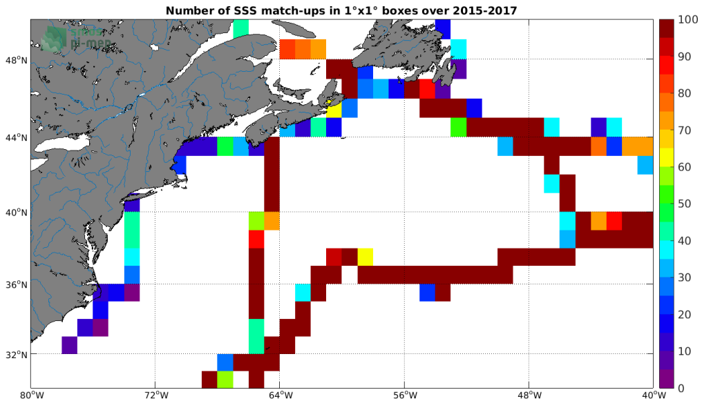
Figure 4: Number of SSS match-ups between TSG (GOSUD-Sailing-ship) SSS and the SMAP SSS L3 v4 - 8-Day running (RSS) SSS product for the Gulf Stream Pi-MEP region over 1°x1° boxes and for the full satellite product period.
