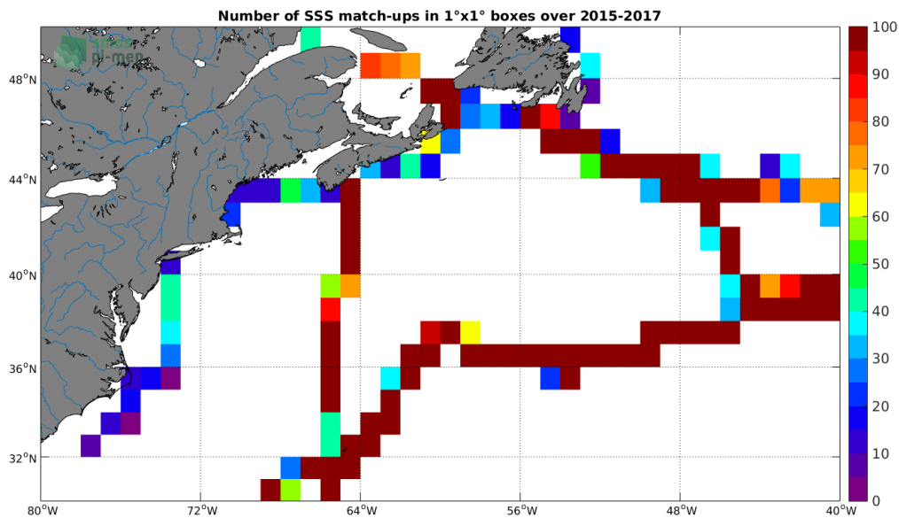
Figure 4: Number of SSS match-ups between TSG-GOSUD-Sailing-ship SSS and the SMAP-L3-RSS-V4-8DAY-RUNNING SSS product for the Gulf Stream Pi-MEP region over 1^\circ \times 1^\circ boxes and for the full satellite product period.
