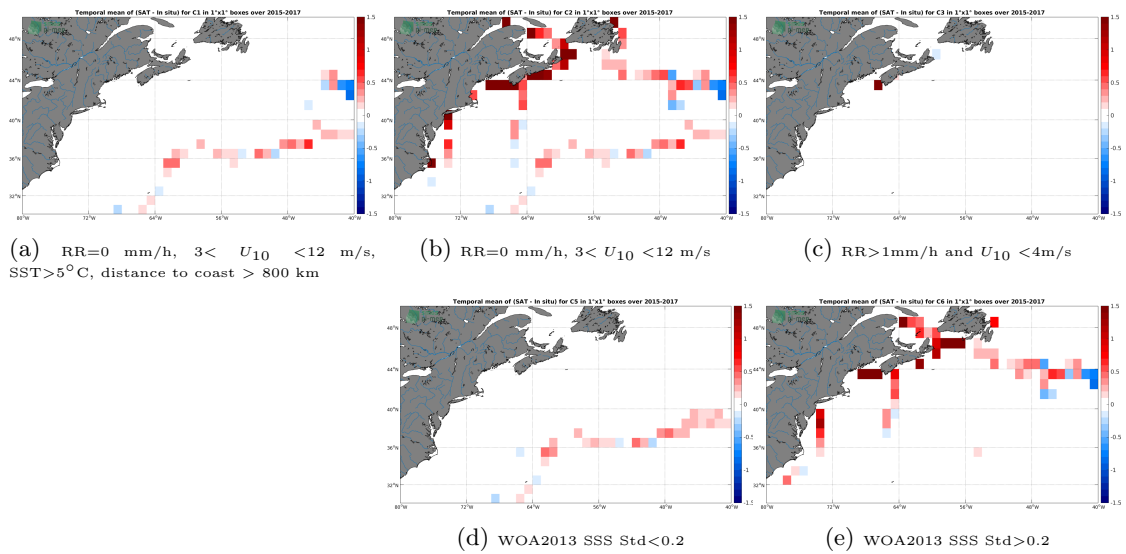
Figure 12: Temporal mean gridded over spatial boxes of size 1^\circ \times 1^\circ of \Delta SSS (SMAP-L3-RSS-V4-8DAY-RUNNING - TSG-GOSUD-Sailing-ship) for 5 different subdatasets corresponding to: RR=0 mm/h, 3 < U_{10} < 12 m/s, SST > 5°C, distance to coast > 800 km (a), RR=0 mm/h, 3 < U_{10} < 12 m/s (b), RR > 1mm/h and U_{10} < 4 m/s (c), WOA2013 SSS Std < 0.2 (d), WOA2013 SSS Std > 0.2 (e).
