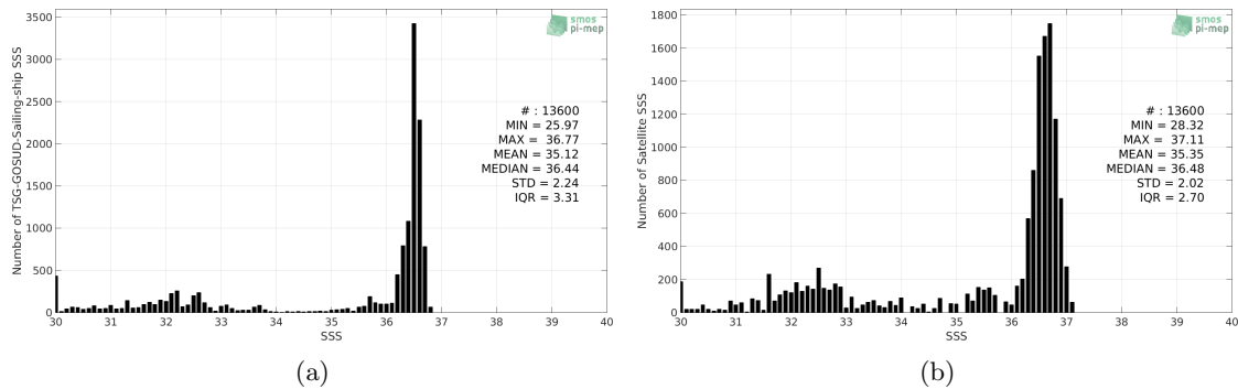
Figure 2: Histograms of SSS from TSG-GOSUD-Sailing-ship (a) and SMAP-L3-RSS-V4-8DAY-RUNNING (b) considering all match-up pairs per bins of 0.1 over the Gulf Stream Pi-MEP region and for the full satellite product period.
