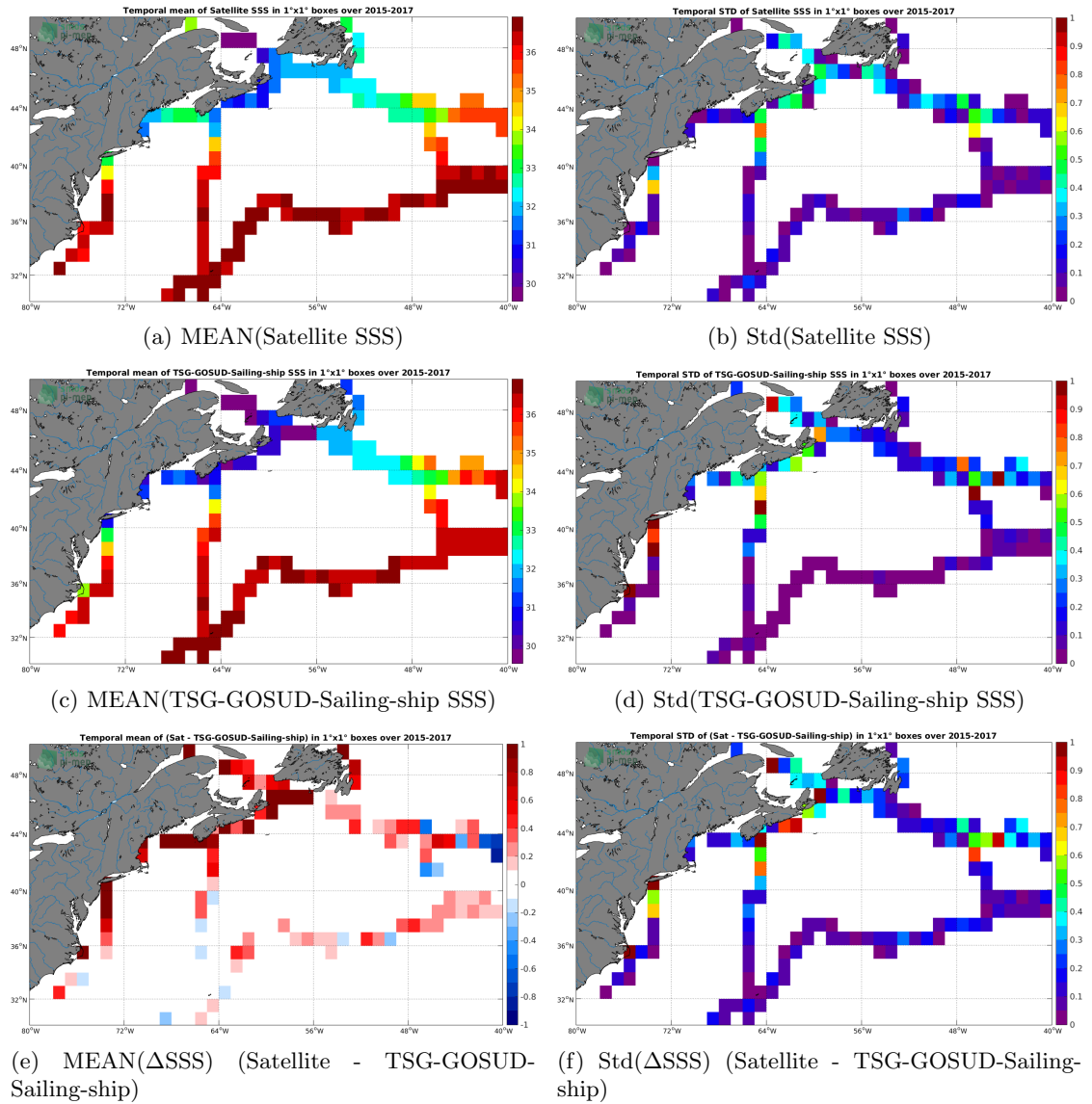
Figure 6: Temporal mean (left) and Std (right) of SSS from SMAP-L3-RSS-V4-8DAY-RUNNING (top), TSG-GOSUD-Sailing-ship (middle), and of \Delta SSS (Satellite - TSG-GOSUD-Sailing-ship). Only match-up pairs are used to generate these maps.
