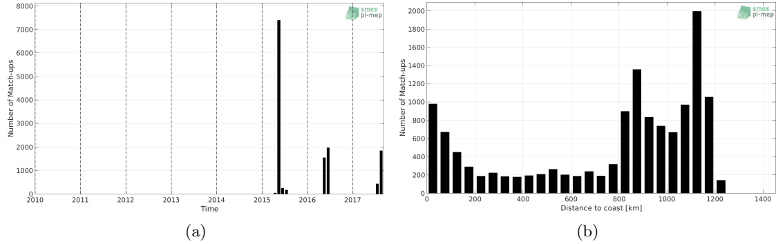
Figure 1: Number of match-ups between TSG-GOSUD-Sailing-ship and SMAP-L3-RSS-V4-8DAY-RUNNING SSS as a function of time (a) and as function of the distance to coast (b) over the Gulf Stream Pi-MEP region and for the full satellite product period.
