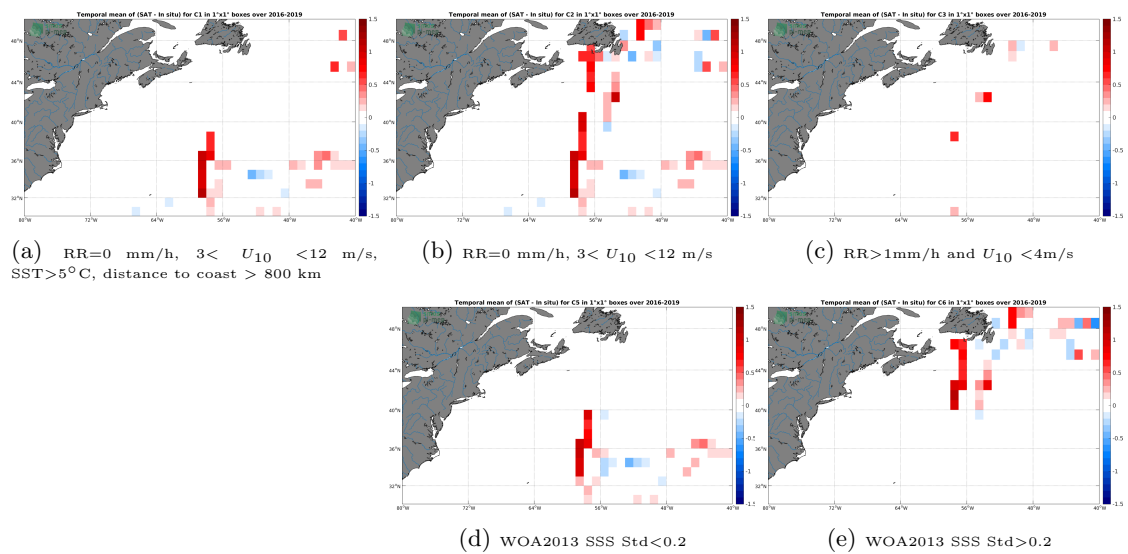
Figure 12: Temporal mean gridded over spatial boxes of size 1^\circ \times 1^\circ of \Delta\text{SSS} (SMAP SSS L3 v4 - 8-Day running (RSS) - TSG (GOSUD-Research-vessel)) for 5 different subdatasets corresponding to: RR=0 mm/h, 3 < U_{10} < 12 m/s, SST > 5°C, distance to coast > 800 km (a), RR=0 mm/h, 3 < U_{10} < 12 m/s (b), RR > 1 mm/h and U_{10} < 4 m/s (c), WOA2013 SSS Std < 0.2 (d), WOA2013 SSS Std > 0.2 (e).
