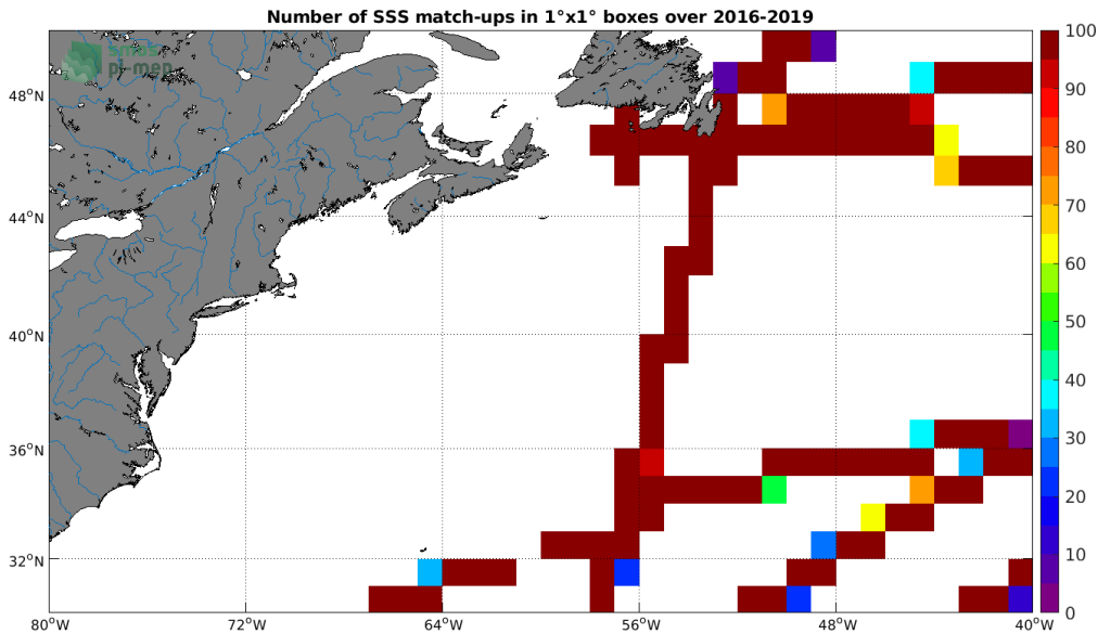
Figure 4: Number of SSS match-ups between TSG (GOSUD-Research-vessel) SSS and the SMAP SSS L3 v4 - 8-Day running (RSS) SSS product for the Gulf Stream Pi-MEP region over 1°x1° boxes and for the full satellite product period.
