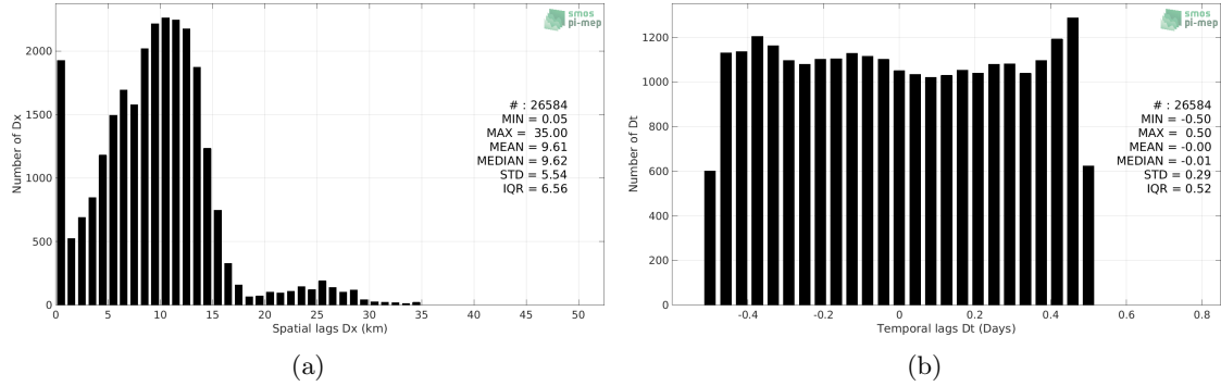
Figure 5: Histograms of the spatial (a) and temporal (b) lags between the time of the TSG (GOSUD-Research-vessel) measurements and the date of the corresponding SMAP SSS L3 v4 - 8-Day running (RSS) SSS product.
