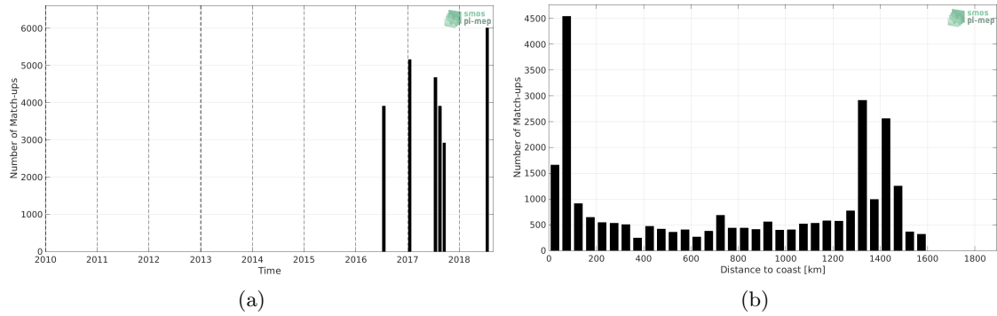
Figure 1: Number of match-ups between TSG (GOSUD-Research-vessel) and SMAP SSS L3 v4 - 8-Day running (RSS) SSS as a function of time (a) and as function of the distance to coast (b) over the Gulf Stream Pi-MEP region and for the full satellite product period.
