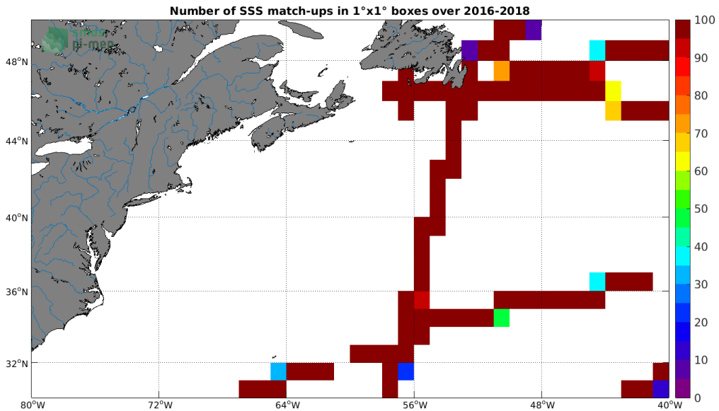
Figure 4: Number of SSS match-ups between TSG (GOSUD-Research-vessel) SSS and the SMAP SSS L3 v4 - 8-Day running (RSS) SSS product for the Gulf Stream Pi-MEP region over 1^\circ \times 1^\circ boxes and for the full satellite product period.
