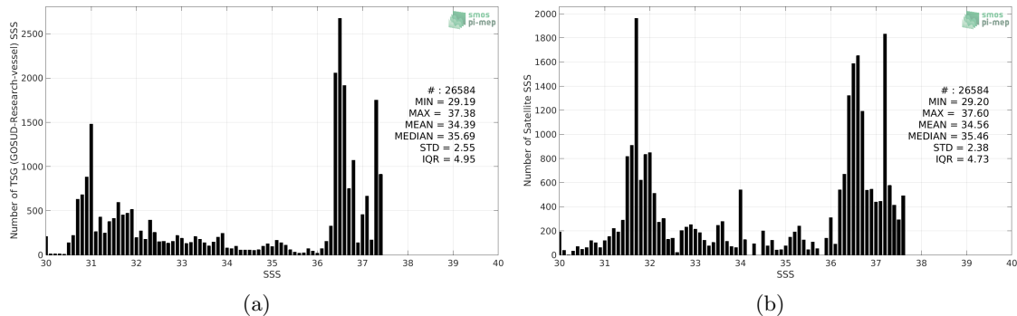
Figure 2: Histograms of SSS from TSG (GOSUD-Research-vessel) (a) and SMAP SSS L3 v4 - 8-Day running (RSS) (b) considering all match-up pairs per bins of 0.1 over the Gulf Stream Pi-MEP region and for the full satellite product period.
