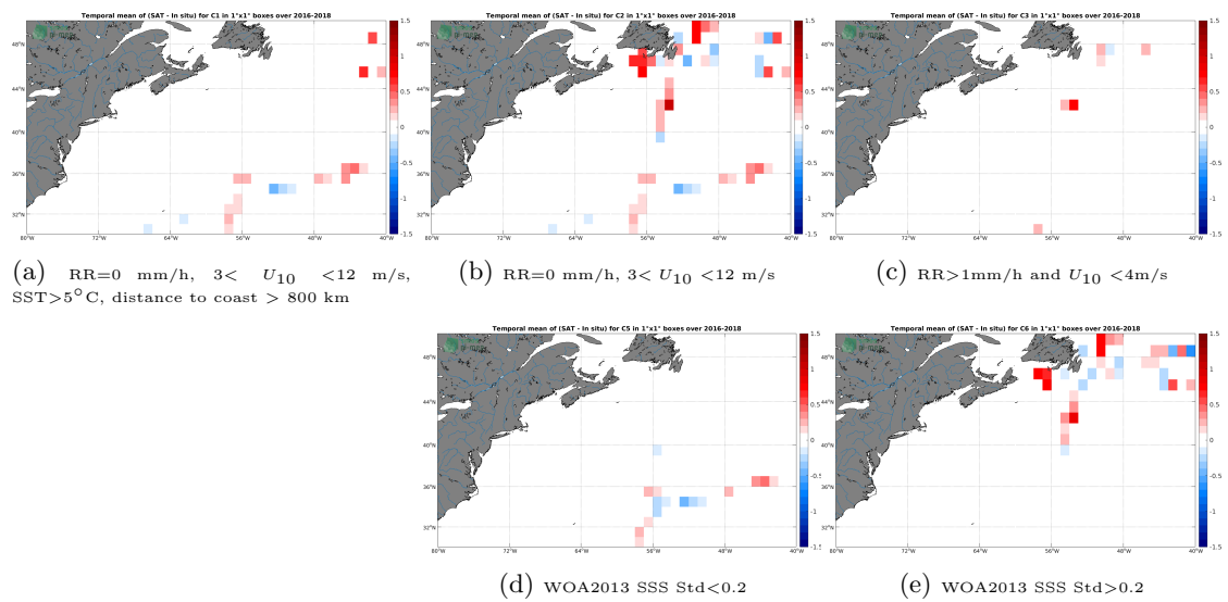
Figure 12: Temporal mean gridded over spatial boxes of size 1^\circ \times 1^\circ of \Delta SSS (SMAP SSS L3 v4 - 8-Day running (RSS) - TSG (GOSUD-Research-vessel)) for 5 different subdatasets corresponding to:RR=0 mm/h, 3 < U_{10} < 12 m/s, SST>5°C, distance to coast > 800 km (a), RR=0 mm/h, 3 < U_{10} < 12 m/s (b), RR>1mm/h and U_{10} < 4 m/s (c), WOA2013 SSS Std<0.2 (d), WOA2013 SSS Std>0.2 (e).
