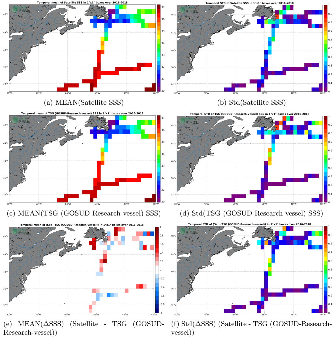
Figure 6: Temporal mean (left) and Std (right) of SSS from SMAP SSS L3 v4 - 8-Day running (RSS) (top), TSG (GOSUD-Research-vessel) (middle), and of \Delta SSS (Satellite - TSG (GOSUD-Research-vessel)). Only match-up pairs are used to generate these maps.
