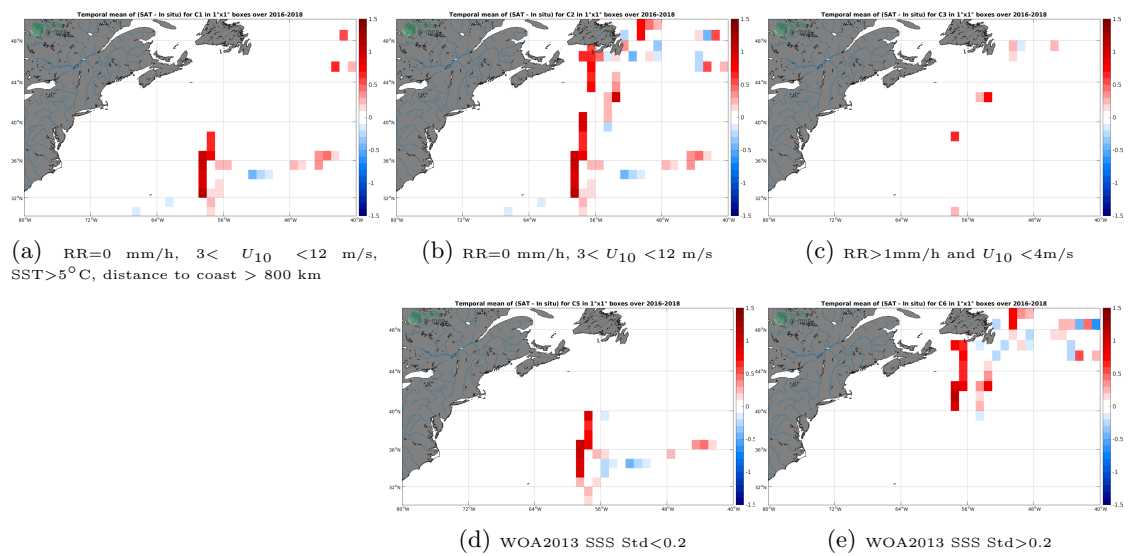
Figure 12: Temporal mean gridded over spatial boxes of size 1^\circ \times 1^\circ of \Delta SSS (SMAP-L3-RSS-V4-8DAY-RUNNING - TSG-GOSUD-Research-vessel) for 5 different subdatasets corresponding to: RR=0 mm/h, 3 < U_{10} < 12 m/s, SST > 5°C, distance to coast > 800 km (a), RR=0 mm/h, 3 < U_{10} < 12 m/s (b), RR > 1mm/h and U_{10} < 4 m/s (c), WOA2013 SSS Std < 0.2 (d), WOA2013 SSS Std > 0.2 (e).
