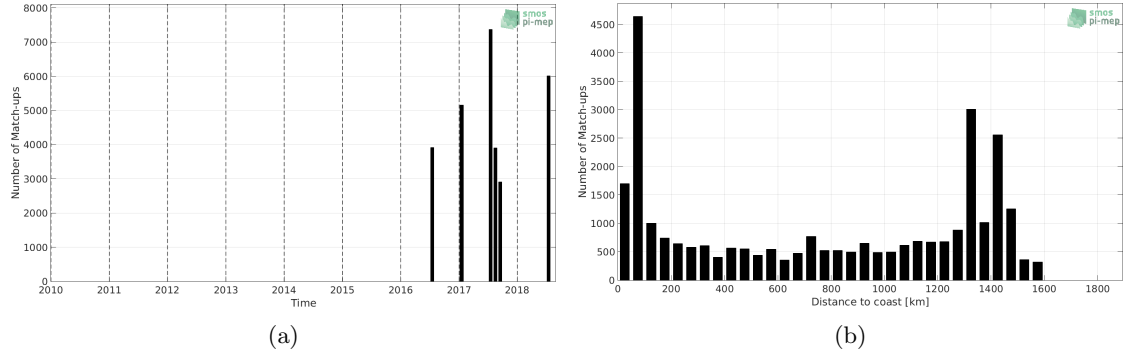
Figure 1: Number of match-ups between TSG-GOSUD-Research-vessel and SMAP-L3-RSS-V4-8DAY-RUNNING SSS as a function of time (a) and as function of the distance to coast (b) over the Gulf Stream Pi-MEP region and for the full satellite product period.
