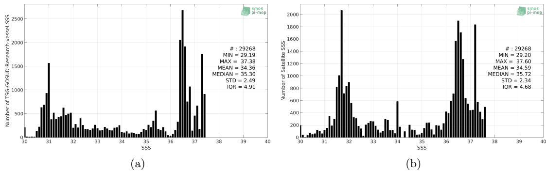
Figure 2: Histograms of SSS from TSG-GOSUD-Research-vessel (a) and SMAP-L3-RSS-V4-8DAY-RUNNING (b) considering all match-up pairs per bins of 0.1 over the Gulf Stream Pi-MEP region and for the full satellite product period.
