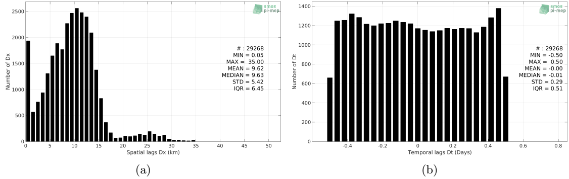
Figure 5: Histograms of the spatial (a) and temporal (b) lags between the time of the TSG-GOSUD-Research-vessel measurements and the date of the corresponding SMAP-L3-RSS-V4-8DAY-RUNNING SSS product.
