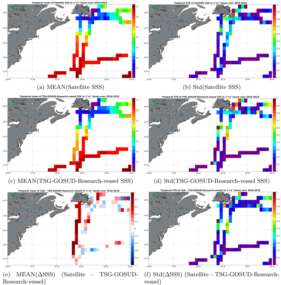
Figure 6: Temporal mean (left) and Std (right) of SSS from SMAP-L3-RSS-V4-8DAY-RUNNING (top), TSG-GOSUD-Research-vessel (middle), and of \Delta SSS (Satellite - TSG-GOSUD-Research-vessel). Only match-up pairs are used to generate these maps.
