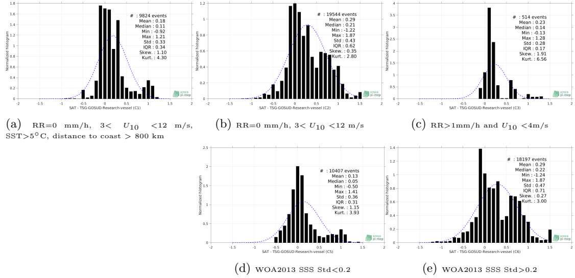
Figure 13: Normalized histogram of \Delta\text{SSS} (SMAP-L3-RSS-V4-8DAY-RUNNING - TSG-GOSUD-Research-vessel) for 5 different subdatasets corresponding to: RR=0 mm/h, 3 < U_{10} < 12 m/s, SST > 5^\circ\text{C} , distance to coast > 800 km (a), RR=0 mm/h, 3 < U_{10} < 12 m/s (b), RR > 1 mm/h and U_{10} < 4 m/s (c), WOA2013 SSS Std < 0.2 (d), WOA2013 SSS Std > 0.2 (e).
