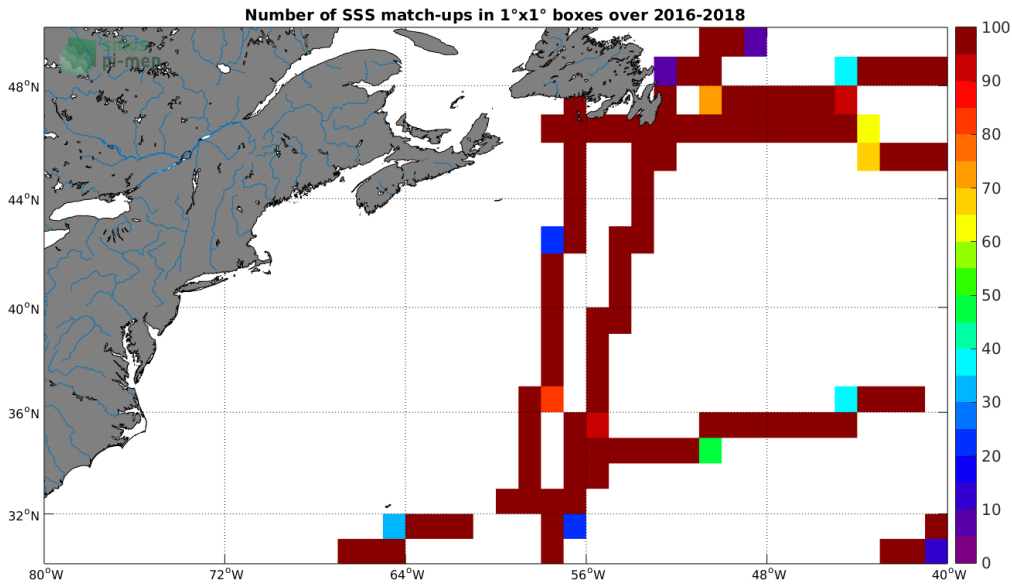
Figure 4: Number of SSS match-ups between TSG-GOSUD-Research-vessel SSS and the SMAP-L3-RSS-V4-8DAY-RUNNING SSS product for the Gulf Stream Pi-MEP region over 1°x1° boxes and for the full satellite product period.
