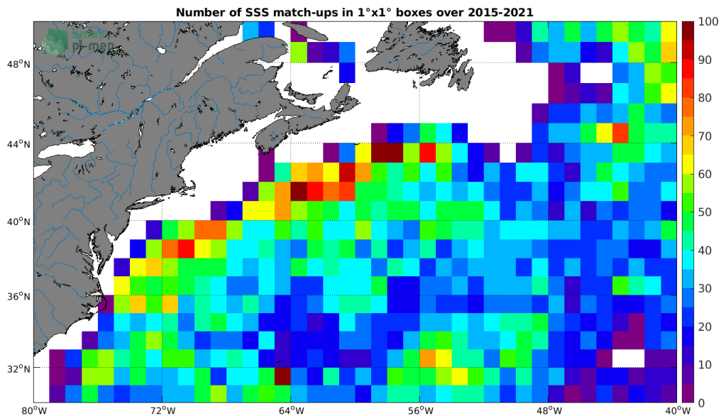
Figure 4: Number of SSS match-ups between Argo SSS and the SMAP SSS L3 v4 - 8-Day running (RSS) SSS product for the Gulf Stream Pi-MEP region over 1^\circ \times 1^\circ boxes and for the full satellite product period.
