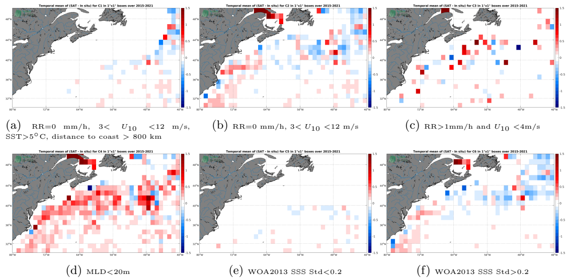
Figure 12: Temporal mean gridded over spatial boxes of size 1^\circ \times 1^\circ of \Delta SSS (SMAP SSS L3 v4 - 8-Day running (RSS) - Argo) for 6 different subdatasets corresponding to:RR=0 mm/h, 3 < U_{10} < 12 m/s, SST >5^\circ C, distance to coast > 800 km (a), RR=0 mm/h, 3 < U_{10} < 12 m/s (b), RR >1 mm/h and U_{10} < 4 m/s (c),MLD <20 m (d),WOA2013 SSS Std <0.2 (e),WOA2013 SSS Std >0.2 (f).
