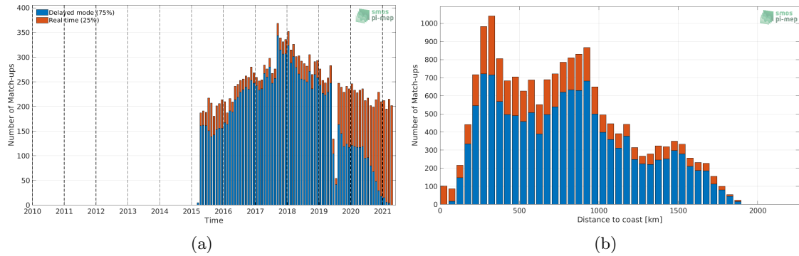
Figure 1: Number of match-ups between Argo and SMAP SSS L3 v4 - 8-Day running (RSS) SSS as a function of time (a) and as function of the distance to coast (b) over the Gulf Stream Pi-MEP region and for the full satellite product period.
