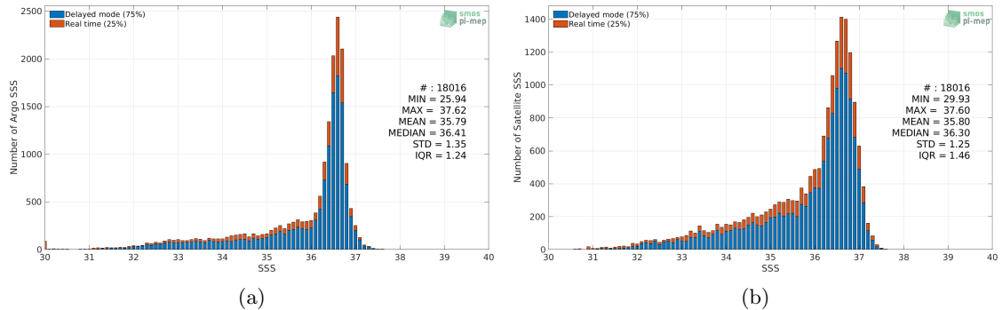
Figure 2: Histograms of SSS from Argo (a) and SMAP SSS L3 v4 - 8-Day running (RSS) (b) considering all match-up pairs per bins of 0.1 over the Gulf Stream Pi-MEP region and for the full satellite product period.
