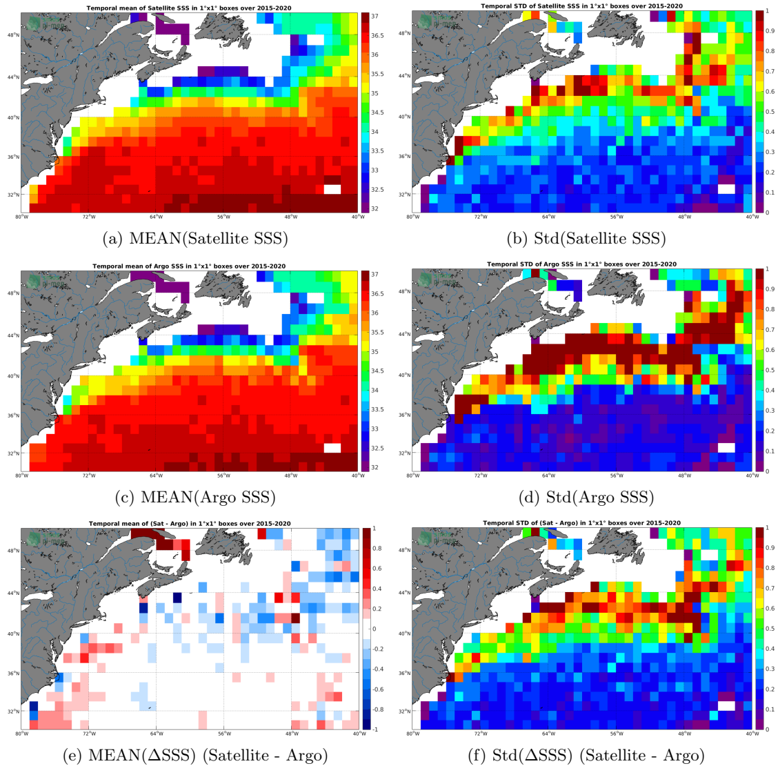
Figure 6: Temporal mean (left) and Std (right) of SSS from SMAP-L3-RSS-V4-8DAY-RUNNING (top), Argo (middle), and of \Delta SSS (Satellite - Argo). Only match-up pairs are used to generate these maps.
