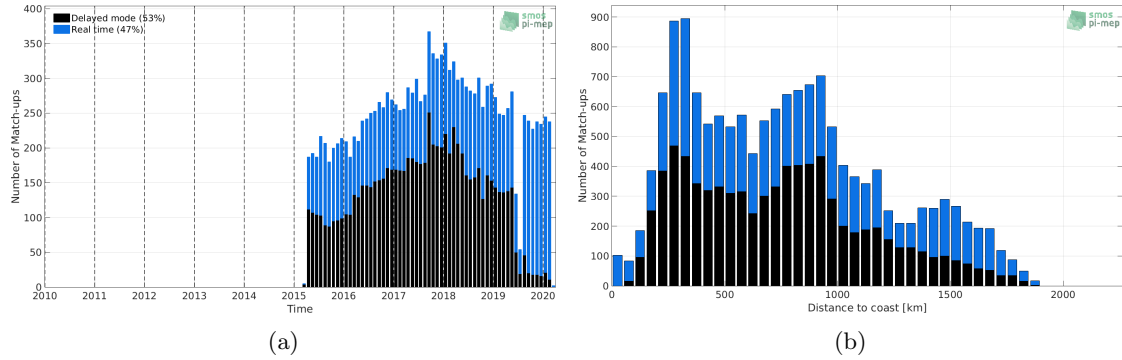
Figure 1: Number of match-ups between Argo and SMAP-L3-RSS-V4-8DAY-RUNNING SSS as a function of time (a) and as function of the distance to coast (b) over the Gulf Stream Pi-MEP region and for the full satellite product period.
