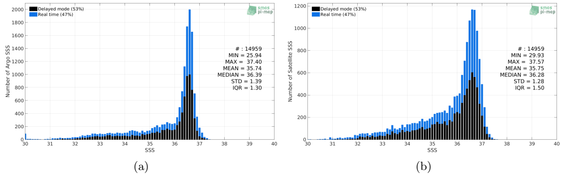
Figure 2: Histograms of SSS from Argo (a) and SMAP-L3-RSS-V4-8DAY-RUNNING (b) considering all match-up pairs per bins of 0.1 over the Gulf Stream Pi-MEP region and for the full satellite product period.
