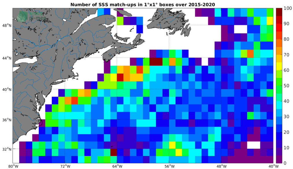
Figure 4: Number of SSS match-ups between Argo SSS and the SMAP-L3-RSS-V4-8DAY-RUNNING SSS product for the Gulf Stream Pi-MEP region over 1^\circ \times 1^\circ boxes and for the full satellite product period.
