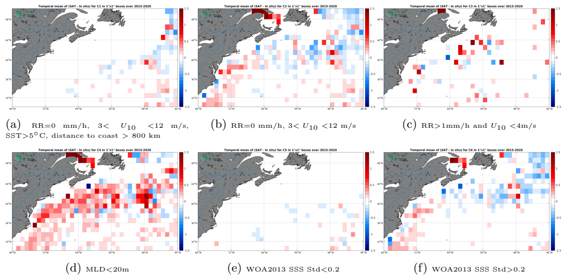
Figure 12: Temporal mean gridded over spatial boxes of size 1^\circ \times 1^\circ of \Delta SSS (SMAP-L3-RSS-V4-8DAY-RUNNING - Argo) for 6 different subdatasets corresponding to:RR=0 mm/h, 3 < U_{10} < 12 m/s, SST >5^\circ C, distance to coast > 800 km (a), RR=0 mm/h, 3 < U_{10} < 12 m/s (b), RR >1 mm/h and U_{10} < 4 m/s (c),MLD <20 m (d),WOA2013 SSS Std <0.2 (e),WOA2013 SSS Std >0.2 (f).
