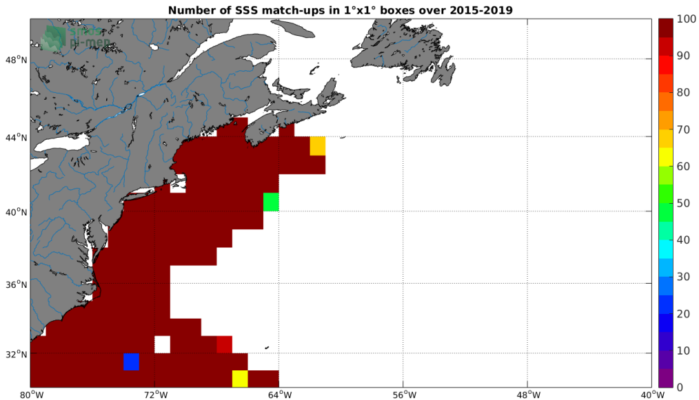
Figure 4: Number of SSS match-ups between TSG-SAMOS SSS and the SMAP-L3-RSS-V4-MONTHLY SSS product for the Gulf Stream Pi-MEP region over 1°x1° boxes and for the full satellite product period.
