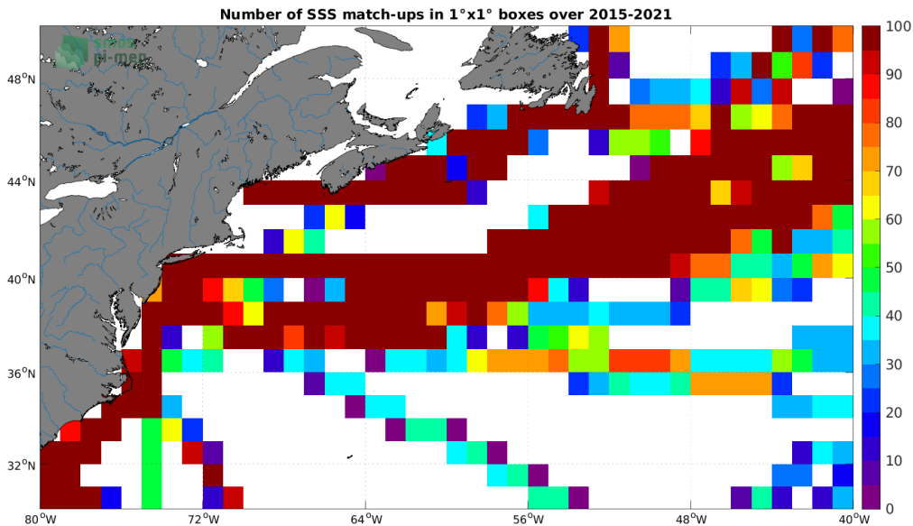
Figure 4: Number of SSS match-ups between TSG (LEGOS-DM) SSS and the SMAP SSS L3 v4 - Monthly (RSS) SSS product for the Gulf Stream Pi-MEP region over 1°×1° boxes and for the full satellite product period.
