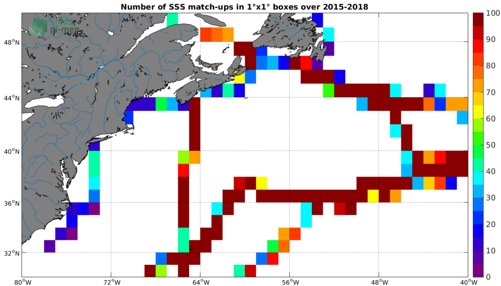
Figure 4: Number of SSS match-ups between TSG (GOSUD-Sailing-ship) SSS and the SMAP SSS L3 v4 - Monthly (RSS) SSS product for the Gulf Stream Pi-MEP region over 1^\circ \times 1^\circ boxes and for the full satellite product period.
