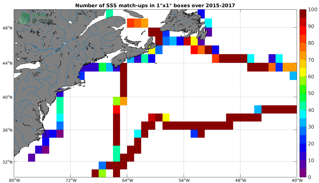
Figure 4: Number of SSS match-ups between TSG (GOSUD-Sailing-ship) SSS and the SMAP SSS L3 v4 - Monthly (RSS) SSS product for the Gulf Stream Pi-MEP region over 1°x1° boxes and for the full satellite product period.
