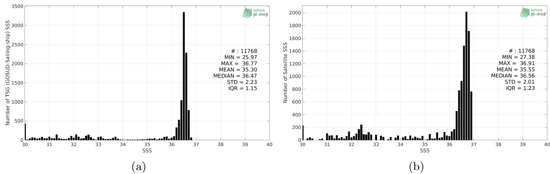
Figure 2: Histograms of SSS from TSG (GOSUD-Sailing-ship) (a) and SMAP SSS L3 v4 - Monthly (RSS) (b) considering all match-up pairs per bins of 0.1 over the Gulf Stream Pi-MEP region and for the full satellite product period.
