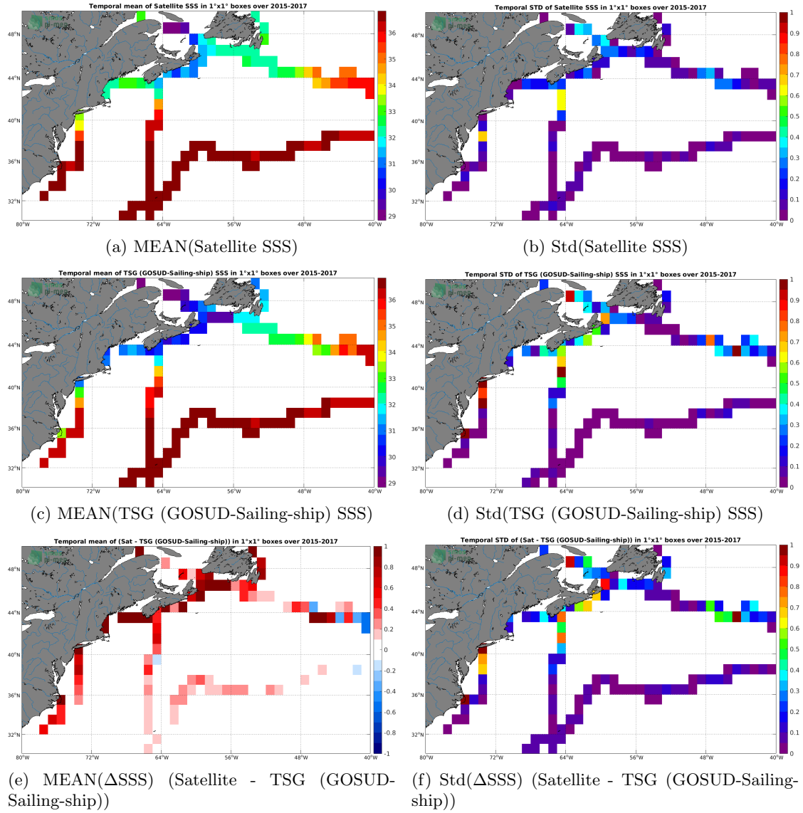
Figure 6: Temporal mean (left) and Std (right) of SSS from SMAP SSS L3 v4 - Monthly (RSS) (top), TSG (GOSUD-Sailing-ship) (middle), and of \Delta SSS (Satellite - TSG (GOSUD-Sailing-ship)). Only match-up pairs are used to generate these maps.
