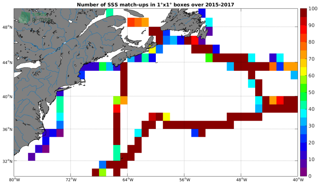
Figure 4: Number of SSS match-ups between TSG-GOSUD-Sailing-ship SSS and the SMAP-L3-RSS-V4-MONTHLY SSS product for the Gulf Stream Pi-MEP region over 1°x1° boxes and for the full satellite product period.
