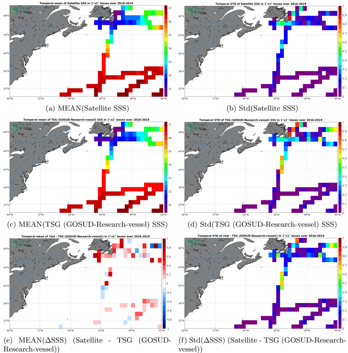
Figure 6: Temporal mean (left) and Std (right) of SSS from SMAP SSS L3 v4 - Monthly (RSS) (top), TSG (GOSUD-Research-vessel) (middle), and of \Delta SSS (Satellite - TSG (GOSUD-Research-vessel)). Only match-up pairs are used to generate these maps.
