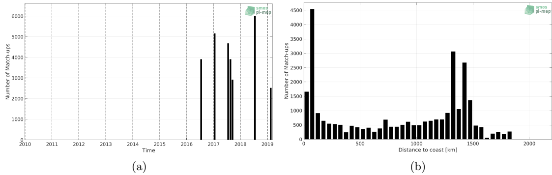
Figure 1: Number of match-ups between TSG (GOSUD-Research-vessel) and SMAP SSS L3 v4 - Monthly (RSS) SSS as a function of time (a) and as function of the distance to coast (b) over the Gulf Stream Pi-MEP region and for the full satellite product period.
