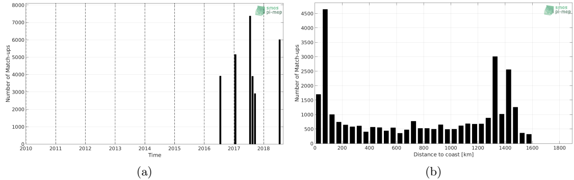
Figure 1: Number of match-ups between TSG-GOSUD-Research-vessel and SMAP-L3-RSS-V4-MONTHLY SSS as a function of time (a) and as function of the distance to coast (b) over the Gulf Stream Pi-MEP region and for the full satellite product period.
