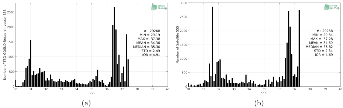
Figure 2: Histograms of SSS from TSG-GOSUD-Research-vessel (a) and SMAP-L3-RSS-V4-MONTHLY (b) considering all match-up pairs per bins of 0.1 over the Gulf Stream Pi-MEP region and for the full satellite product period.
