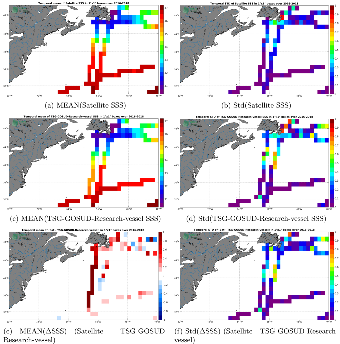
Figure 6: Temporal mean (left) and Std (right) of SSS from SMAP-L3-RSS-V4-MONTHLY (top), TSG-GOSUD-Research-vessel (middle), and of \Delta SSS (Satellite - TSG-GOSUD-Research-vessel). Only match-up pairs are used to generate these maps.
