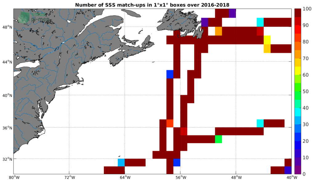
Figure 4: Number of SSS match-ups between TSG-GOSUD-Research-vessel SSS and the SMAP-L3-RSS-V4-MONTHLY SSS product for the Gulf Stream Pi-MEP region over 1°x1° boxes and for the full satellite product period.
