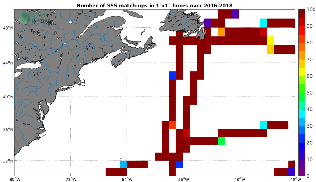
Figure 4: Number of SSS match-ups between TSG-GOSUD-Research-vessel SSS and the SMAP-L3-RSS-V4-MONTHLY SSS product for the Gulf Stream Pi-MEP region over 1^\circ \times 1^\circ boxes and for the full satellite product period.
