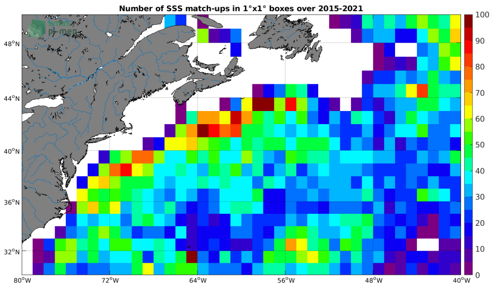
Figure 4: Number of SSS match-ups between Argo SSS and the SMAP SSS L3 v4 - Monthly (RSS) SSS product for the Gulf Stream Pi-MEP region over 1^\circ \times 1^\circ boxes and for the full satellite product period.
