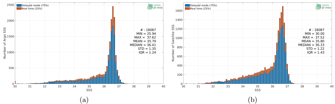
Figure 2: Histograms of SSS from Argo (a) and SMAP SSS L3 v4 - Monthly (RSS) (b) considering all match-up pairs per bins of 0.1 over the Gulf Stream Pi-MEP region and for the full satellite product period.
