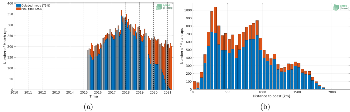
Figure 1: Number of match-ups between Argo and SMAP SSS L3 v4 - Monthly (RSS) SSS as a function of time (a) and as function of the distance to coast (b) over the Gulf Stream Pi-MEP region and for the full satellite product period.
