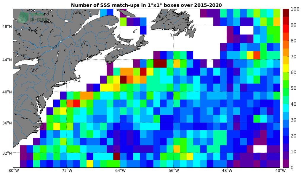
Figure 4: Number of SSS match-ups between Argos SSS and the SMAP SSS L3 v4 - Monthly (RSS) SSS product for the Gulf Stream Pi-MEP region over 1^{\circ} \times 1^{\circ} boxes and for the full satellite product period.
