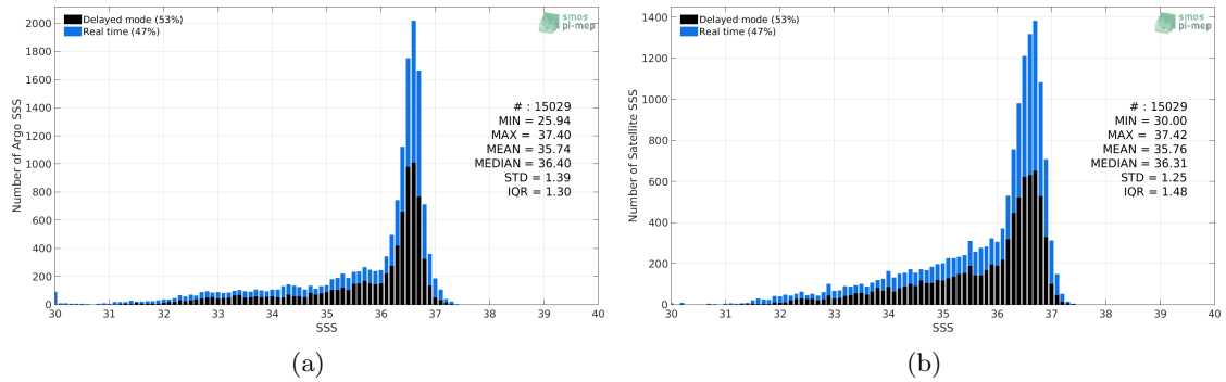
Figure 2: Histograms of SSS from Argo (a) and SMAP-L3-RSS-V4-MONTHLY (b) considering all match-up pairs per bins of 0.1 over the Gulf Stream Pi-MEP region and for the full satellite product period.
