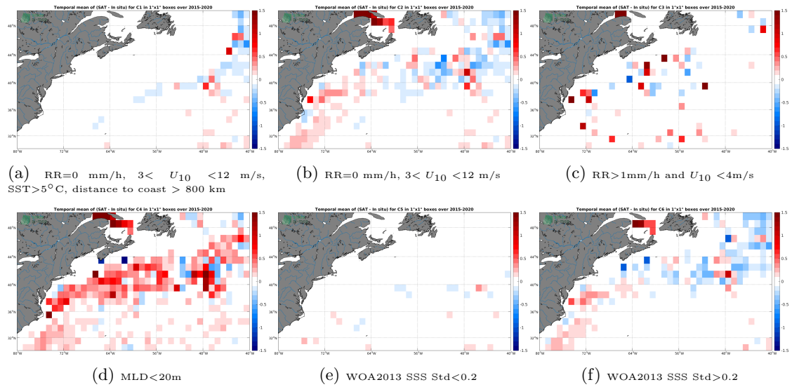
Figure 12: Temporal mean gridded over spatial boxes of size 1^\circ \times 1^\circ of \Delta SSS (SMAP-L3-RSS-V4-MONTHLY - Argo) for 6 different subdatasets corresponding to:RR=0 mm/h, 3 < U_{10} < 12 m/s, SST > 5^\circ\text{C} , distance to coast > 800 km (a), RR=0 mm/h, 3 < U_{10} < 12 m/s (b), RR > 1 mm/h and U_{10} < 4 m/s (c),MLD < 20 m (d),WOA2013 SSS Std < 0.2 (e),WOA2013 SSS Std > 0.2 (f).
