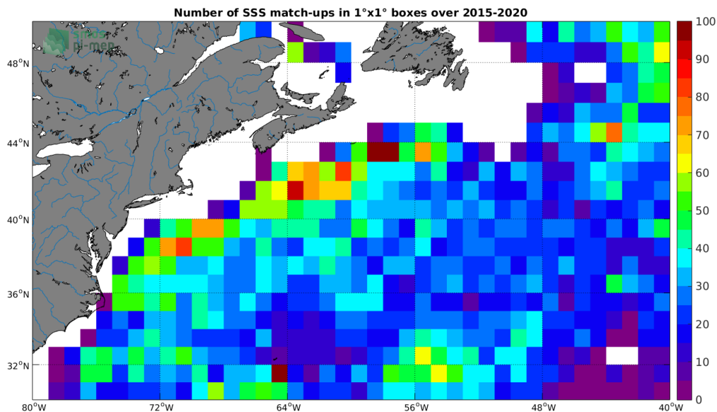
Figure 4: Number of SSS match-ups between Argo SSS and the SMAP-L3-RSS-V4-MONTHLY SSS product for the Gulf Stream Pi-MEP region over 1^\circ \times 1^\circ boxes and for the full satellite product period.
