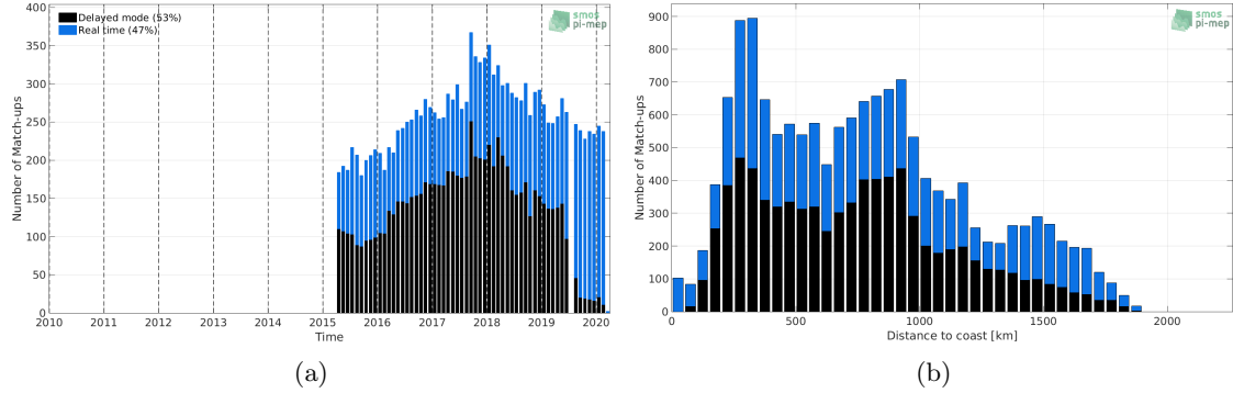
Figure 1: Number of match-ups between Argo and SMAP-L3-RSS-V4-MONTHLY SSS as a function of time (a) and as function of the distance to coast (b) over the Gulf Stream Pi-MEP region and for the full satellite product period.
