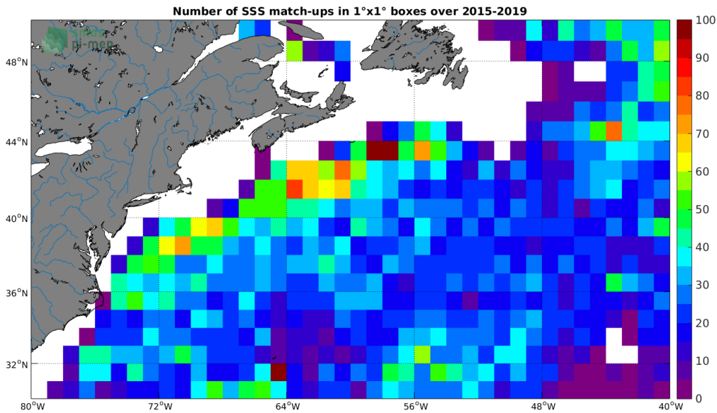
Figure 4: Number of SSS match-ups between Argo SSS and the SMAP-L3-RSS-V4-MONTHLY SSS product for the Gulf Stream Pi-MEP region over 1°x1° boxes and for the full satellite product period.
