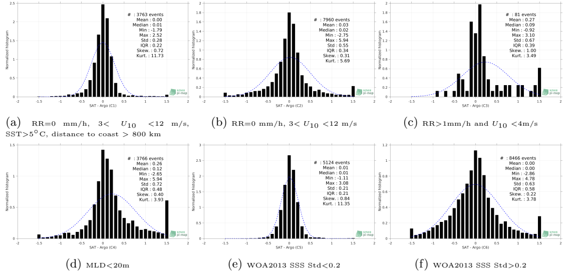
Figure 13: Normalized histogram of \Delta\text{SSS} (SMAP-L3-RSS-V4-MONTHLY - Argo) for 6 different subdatasets corresponding to: RR=0 mm/h, 3 < U_{10} < 12 m/s, SST>5°C, distance to coast > 800 km (a), RR=0 mm/h, 3 < U_{10} < 12 m/s (b), RR>1mm/h and U_{10} < 4 m/s (c), MLD<20m (d), WOA2013 SSS Std<0.2 (e), WOA2013 SSS Std>0.2 (f).
