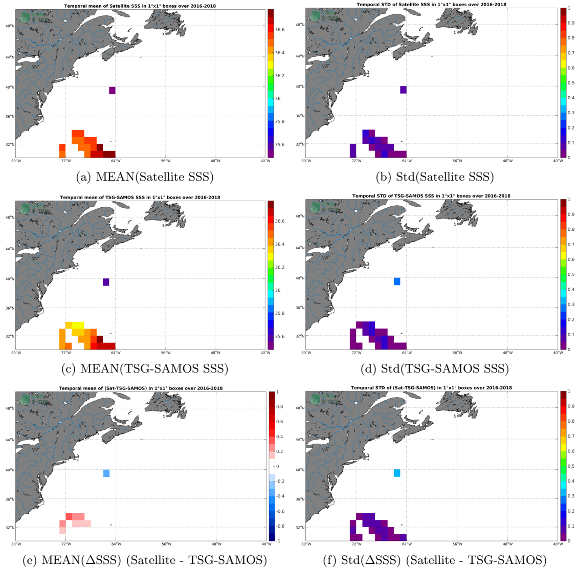
Figure 6: Temporal mean (left) and Std (right) of SSS from SMAP-L3-RSS-V3-8DAY-RUNNING-70KM (top), TSG-SAMOS (middle), and of \Delta SSS (Satellite - TSG-SAMOS). Only match-up pairs are used to generate these maps.
