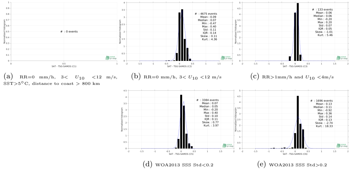
Figure 13: Normalized histogram of \Delta SSS (SMAP-L3-RSS-V3-8DAY-RUNNING-70KM - TSG-SAMOS) for 5 different subdatasets corresponding to: RR=0 mm/h, 3 < U_{10} < 12 m/s, SST > 5°C, distance to coast > 800 km (a), RR=0 mm/h, 3 < U_{10} < 12 m/s (b), RR > 1mm/h and U_{10} < 4 m/s (c), WOA2013 SSS Std < 0.2 (d), WOA2013 SSS Std > 0.2 (e).
