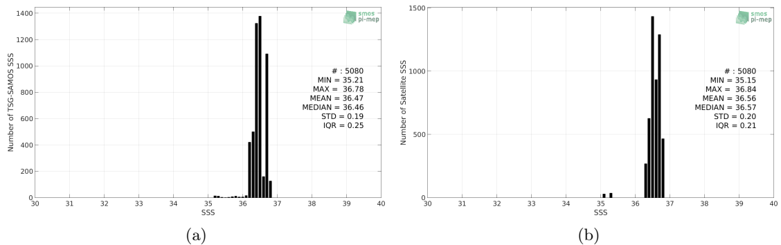
Figure 2: Histograms of SSS from TSG-SAMOS (a) and SMAP-L3-RSS-V3-8DAY-RUNNING-70KM (b) considering all match-up pairs per bins of 0.1 over the Gulf Stream Pi-MEP region and for the full satellite product period.
