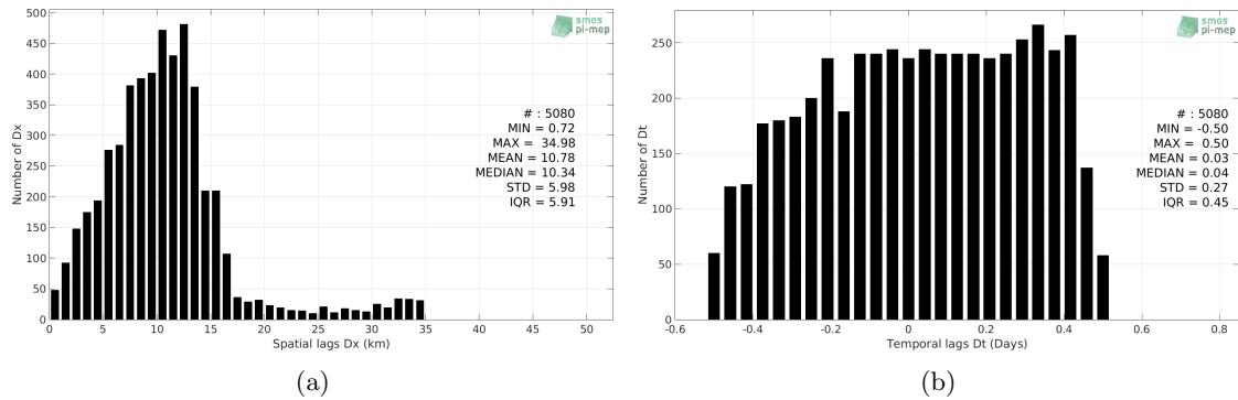
Figure 5: Histograms of the spatial (a) and temporal (b) lags between the time of the TSG-SAMOS measurements and the date of the corresponding SMAP-L3-RSS-V3-8DAY-RUNNING-70KM SSS product.
