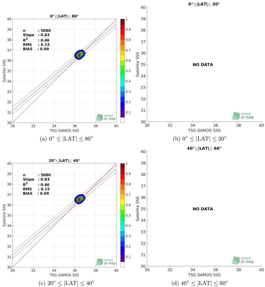
Figure 9: Contour maps of the concentration of SMAP-L3-RSS-V3-8DAY-RUNNING-70KM SSS (y-axis) versus TSG-SAMOS SSS (x-axis) at match-up pairs for different latitude bands. For each plot, the red line shows x=y . The black thin and dashed lines indicate a linear fit through the data cloud and the \pm 95\% confidence levels, respectively. The number match-up pairs n , the slope and R^2 coefficient of the linear fit, the root mean square (RMS) and the mean bias between satellite and in situ data are indicated for each latitude band in each plots.
