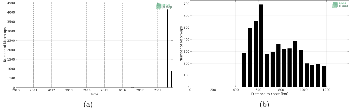
Figure 1: Number of match-ups between TSG-SAMOS and SMAP-L3-RSS-V3-8DAY-RUNNING-70KM SSS as a function of time (a) and as function of the distance to coast (b) over the Gulf Stream Pi-MEP region and for the full satellite product period.
