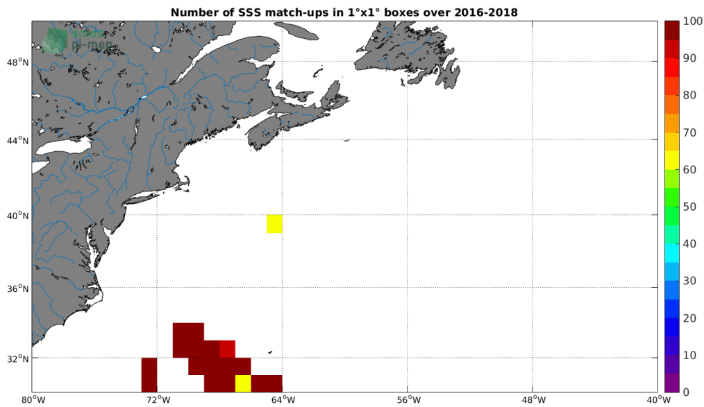
Figure 4: Number of SSS match-ups between TSG-SAMOS SSS and the SMAP-L3-RSS-V3-8DAY-RUNNING-70KM SSS product for the Gulf Stream Pi-MEP region over 1^\circ \times 1^\circ boxes and for the full satellite product period.
