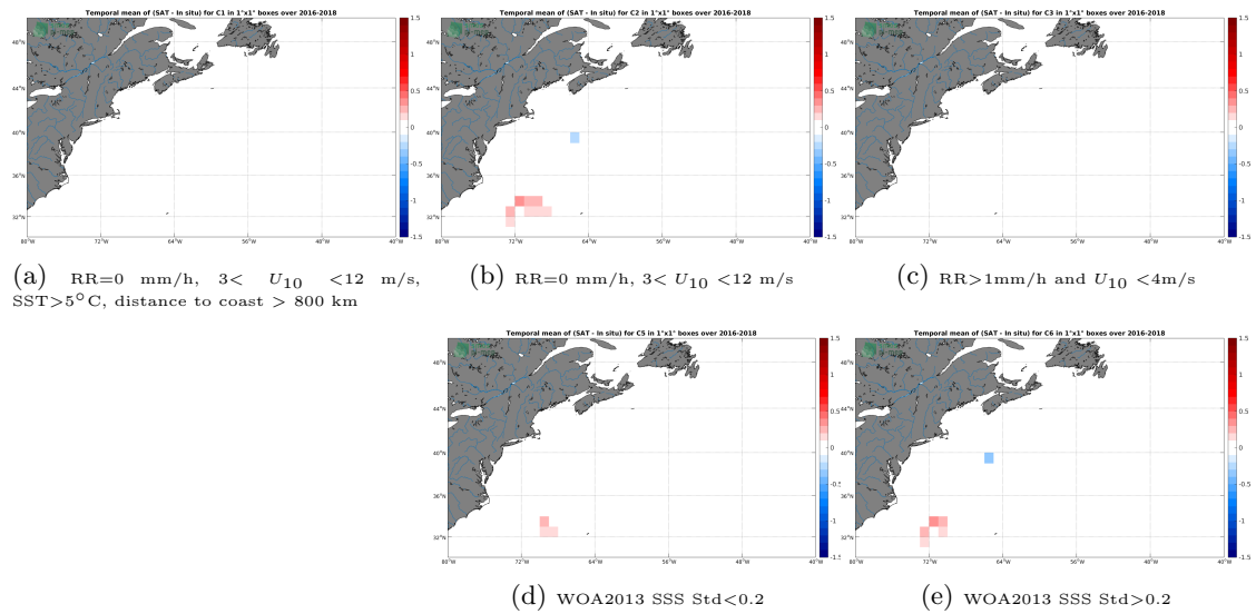
Figure 12: Temporal mean gridded over spatial boxes of size 1^\circ \times 1^\circ of \Delta SSS (SMAP-L3-RSS-V3-8DAY-RUNNING-70KM - TSG-SAMOS) for 5 different subdatasets corresponding to:RR=0 mm/h, 3 < U_{10} < 12 m/s, SST >5^\circ C, distance to coast > 800 km (a), RR=0 mm/h, 3 < U_{10} < 12 m/s (b), RR >1 mm/h and U_{10} < 4 m/s (c), WOA2013 SSS Std <0.2 (d), WOA2013 SSS Std >0.2 (e).
