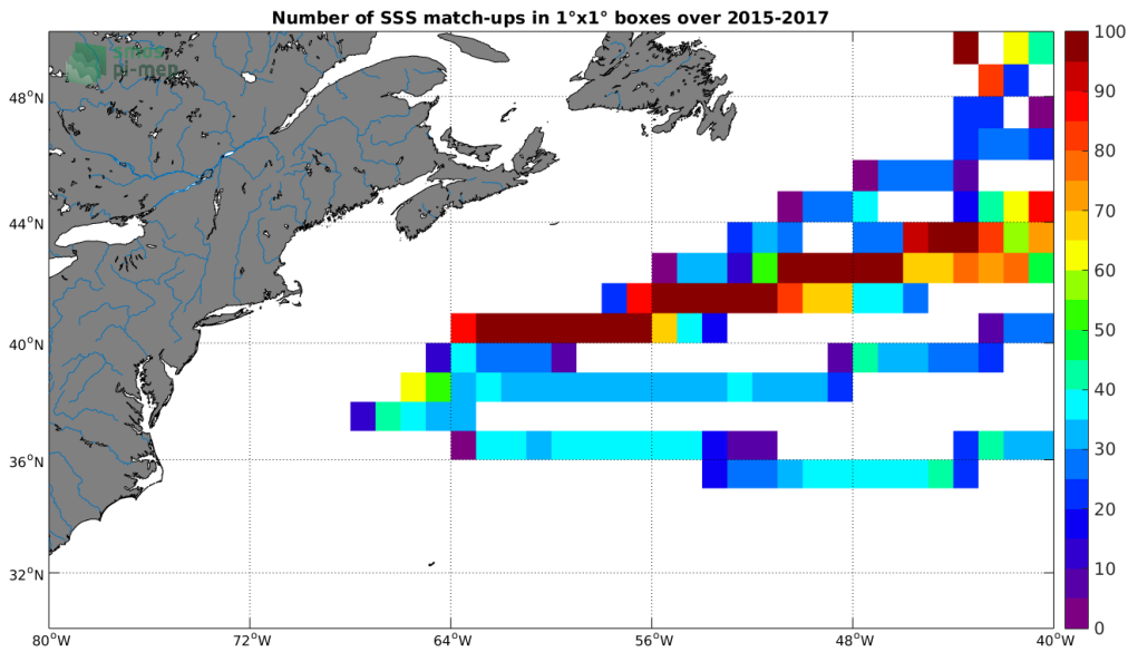
Figure 4: Number of SSS match-ups between TSG-LEGOS-DM SSS and the SMAP-L3-RSS-V3-8DAY-RUNNING-70KM SSS product for the Gulf Stream Pi-MEP region over 1^\circ \times 1^\circ boxes and for the full satellite product period.
