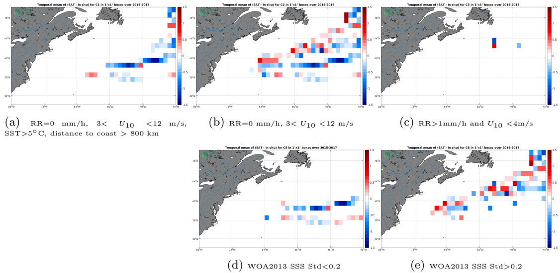
Figure 12: Temporal mean gridded over spatial boxes of size 1^\circ \times 1^\circ of \Delta SSS (SMAP-L3-RSS-V3-8DAY-RUNNING-70KM - TSG-LEGOS-DM) for 5 different subdatasets corresponding to:RR=0 mm/h, 3 < U_{10} < 12 m/s, SST >5^\circ C, distance to coast > 800 km (a), RR=0 mm/h, 3 < U_{10} < 12 m/s (b), RR >1 mm/h and U_{10} < 4 m/s (c), WOA2013 SSS Std <0.2 (d), WOA2013 SSS Std >0.2 (e).
