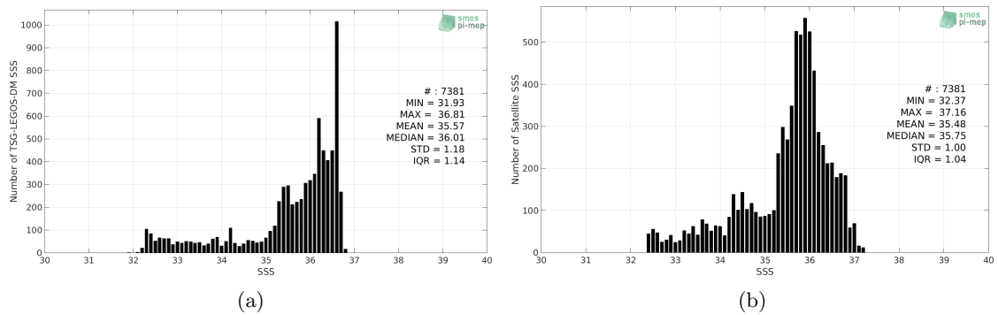
Figure 2: Histograms of SSS from TSG-LEGOS-DM (a) and SMAP-L3-RSS-V3-8DAY-RUNNING-70KM (b) considering all match-up pairs per bins of 0.1 over the Gulf Stream Pi-MEP region and for the full satellite product period.
