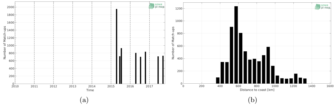
Figure 1: Number of match-ups between TSG-LEGOS-DM and SMAP-L3-RSS-V3-8DAY-RUNNING-70KM SSS as a function of time (a) and as function of the distance to coast (b) over the Gulf Stream Pi-MEP region and for the full satellite product period.
