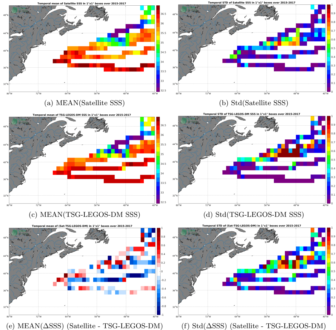
Figure 6: Temporal mean (left) and Std (right) of SSS from SMAP-L3-RSS-V3-8DAY-RUNNING-70KM (top), TSG-LEGOS-DM (middle), and of \Delta SSS (Satellite - TSG-LEGOS-DM). Only match-up pairs are used to generate these maps.
