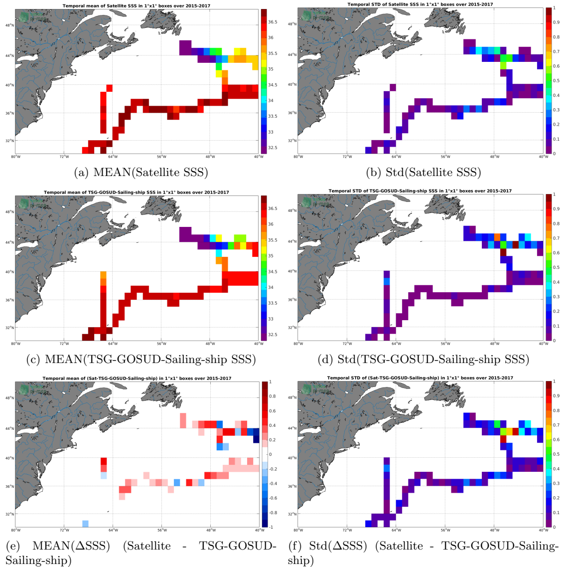
Figure 6: Temporal mean (left) and Std (right) of SSS from SMAP-L3-RSS-V3-8DAY-RUNNING-70KM (top), TSG-GOSUD-Sailing-ship (middle), and of \Delta SSS (Satellite - TSG-GOSUD-Sailing-ship). Only match-up pairs are used to generate these maps.
