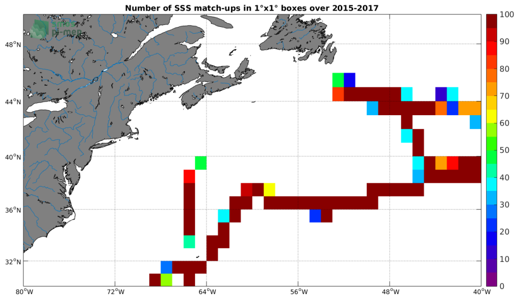
Figure 4: Number of SSS match-ups between TSG-GOSUD-Sailing-ship SSS and the SMAP-L3-RSS-V3-8DAY-RUNNING-70KM SSS product for the Gulf Stream Pi-MEP region over 1^\circ \times 1^\circ boxes and for the full satellite product period.
