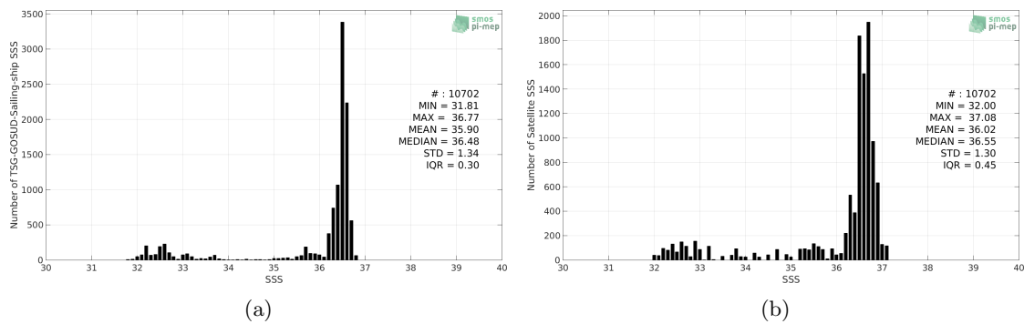
Figure 2: Histograms of SSS from TSG-GOSUD-Sailing-ship (a) and SMAP-L3-RSS-V3-8DAY-RUNNING-70KM (b) considering all match-up pairs per bins of 0.1 over the Gulf Stream Pi-MEP region and for the full satellite product period.
