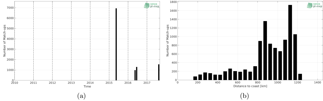
Figure 1: Number of match-ups between TSG-GOSUD-Sailing-ship and SMAP-L3-RSS-V3-8DAY-RUNNING-70KM SSS as a function of time (a) and as function of the distance to coast (b) over the Gulf Stream Pi-MEP region and for the full satellite product period.
