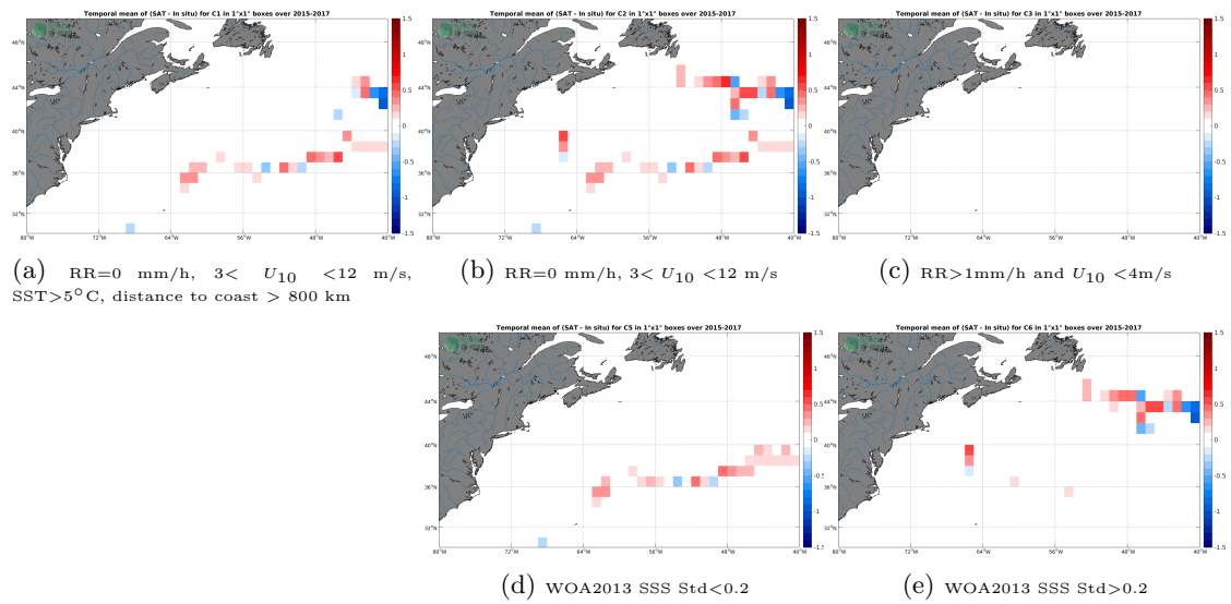
Figure 12: Temporal mean gridded over spatial boxes of size 1^\circ \times 1^\circ of \Delta SSS (SMAP-L3-RSS-V3-8DAY-RUNNING-70KM - TSG-GOSUD-Sailing-ship) for 5 different subdatasets corresponding to:RR=0 mm/h, 3 < U_{10} < 12 m/s, SST >5^\circ C, distance to coast > 800 km (a), RR=0 mm/h, 3 < U_{10} < 12 m/s (b), RR >1 mm/h and U_{10} < 4 m/s (c), WOA2013 SSS Std <0.2 (d), WOA2013 SSS Std >0.2 (e).
