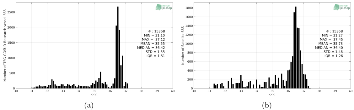
Figure 2: Histograms of SSS from TSG-GOSUD-Research-vessel (a) and SMAP-L3-RSS-V3-8DAY-RUNNING-70KM (b) considering all match-up pairs per bins of 0.1 over the Gulf Stream Pi-MEP region and for the full satellite product period.
