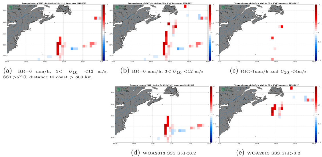
Figure 12: Temporal mean gridded over spatial boxes of size 1^\circ \times 1^\circ of \Delta SSS (SMAP-L3-RSS-V3-8DAY-RUNNING-70KM - TSG-GOSUD-Research-vessel) for 5 different subdatasets corresponding to:RR=0 mm/h, 3 < U_{10} < 12 m/s, SST >5^\circ C, distance to coast > 800 km (a), RR=0 mm/h, 3 < U_{10} < 12 m/s (b), RR >1 mm/h and U_{10} < 4 m/s (c), WOA2013 SSS Std <0.2 (d), WOA2013 SSS Std >0.2 (e).
