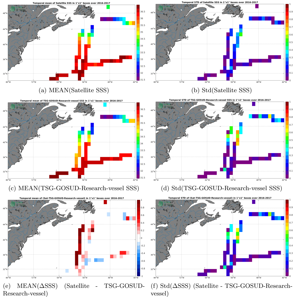
Figure 6: Temporal mean (left) and Std (right) of SSS from SMAP-L3-RSS-V3-8DAY-RUNNING-70KM (top), TSG-GOSUD-Research-vessel (middle), and of \Delta SSS (Satellite - TSG-GOSUD-Research-vessel). Only match-up pairs are used to generate these maps.
