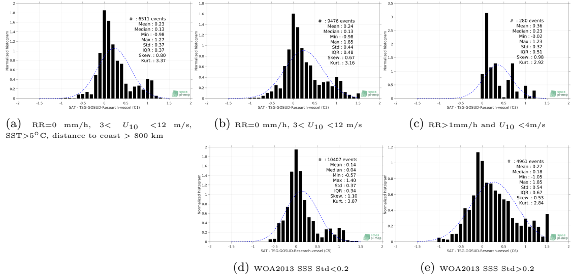
Figure 13: Normalized histogram of \Delta SSS (SMAP-L3-RSS-V3-8DAY-RUNNING-70KM - TSG-GOSUD-Research-vessel) for 5 different subdatasets corresponding to: RR=0 mm/h, 3 < U_{10} < 12 m/s, SST > 5°C, distance to coast > 800 km (a), RR=0 mm/h, 3 < U_{10} < 12 m/s (b), RR > 1mm/h and U_{10} < 4 m/s (c), WOA2013 SSS Std < 0.2 (d), WOA2013 SSS Std > 0.2 (e).
