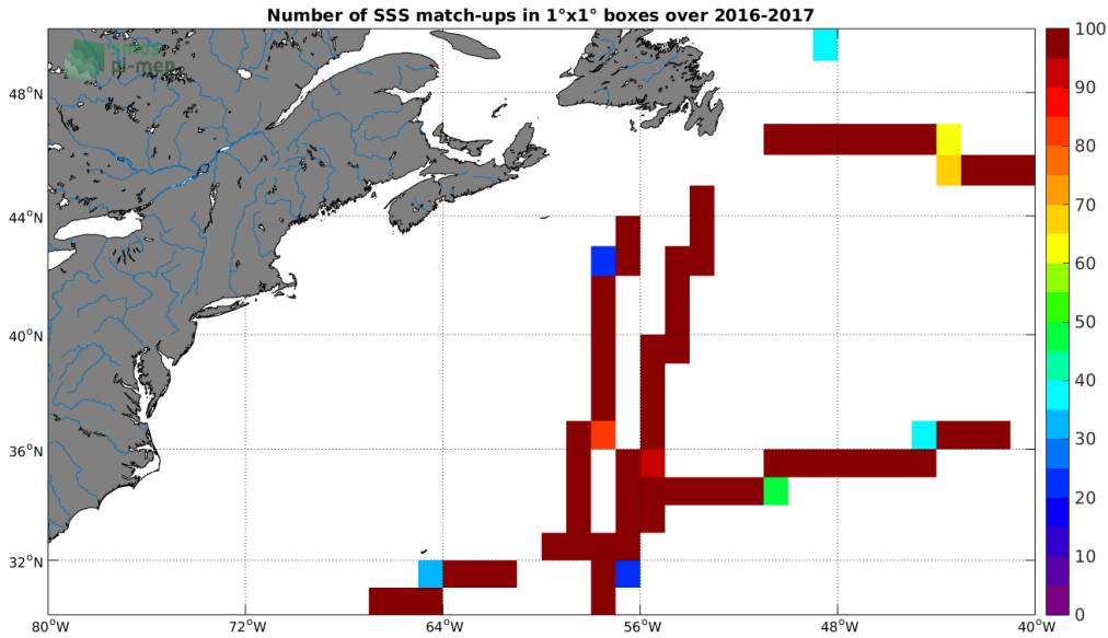
Figure 4: Number of SSS match-ups between TSG-GOSUD-Research-vessel SSS and the SMAP-L3-RSS-V3-8DAY-RUNNING-70KM SSS product for the Gulf Stream Pi-MEP region over 1^\circ \times 1^\circ boxes and for the full satellite product period.
