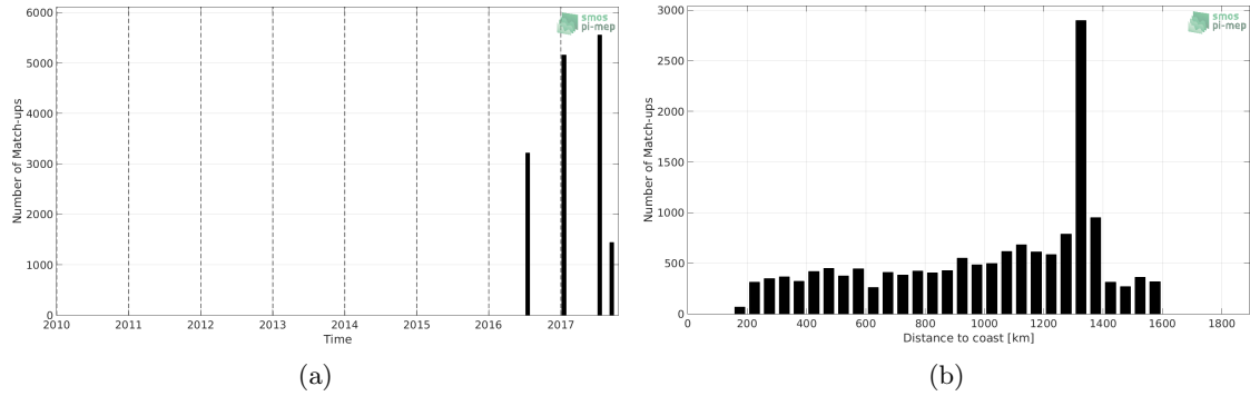
Figure 1: Number of match-ups between TSG-GOSUD-Research-vessel and SMAP-L3-RSS-V3-8DAY-RUNNING-70KM SSS as a function of time (a) and as function of the distance to coast (b) over the Gulf Stream Pi-MEP region and for the full satellite product period.
