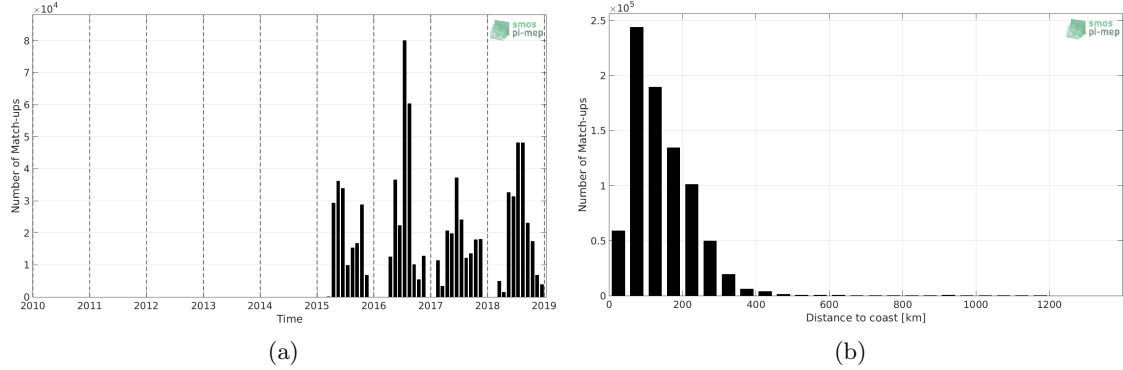
Figure 1: Number of match-ups between TSG-SAMOS and SMAP-L3-RSS-V3-8DAY-RUNNING-40KM SSS as a function of time (a) and as function of the distance to coast (b) over the Gulf Stream Pi-MEP region and for the full satellite product period.
