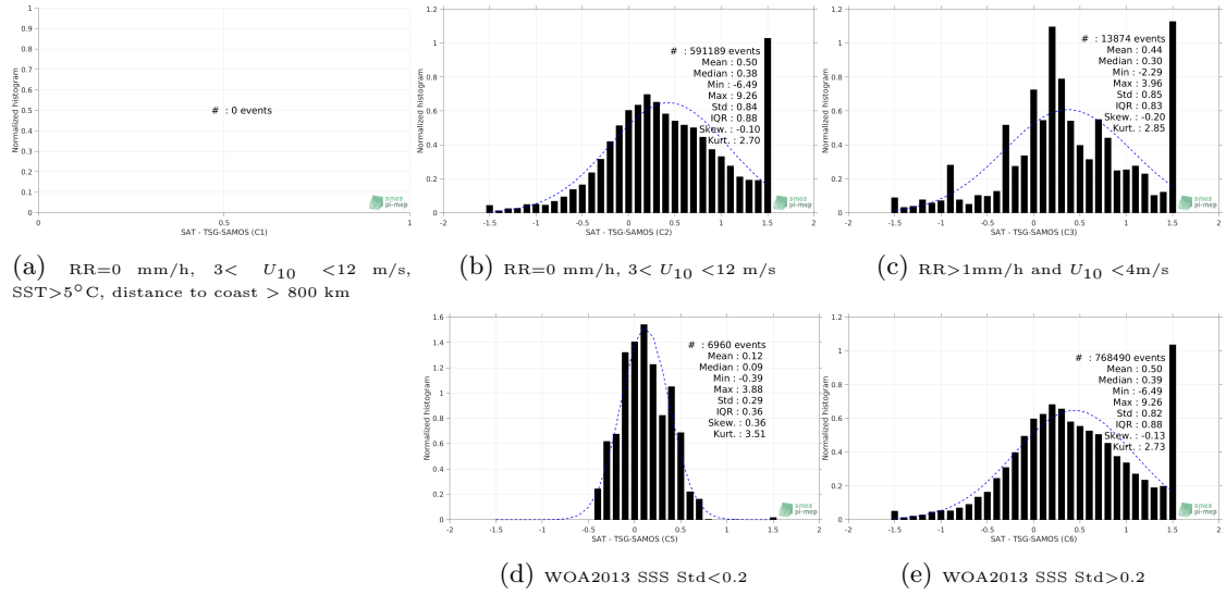
Figure 13: Normalized histogram of \Delta SSS (SMAP-L3-RSS-V3-8DAY-RUNNING-40KM - TSG-SAMOS) for 5 different subdatasets corresponding to: RR=0 mm/h, 3 < U_{10} < 12 m/s, SST > 5°C, distance to coast > 800 km (a), RR=0 mm/h, 3 < U_{10} < 12 m/s (b), RR > 1mm/h and U_{10} < 4 m/s (c), WOA2013 SSS Std < 0.2 (d), WOA2013 SSS Std > 0.2 (e).
