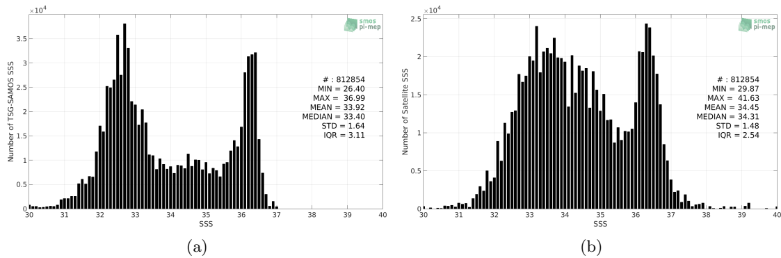
Figure 2: Histograms of SSS from TSG-SAMOS (a) and SMAP-L3-RSS-V3-8DAY-RUNNING-40KM (b) considering all match-up pairs per bins of 0.1 over the Gulf Stream Pi-MEP region and for the full satellite product period.
