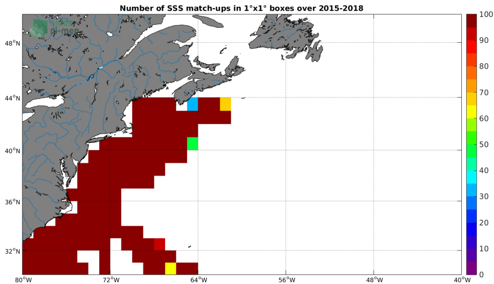
Figure 4: Number of SSS match-ups between TSG-SAMOS SSS and the SMAP-L3-RSS-V3-8DAY-RUNNING-40KM SSS product for the Gulf Stream Pi-MEP region over 1^\circ \times 1^\circ boxes and for the full satellite product period.
