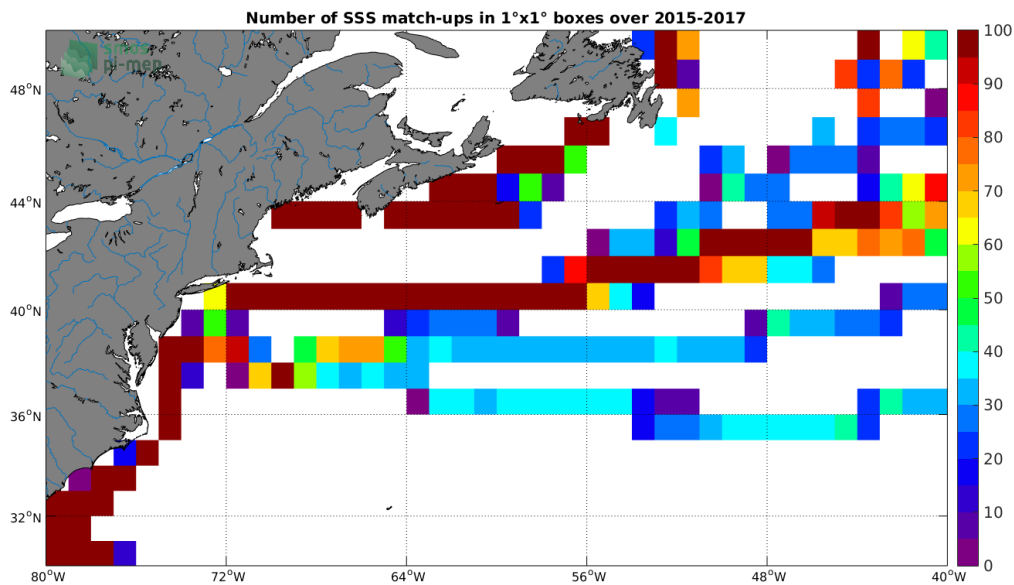
Figure 4: Number of SSS match-ups between TSG-LEGOS-DM SSS and the SMAP-L3-RSS-V3-8DAY-RUNNING-40KM SSS product for the Gulf Stream Pi-MEP region over 1^\circ \times 1^\circ boxes and for the full satellite product period.
