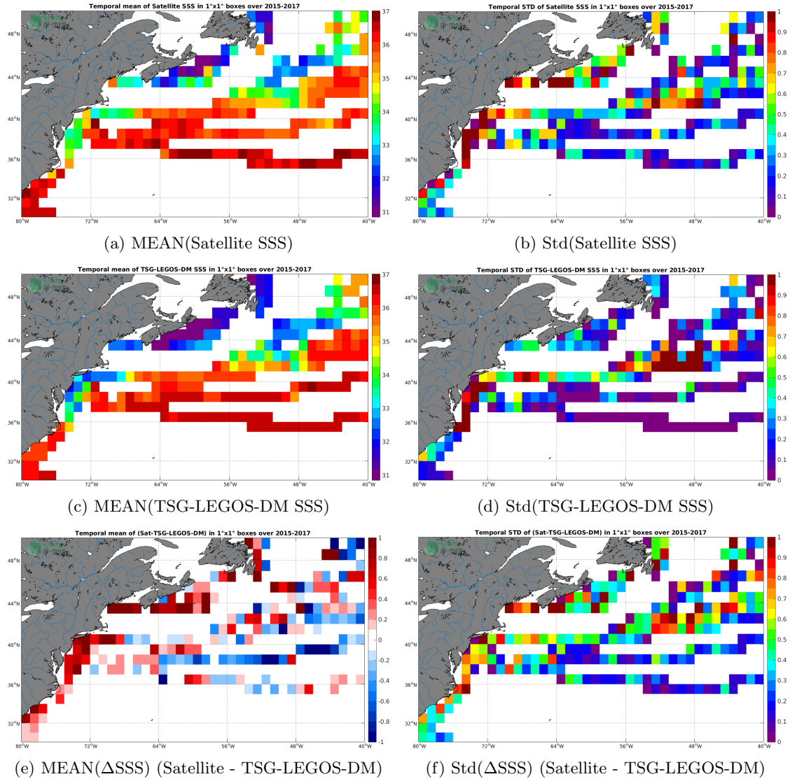
Figure 6: Temporal mean (left) and Std (right) of SSS from SMAP-L3-RSS-V3-8DAY-RUNNING-40KM (top), TSG-LEGOS-DM (middle), and of \Delta SSS (Satellite - TSG-LEGOS-DM). Only match-up pairs are used to generate these maps.
