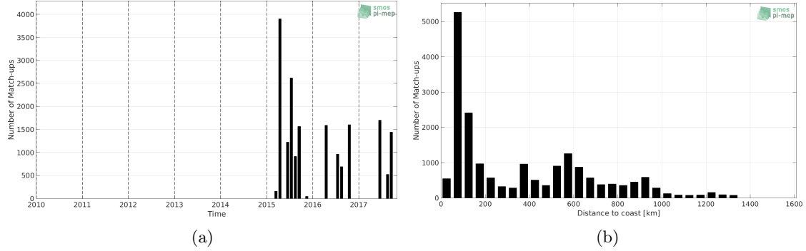
Figure 1: Number of match-ups between TSG-LEGOS-DM and SMAP-L3-RSS-V3-8DAY-RUNNING-40KM SSS as a function of time (a) and as function of the distance to coast (b) over the Gulf Stream Pi-MEP region and for the full satellite product period.
