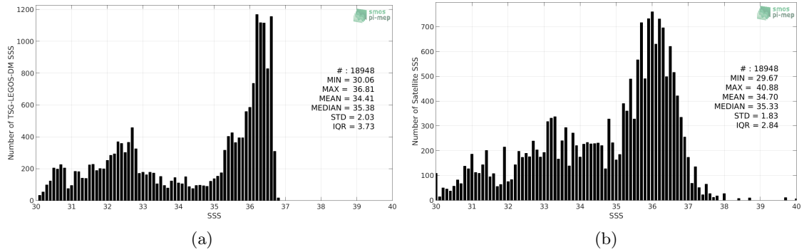
Figure 2: Histograms of SSS from TSG-LEGOS-DM (a) and SMAP-L3-RSS-V3-8DAY-RUNNING-40KM (b) considering all match-up pairs per bins of 0.1 over the Gulf Stream Pi-MEP region and for the full satellite product period.
