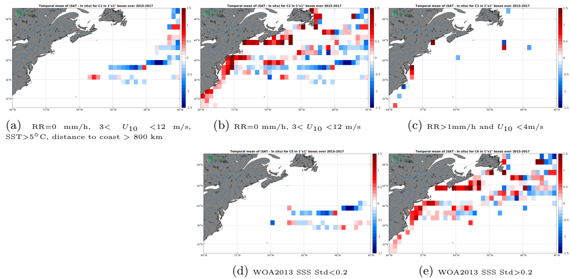
Figure 12: Temporal mean gridded over spatial boxes of size 1^\circ \times 1^\circ of \Delta SSS (SMAP-L3-RSS-V3-8DAY-RUNNING-40KM - TSG-LEGOS-DM) for 5 different subdatasets corresponding to:RR=0 mm/h, 3 < U_{10} < 12 m/s, SST >5^\circ C, distance to coast > 800 km (a), RR=0 mm/h, 3 < U_{10} < 12 m/s (b), RR >1 mm/h and U_{10} < 4 m/s (c), WOA2013 SSS Std <0.2 (d), WOA2013 SSS Std >0.2 (e).
