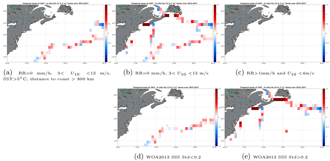
Figure 12: Temporal mean gridded over spatial boxes of size 1^\circ \times 1^\circ of \Delta SSS (SMAP-L3-RSS-V3-8DAY-RUNNING-40KM - TSG-GOSUD-Sailing-ship) for 5 different subdatasets corresponding to: RR=0 mm/h, 3 < U_{10} < 12 m/s, SST > 5^\circ C , distance to coast > 800 km (a), RR=0 mm/h, 3 < U_{10} < 12 m/s (b), RR > 1 mm/h and U_{10} < 4 m/s (c), WOA2013 SSS Std < 0.2 (d), WOA2013 SSS Std > 0.2 (e).
