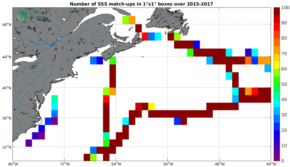
Figure 4: Number of SSS match-ups between TSG-GOSUD-Sailing-ship SSS and the SMAP-L3-RSS-V3-8DAY-RUNNING-40KM SSS product for the Gulf Stream Pi-MEP region over 1^\circ \times 1^\circ boxes and for the full satellite product period.
