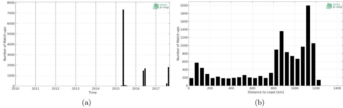
Figure 1: Number of match-ups between TSG-GOSUD-Sailing-ship and SMAP-L3-RSS-V3-8DAY-RUNNING-40KM SSS as a function of time (a) and as function of the distance to coast (b) over the Gulf Stream Pi-MEP region and for the full satellite product period.
