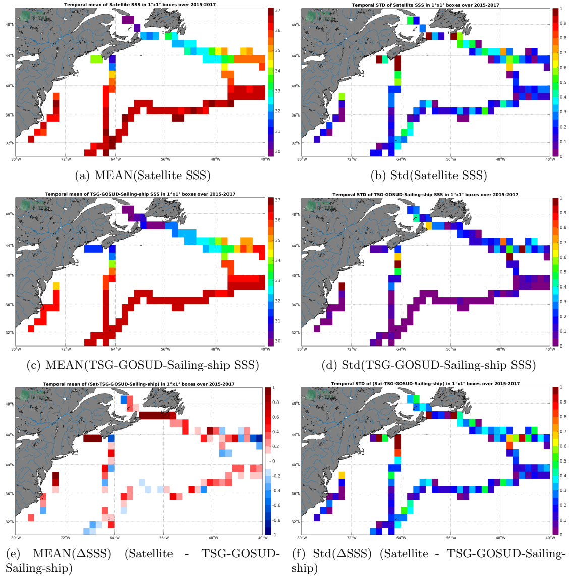
Figure 6: Temporal mean (left) and Std (right) of SSS from SMAP-L3-RSS-V3-8DAY-RUNNING-40KM (top), TSG-GOSUD-Sailing-ship (middle), and of \Delta SSS (Satellite - TSG-GOSUD-Sailing-ship). Only match-up pairs are used to generate these maps.
