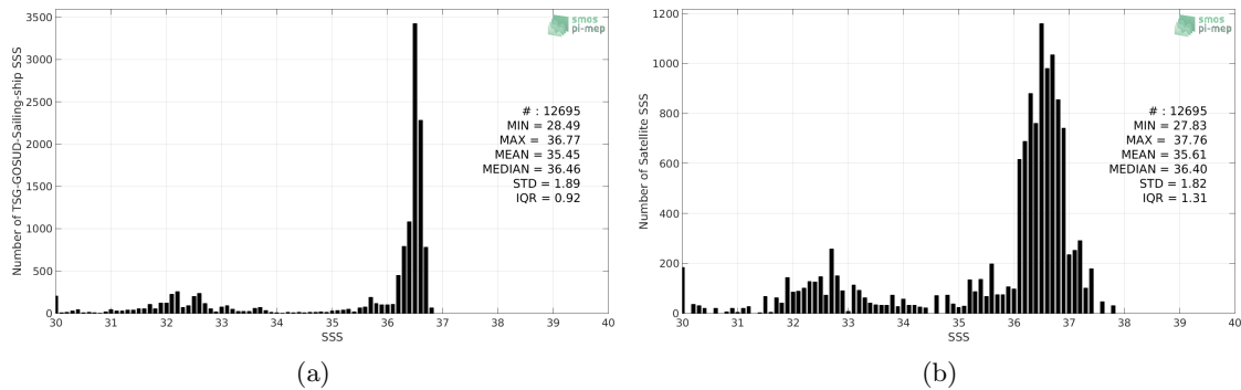
Figure 2: Histograms of SSS from TSG-GOSUD-Sailing-ship (a) and SMAP-L3-RSS-V3-8DAY-RUNNING-40KM (b) considering all match-up pairs per bins of 0.1 over the Gulf Stream Pi-MEP region and for the full satellite product period.
