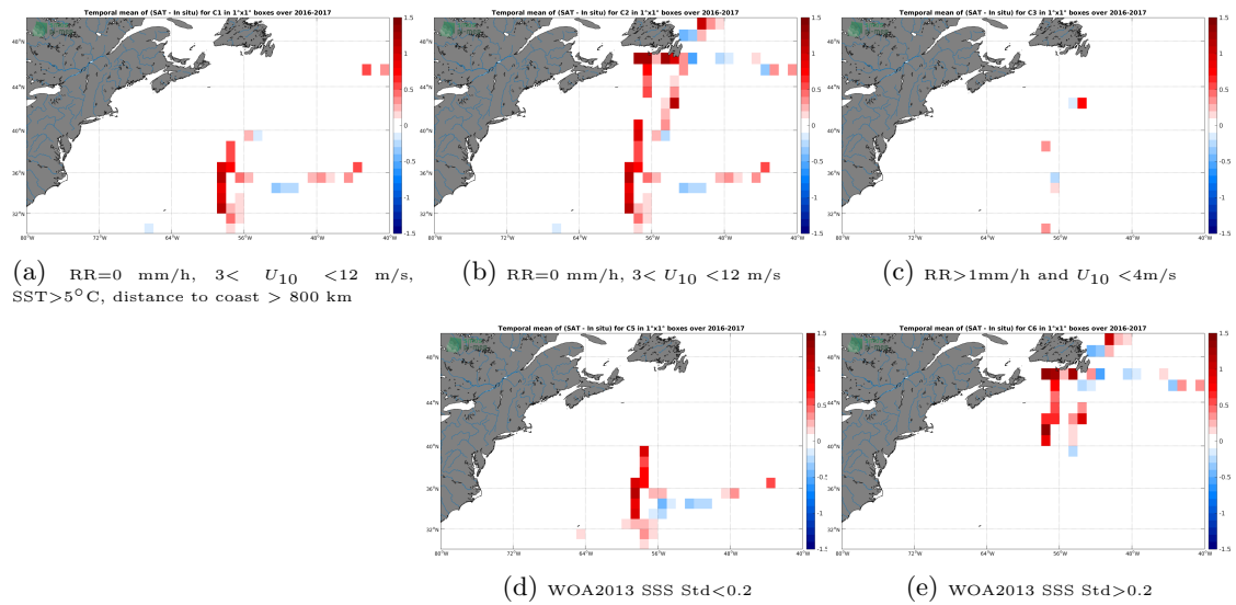
Figure 12: Temporal mean gridded over spatial boxes of size 1^\circ \times 1^\circ of \Delta SSS (SMAP-L3-RSS-V3-8DAY-RUNNING-40KM - TSG-GOSUD-Research-vessel) for 5 different subdatasets corresponding to:RR=0 mm/h, 3 < U_{10} < 12 m/s, SST >5^\circ C, distance to coast > 800 km (a), RR=0 mm/h, 3 < U_{10} < 12 m/s (b), RR >1 mm/h and U_{10} < 4 m/s (c), WOA2013 SSS Std <0.2 (d), WOA2013 SSS Std >0.2 (e).
