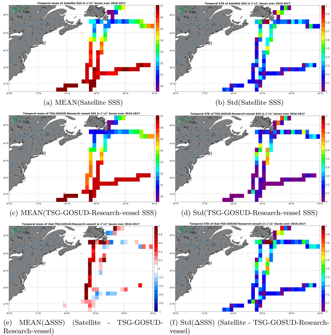
Figure 6: Temporal mean (left) and Std (right) of SSS from SMAP-L3-RSS-V3-8DAY-RUNNING-40KM (top), TSG-GOSUD-Research-vessel (middle), and of \Delta SSS (Satellite - TSG-GOSUD-Research-vessel). Only match-up pairs are used to generate these maps.
