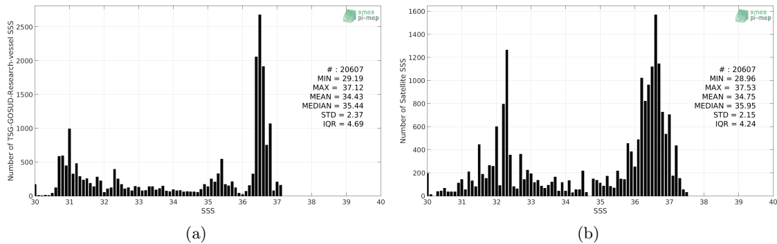
Figure 2: Histograms of SSS from TSG-GOSUD-Research-vessel (a) and SMAP-L3-RSS-V3-8DAY-RUNNING-40KM (b) considering all match-up pairs per bins of 0.1 over the Gulf Stream Pi-MEP region and for the full satellite product period.
