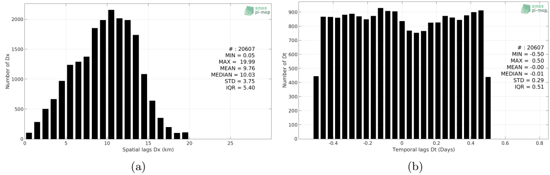
Figure 5: Histograms of the spatial (a) and temporal (b) lags between the time of the TSG-GOSUD-Research-vessel measurements and the date of the corresponding SMAP-L3-RSS-V3-8DAY-RUNNING-40KM SSS product.
