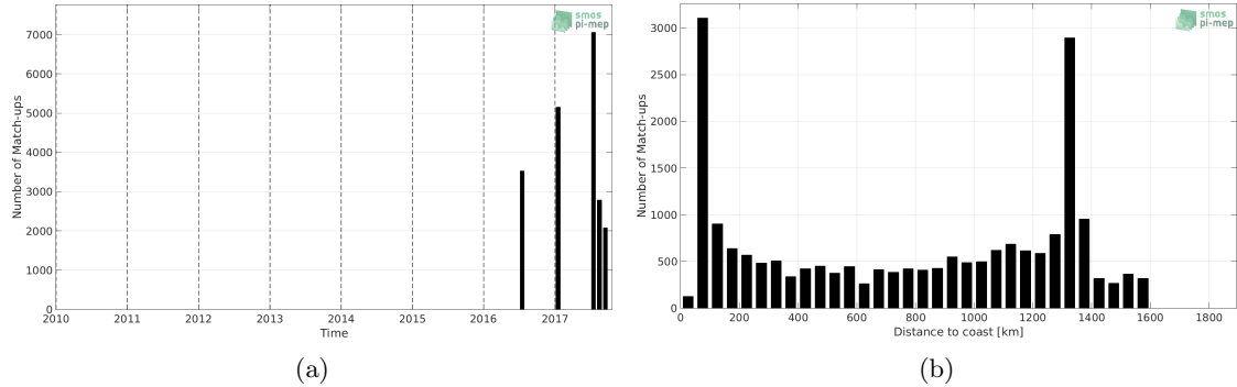
Figure 1: Number of match-ups between TSG-GOSUD-Research-vessel and SMAP-L3-RSS-V3-8DAY-RUNNING-40KM SSS as a function of time (a) and as function of the distance to coast (b) over the Gulf Stream Pi-MEP region and for the full satellite product period.
