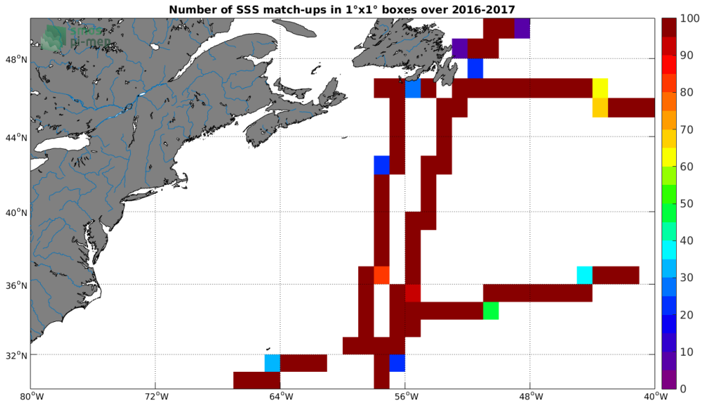
Figure 4: Number of SSS match-ups between TSG-GOSUD-Research-vessel SSS and the SMAP-L3-RSS-V3-8DAY-RUNNING-40KM SSS product for the Gulf Stream Pi-MEP region over 1^\circ \times 1^\circ boxes and for the full satellite product period.
