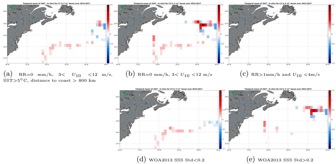
Figure 12: Temporal mean gridded over spatial boxes of size 1^\circ \times 1^\circ of \Delta SSS (SMAP-L3-RSS-V3-MONTHLY-70KM - TSG-GOSUD-Sailing-ship) for 5 different subdatasets corresponding to: RR=0 mm/h, 3 < U_{10} < 12 m/s, SST > 5^\circ C , distance to coast > 800 km (a), RR=0 mm/h, 3 < U_{10} < 12 m/s (b), RR > 1 mm/h and U_{10} < 4 m/s (c), WOA2013 SSS Std < 0.2 (d), WOA2013 SSS Std > 0.2 (e).
