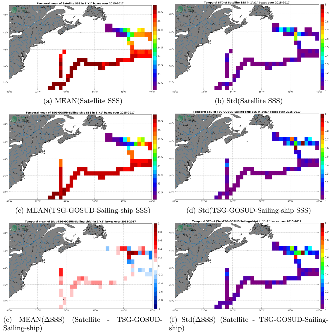
Figure 6: Temporal mean (left) and Std (right) of SSS from SMAP-L3-RSS-V3-MONTHLY-70KM (top), TSG-GOSUD-Sailing-ship (middle), and of \Delta SSS (Satellite - TSG-GOSUD-Sailing-ship). Only match-up pairs are used to generate these maps.
