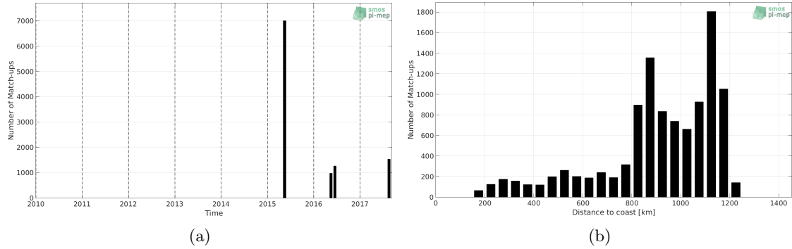
Figure 1: Number of match-ups between TSG-GOSUD-Sailing-ship and SMAP-L3-RSS-V3-MONTHLY-70KM SSS as a function of time (a) and as function of the distance to coast (b) over the Gulf Stream Pi-MEP region and for the full satellite product period.
