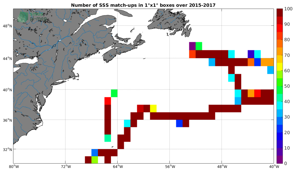
Figure 4: Number of SSS match-ups between TSG-GOSUD-Sailing-ship SSS and the SMAP-L3-RSS-V3-MONTHLY-70KM SSS product for the Gulf Stream Pi-MEP region over 1^\circ \times 1^\circ boxes and for the full satellite product period.
