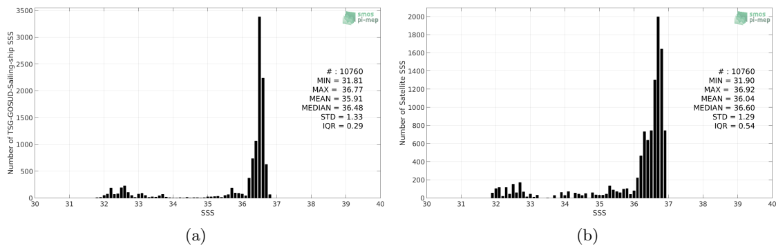
Figure 2: Histograms of SSS from TSG-GOSUD-Sailing-ship (a) and SMAP-L3-RSS-V3-MONTHLY-70KM (b) considering all match-up pairs per bins of 0.1 over the Gulf Stream Pi-MEP region and for the full satellite product period.
