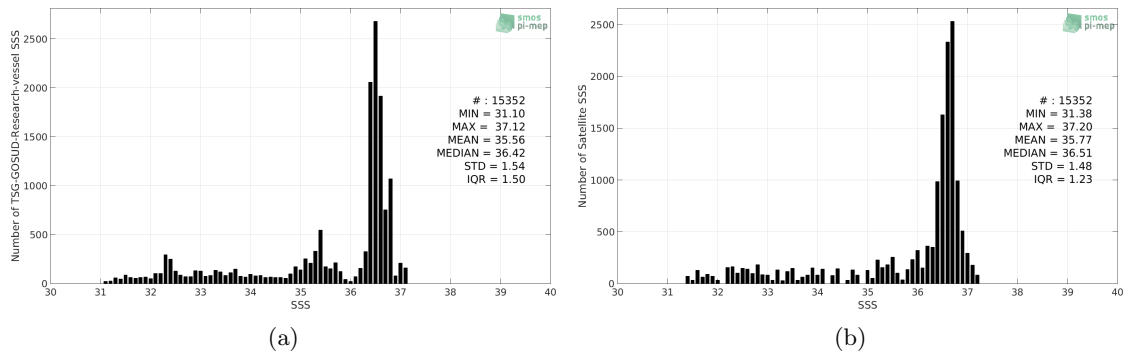
Figure 2: Histograms of SSS from TSG-GOSUD-Research-vessel (a) and SMAP-L3-RSS-V3-MONTHLY-70KM (b) considering all match-up pairs per bins of 0.1 over the Gulf Stream Pi-MEP region and for the full satellite product period.
