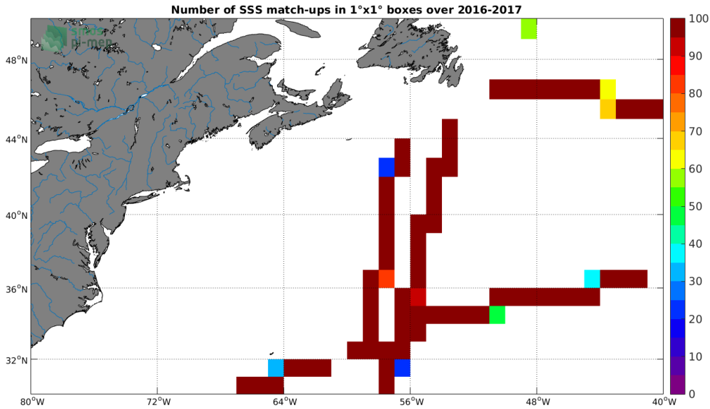
Figure 4: Number of SSS match-ups between TSG-GOSUD-Research-vessel SSS and the SMAP-L3-RSS-V3-MONTHLY-70KM SSS product for the Gulf Stream Pi-MEP region over 1^\circ \times 1^\circ boxes and for the full satellite product period.
