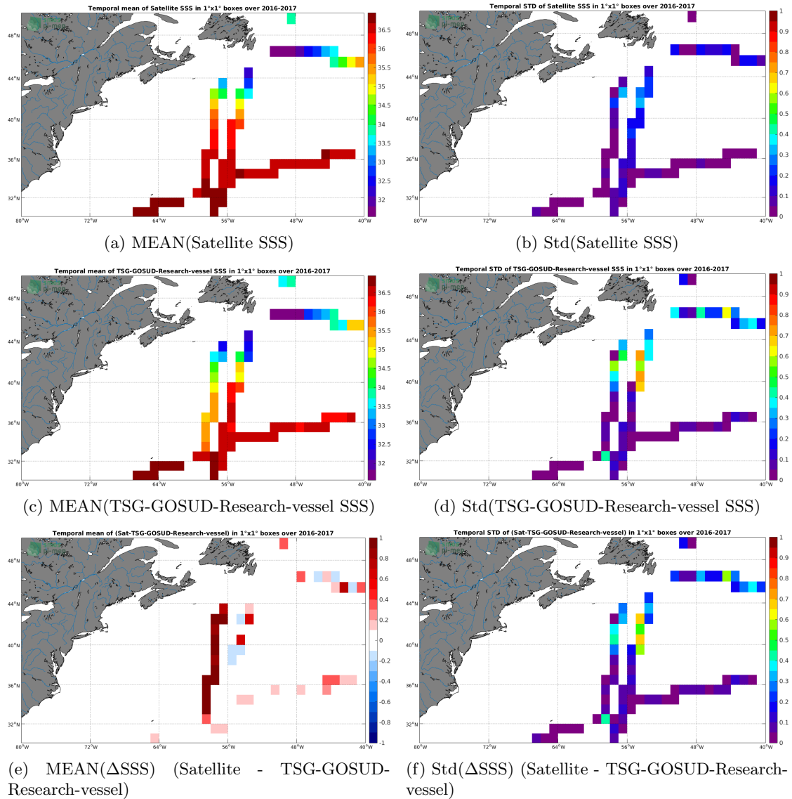
Figure 6: Temporal mean (left) and Std (right) of SSS from SMAP-L3-RSS-V3-MONTHLY-70KM (top), TSG-GOSUD-Research-vessel (middle), and of \Delta SSS (Satellite - TSG-GOSUD-Research-vessel). Only match-up pairs are used to generate these maps.
