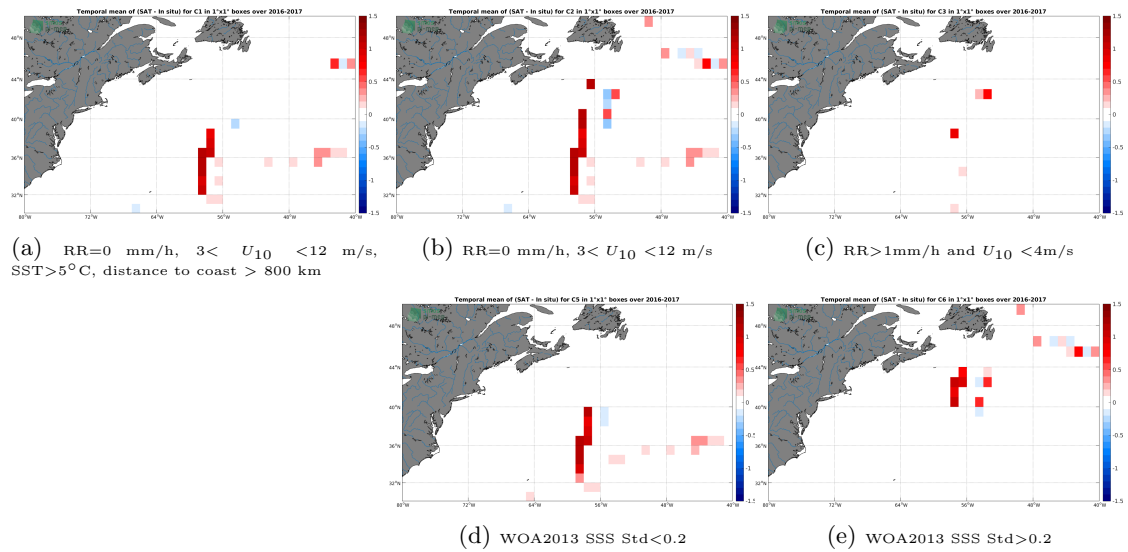
Figure 12: Temporal mean gridded over spatial boxes of size 1^\circ \times 1^\circ of \Delta SSS (SMAP-L3-RSS-V3-MONTHLY-70KM - TSG-GOSUD-Research-vessel) for 5 different subdatasets corresponding to: RR=0 mm/h, 3 < U_{10} < 12 m/s, SST > 5^\circ C , distance to coast > 800 km (a), RR=0 mm/h, 3 < U_{10} < 12 m/s (b), RR > 1 mm/h and U_{10} < 4 m/s (c), WOA2013 SSS Std < 0.2 (d), WOA2013 SSS Std > 0.2 (e).
