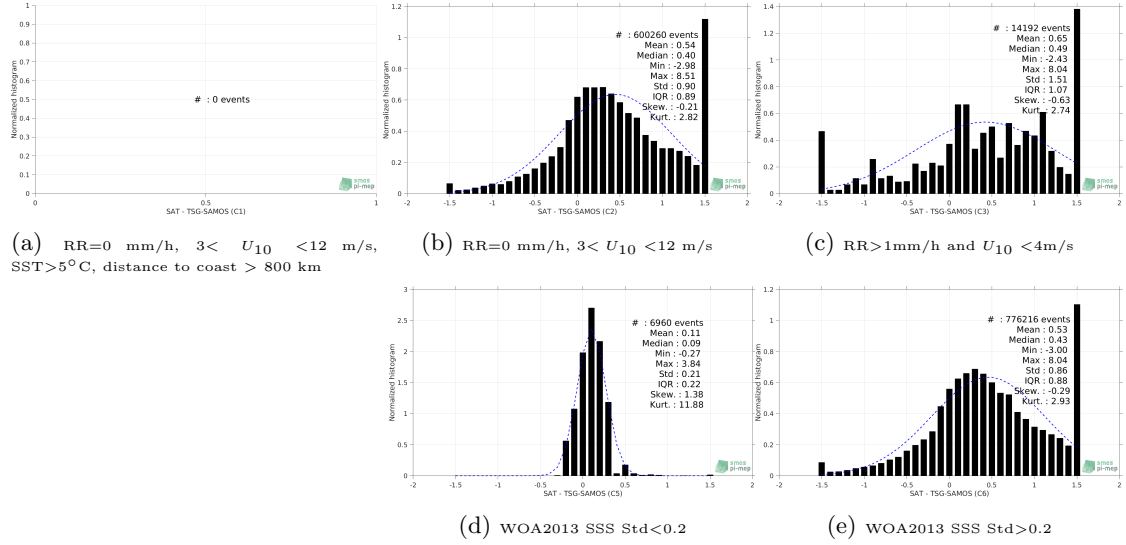
Figure 13: Normalized histogram of \Delta\text{SSS} (SMAP-L3-RSS-V3-MONTHLY-0.25DEG-40KM - TSG-SAMOS) for 5 different subdatasets corresponding to: RR=0 mm/h, 3 < U_{10} < 12 m/s, SST > 5^\circ\text{C} , distance to coast > 800 km (a), RR=0 mm/h, 3 < U_{10} < 12 m/s (b), RR > 1\text{mm/h} and U_{10} < 4\text{m/s} (c), WOA2013 SSS Std <0.2 (d), WOA2013 SSS Std >0.2 (e).
