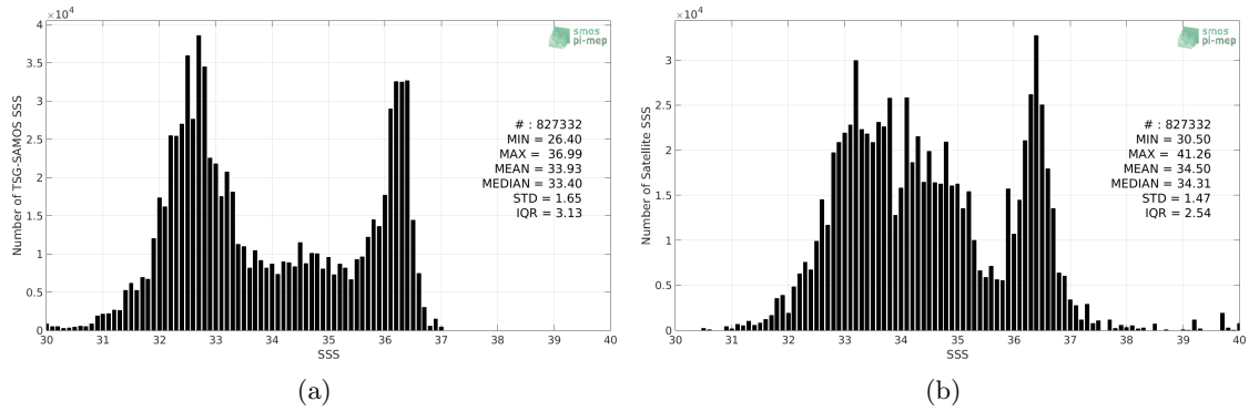
Figure 2: Histograms of SSS from TSG-SAMOS (a) and SMAP-L3-RSS-V3-MONTHLY-0.25DEG-40KM (b) considering all match-up pairs per bins of 0.1 over the Gulf Stream Pi-MEP region and for the full satellite product period.
