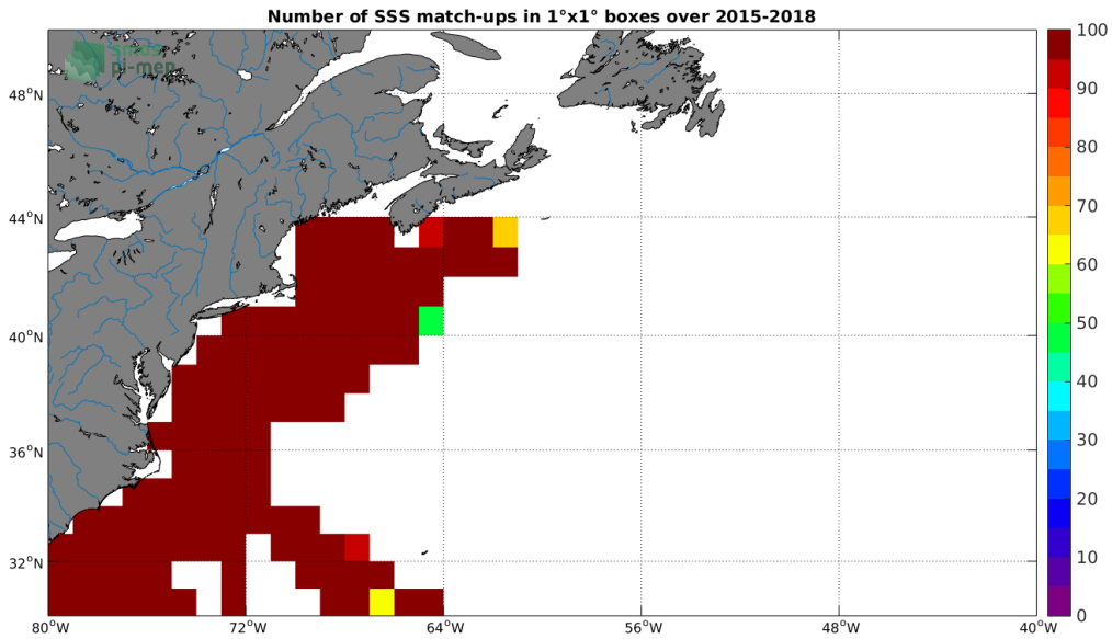
Figure 4: Number of SSS match-ups between TSG-SAMOS SSS and the SMAP-L3-RSS-V3-MONTHLY-0.25DEG-40KM SSS product for the Gulf Stream Pi-MEP region over 1^\circ \times 1^\circ boxes and for the full satellite product period.
