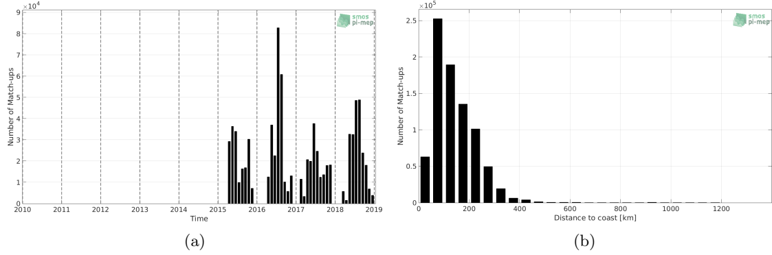
Figure 1: Number of match-ups between TSG-SAMOS and SMAP-L3-RSS-V3-MONTHLY-0.25DEG-40KM SSS as a function of time (a) and as function of the distance to coast (b) over the Gulf Stream Pi-MEP region and for the full satellite product period.
